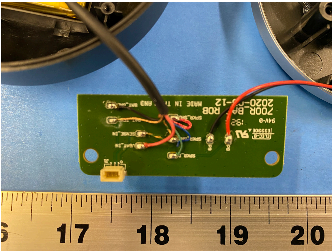
Figure 4: Internal Photo of Stealth700X-MAX-RX (Right Ear PCB, Top)
