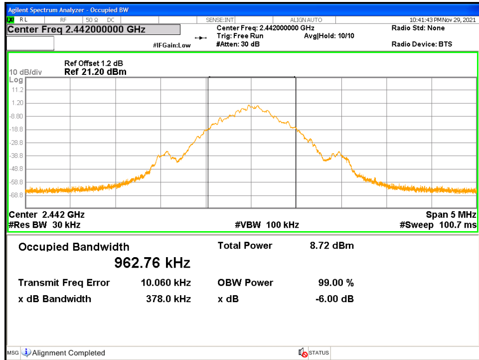
Figure 9: 99% Bandwidth - 2442 MHz
