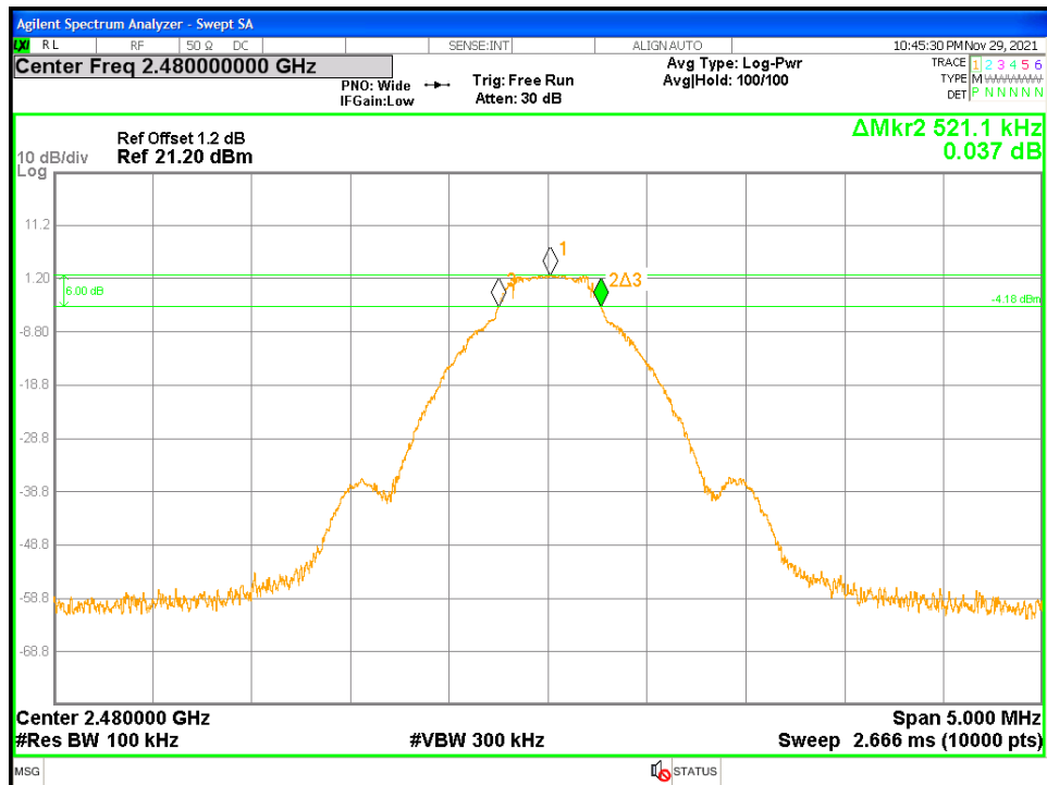
Figure 7: DTS Bandwidth - 2480 MHz
