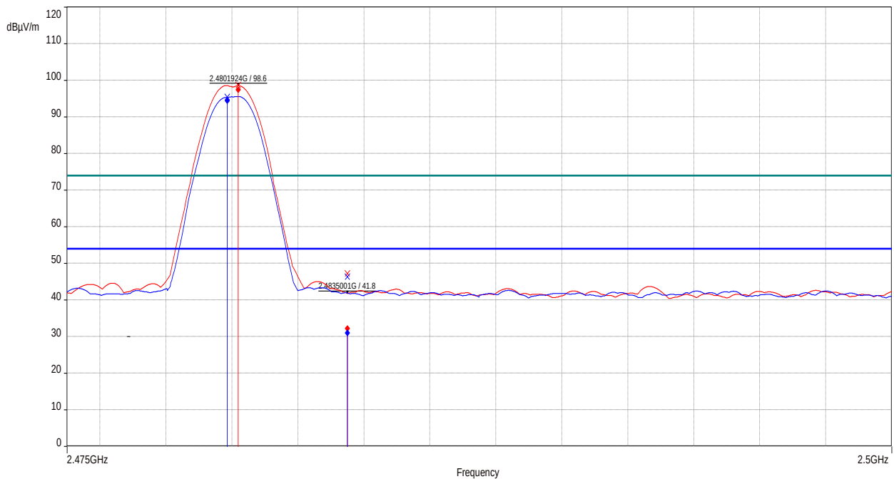
Figure 21: Band-edge-2480 MHz
