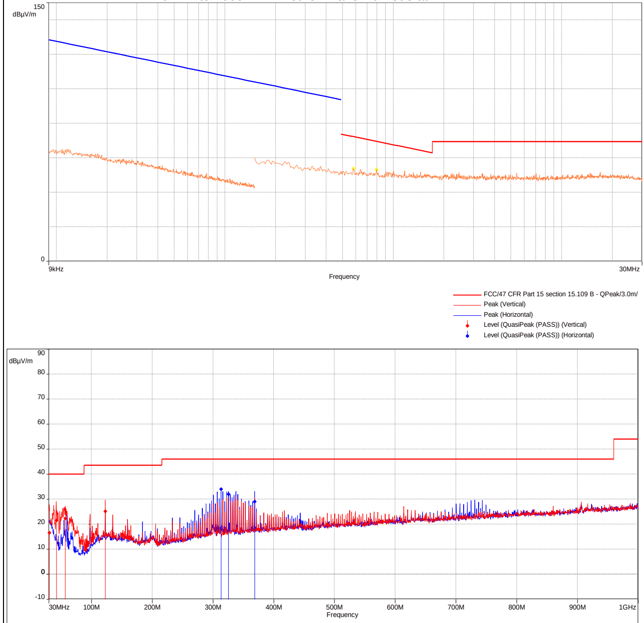
9 kHz to 1000 MHz Plot for Transmit Mode at 2442 MHz
