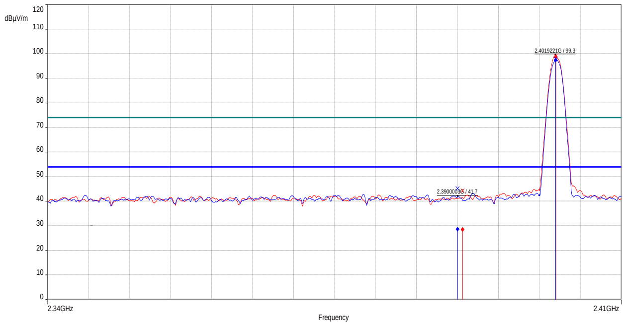
Figure 20: Band-edge-2402 MHz
