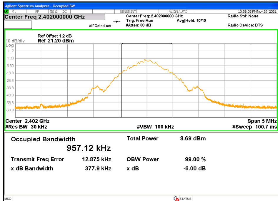
Figure 8: 99% Bandwidth - 2402 MHz
