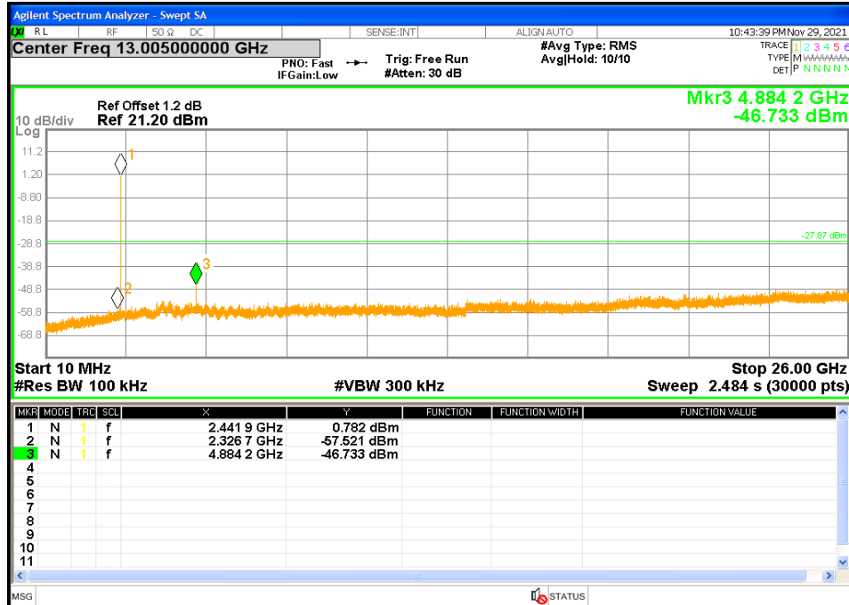
Figure 17: Out of band Emissions at 2442 MHz
