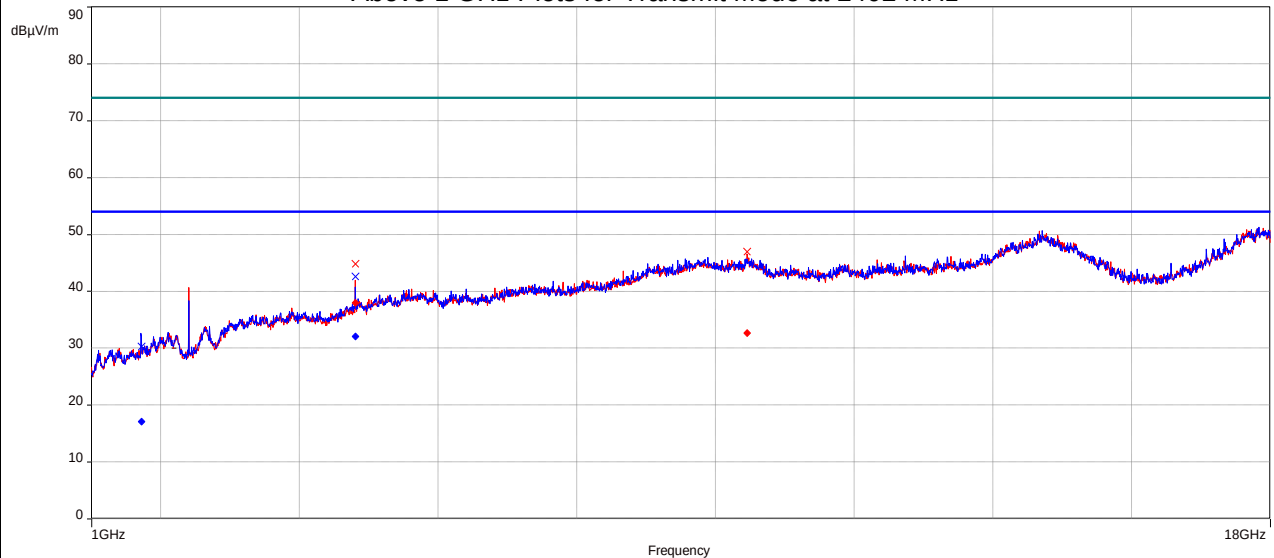
Above 1 GHz Plots for Transmit Mode at 2402 MHz
