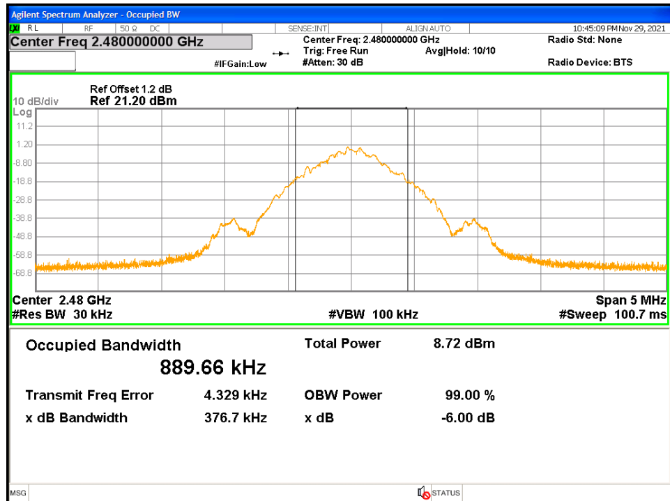
Figure 10: 99% Bandwidth - 2480 MHz
