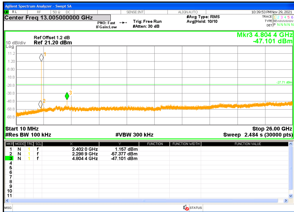
Figure 15: Out of band Emissions at 2402 MHz
