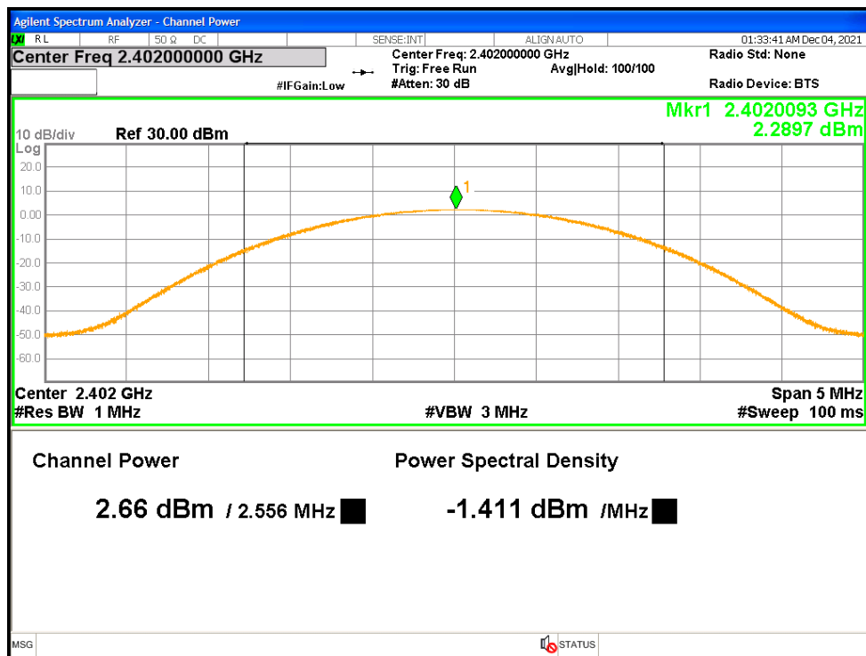
Figure 2: Maximum Transmitted Power, 2402 MHz
