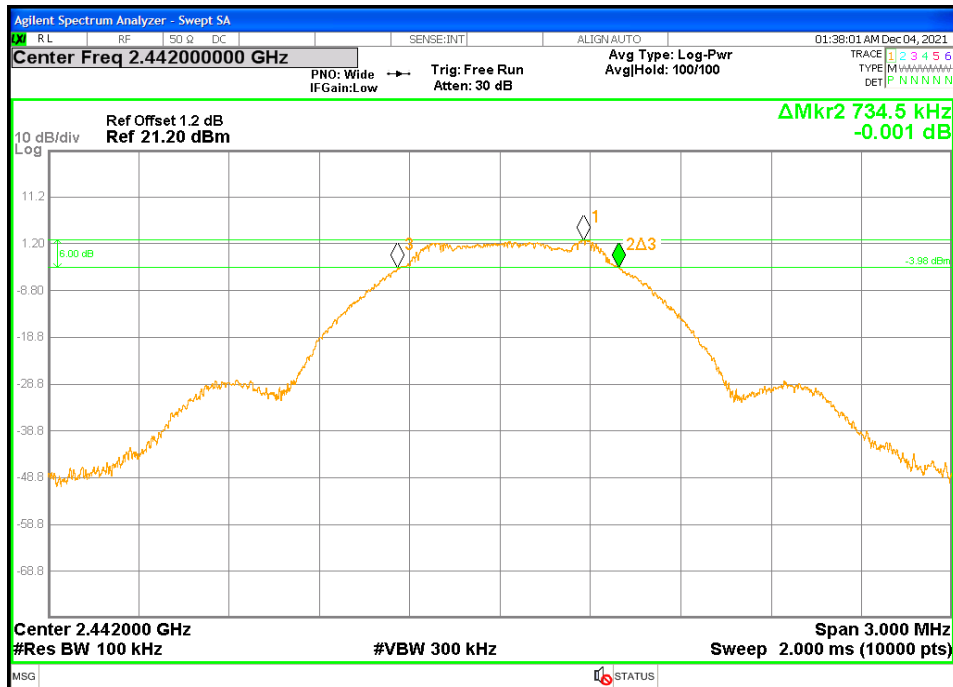
Figure 6: DTS Bandwidth-Headset - 2442 MHz
