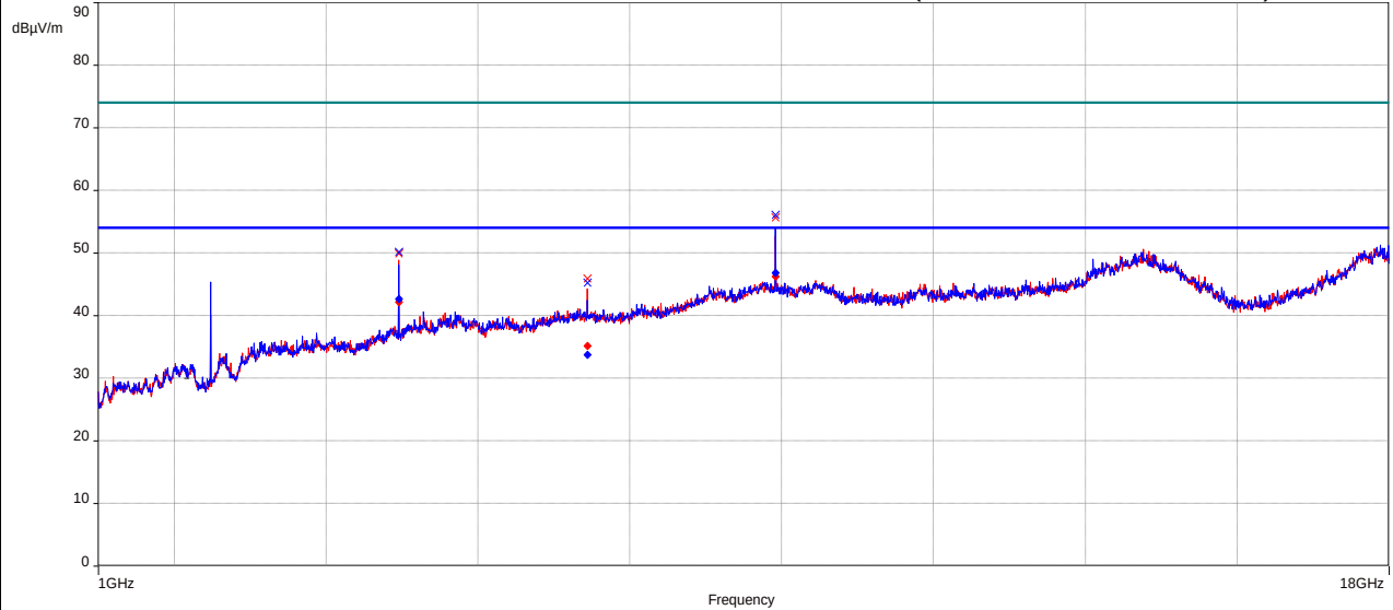
Transmitted Data. Wi-Fi and Bluetooth Radios at 2480 MHz. (Wi-Fi Radio is Worst Case)
