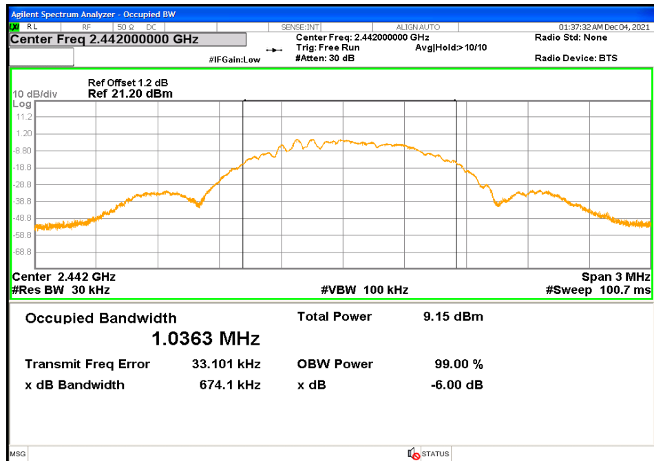
Figure 9: 99% Bandwidth-Headset - 2442 MHz
