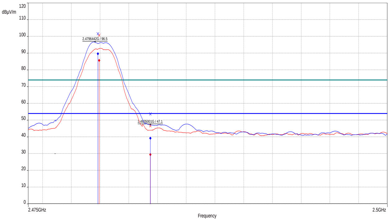
Figure 21: Band-edge-2480 MHz
