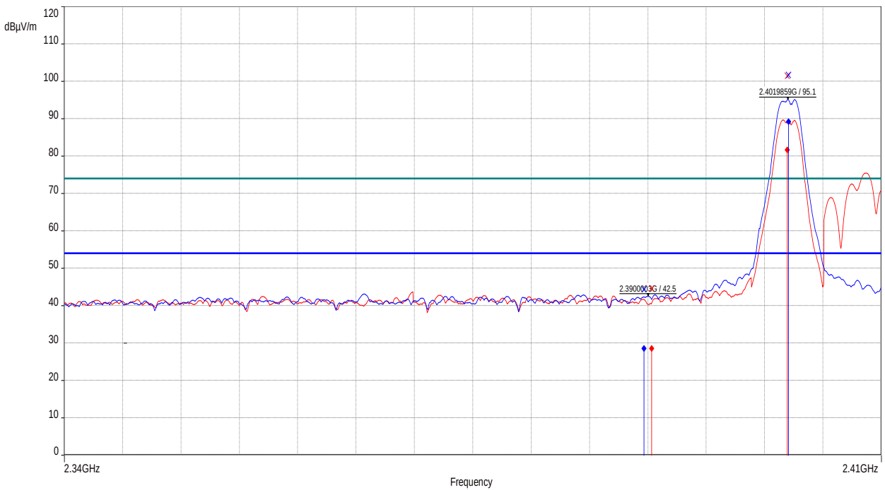
Figure 20: Band-edge-2402 MHz
