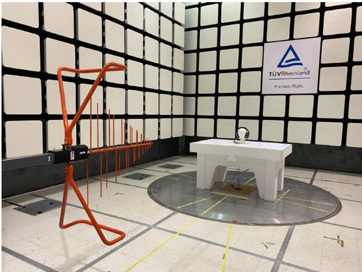
Figure 4: Test Setup for 30 MHz to 1000 MHz (Rear View)
