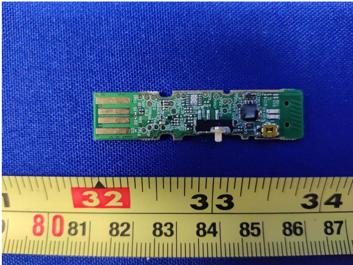
Figure 2: Internal Photo of Stealth600P-MAX-TX – Top PCB
