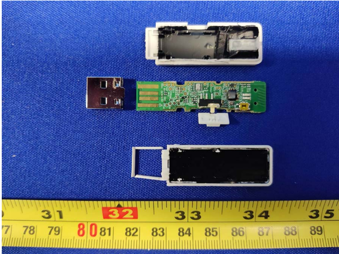
Figure 1: Internal Photo of Stealth600P-MAX-TX with Plastic Cover Removed
