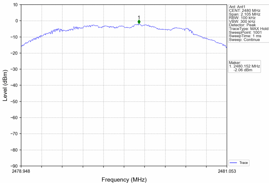
2.4G_HCH_2480MHz_Ant1_NTNV
