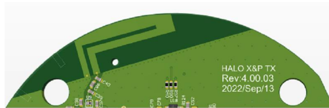
Figure 2 Antenna Placement
