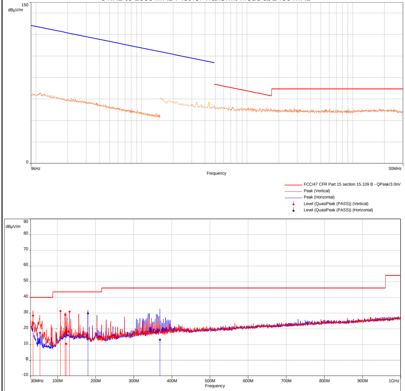
9 kHz to 1000 MHz Plot for Transmit Mode at 2480 MHz
