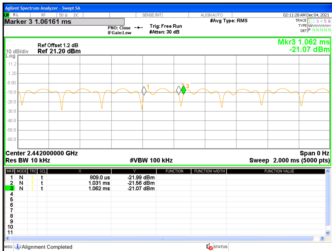
Figure 1: Duty Cycle
