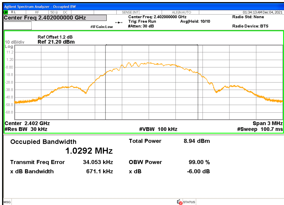
Figure 8: 99% Bandwidth-Headset -2402 MHz
