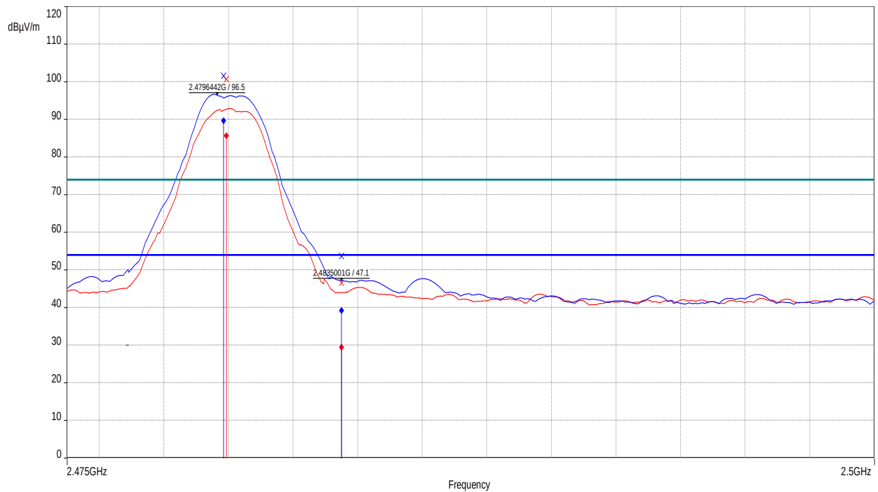
Figure 21: Band-edge-2480 MHz
