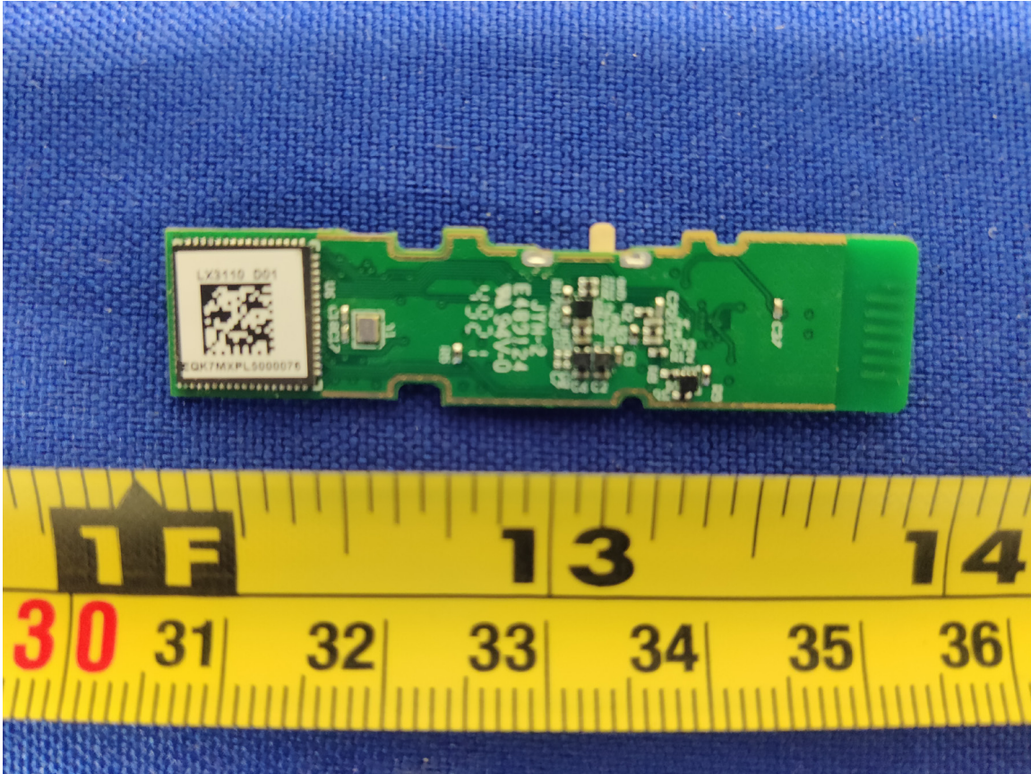
Figure 3: Internal Photo of Stealth700P-MAX-TX – Bottom PCB
