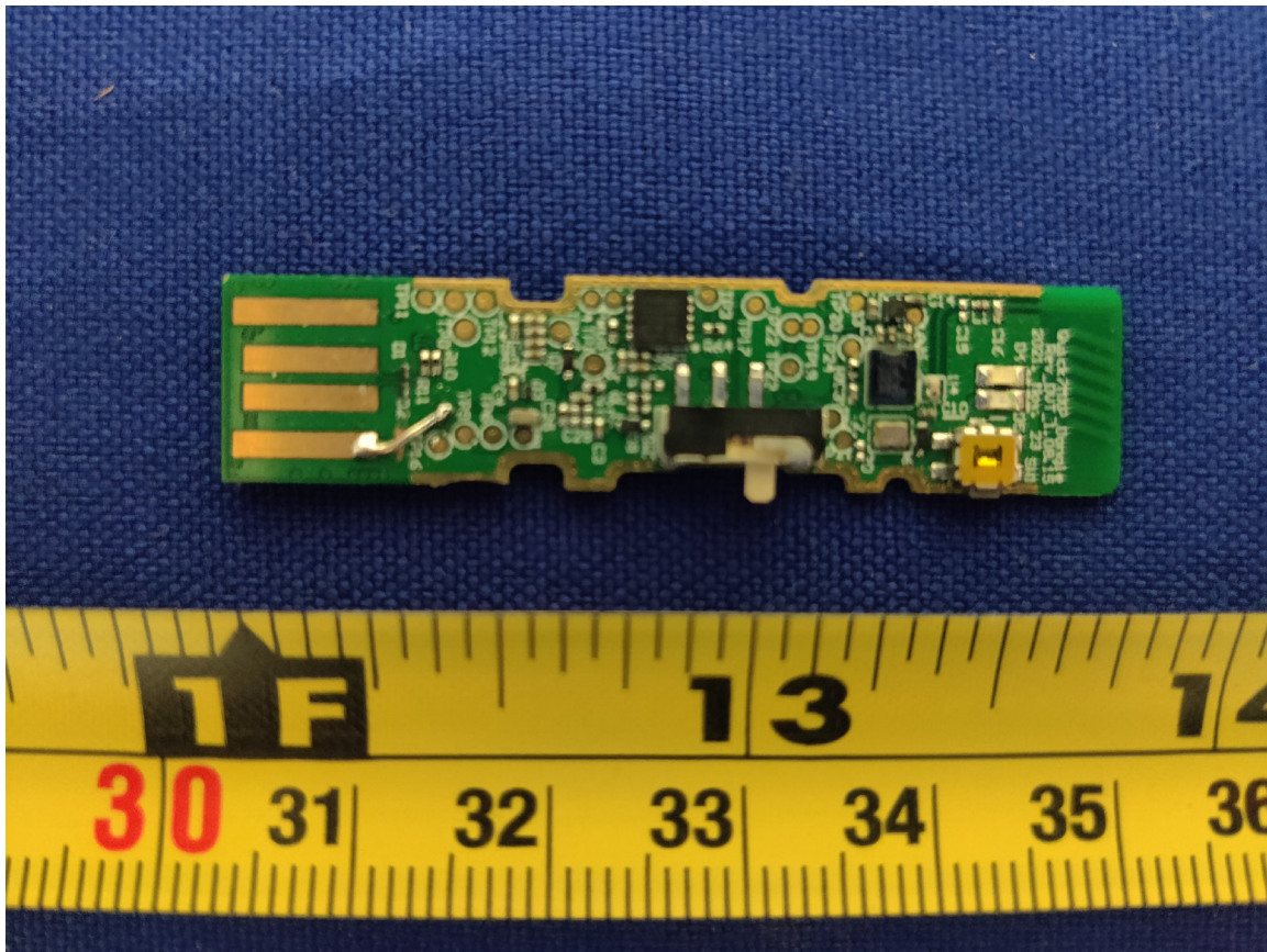
Figure 2: Internal Photo of Stealth700P-MAX-TX – Top PCB
