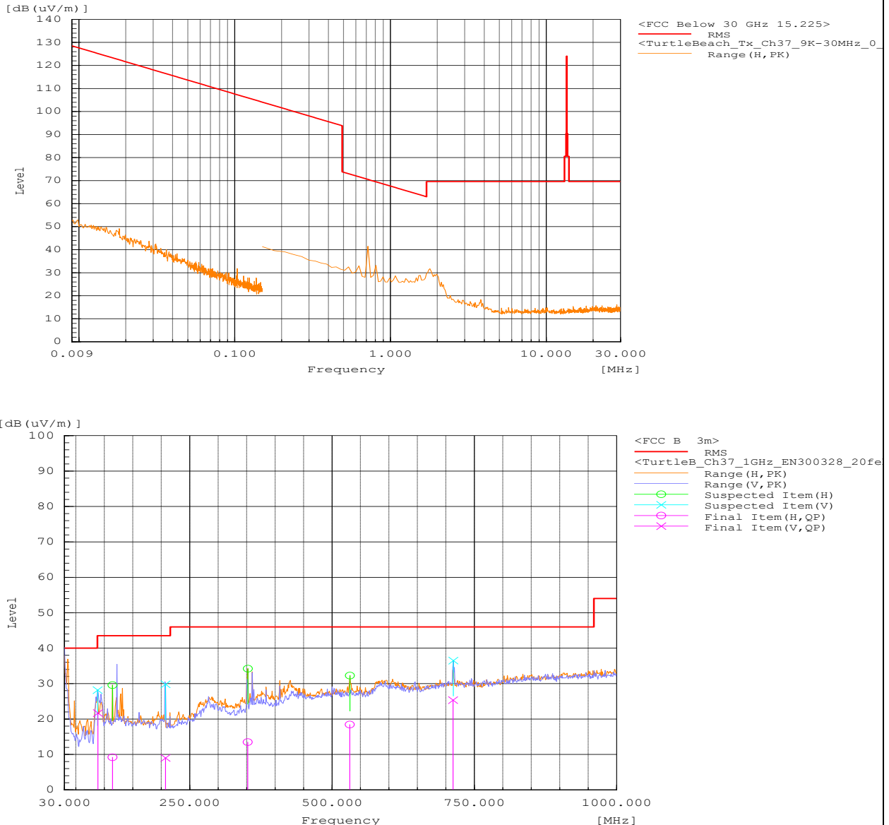
9 kHz to 1000 MHz Plot for Transmit Mode at 2402 MHz
