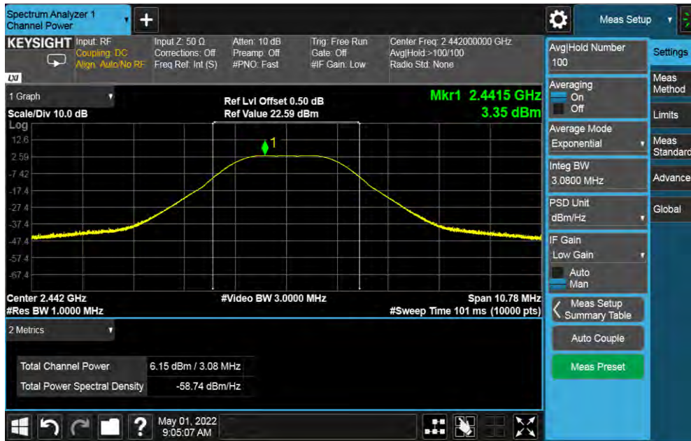
Figure 6: Maximum Conducted Output Power at 2442 MHz at 2Mbps
