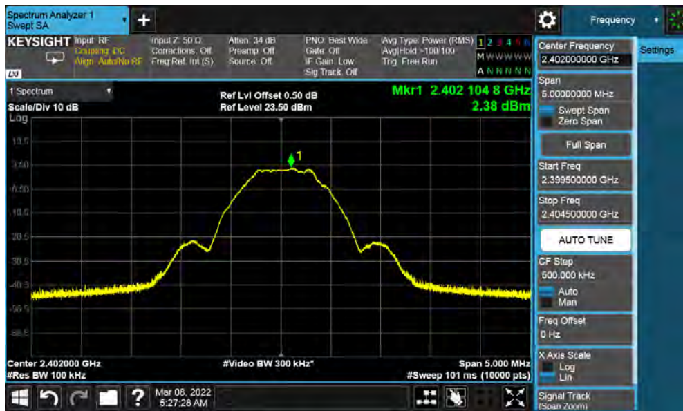
Figure 20: Maximum Power Spectral Density-2402 MHz at 1 Mbps
