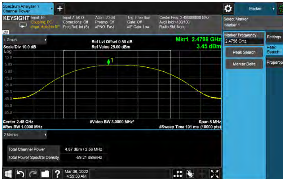
Figure 4: Maximum Conducted Output Power at 2480 MHz at 1Mbps
