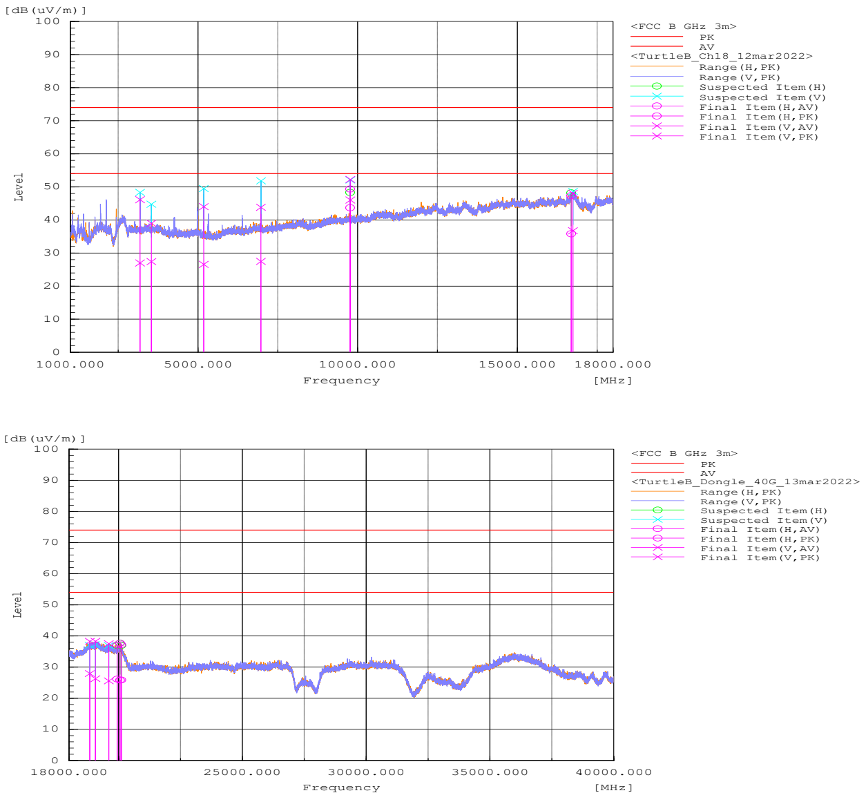
Above 1 GHz Plots for Transmit Mode at 2442 MHz
