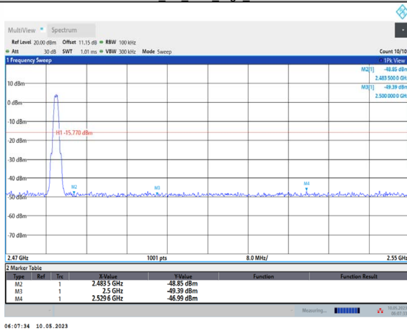
BLE_1M_Ant1_High_2480
