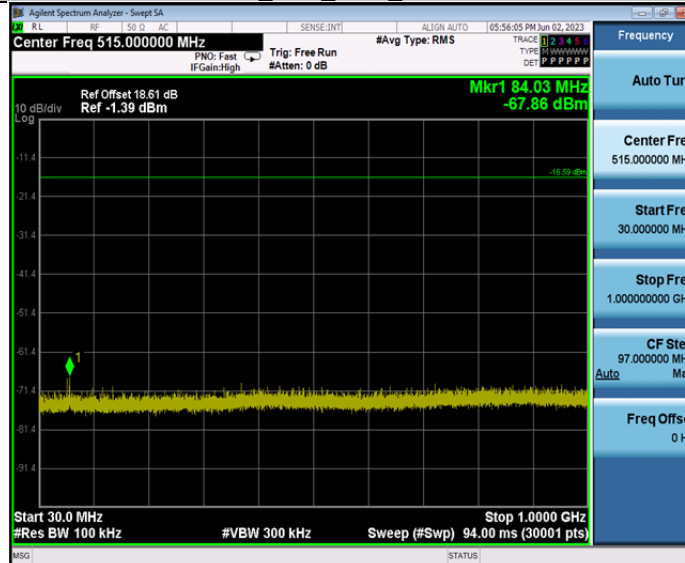
DH5_Ant1_2441_30~1000
