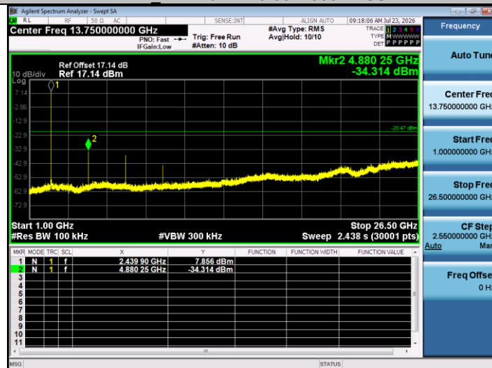
BLE_1M-Ant1-2440-1000~26500-PASS
