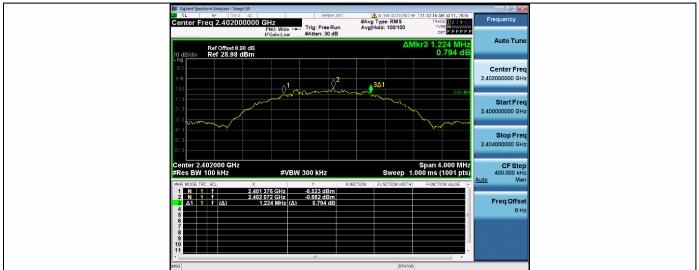
BLE_2M-Ant1-2402-PASS
