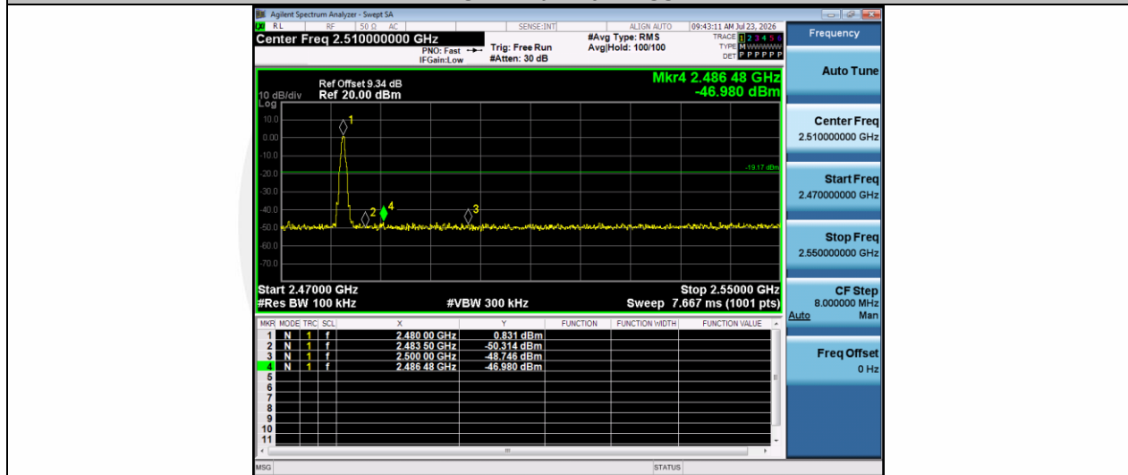
SRD-Ant1-2480-PASS
