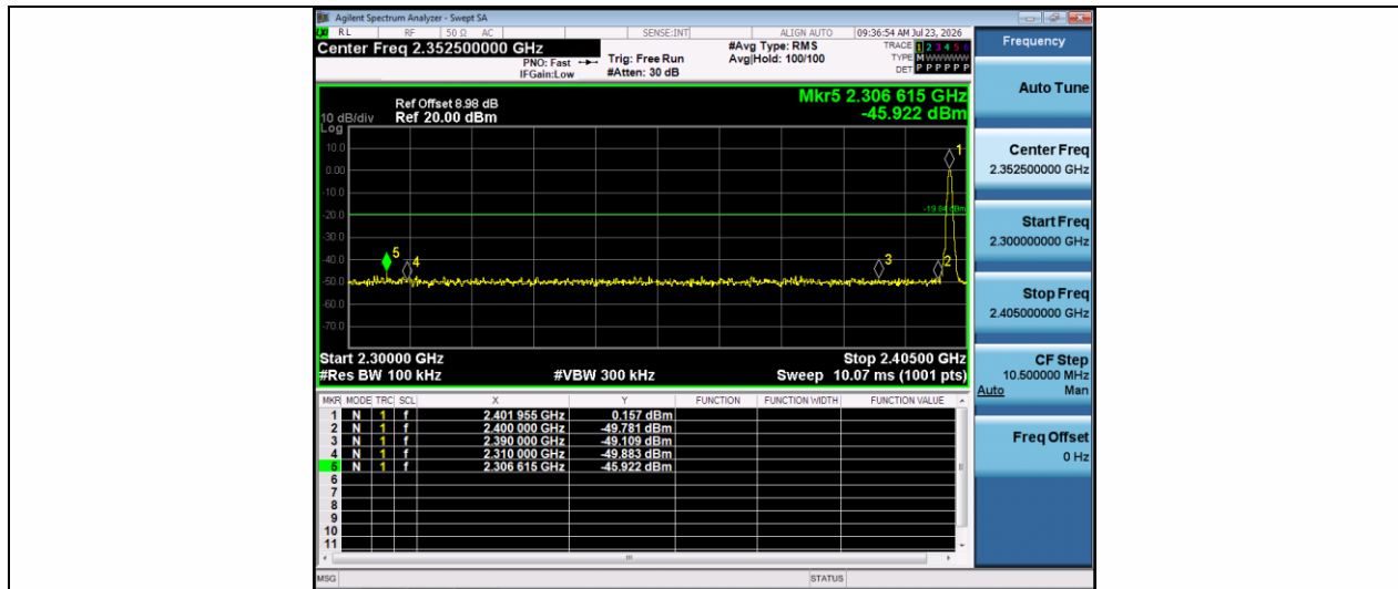
SRD-Ant1-2402-PASS
