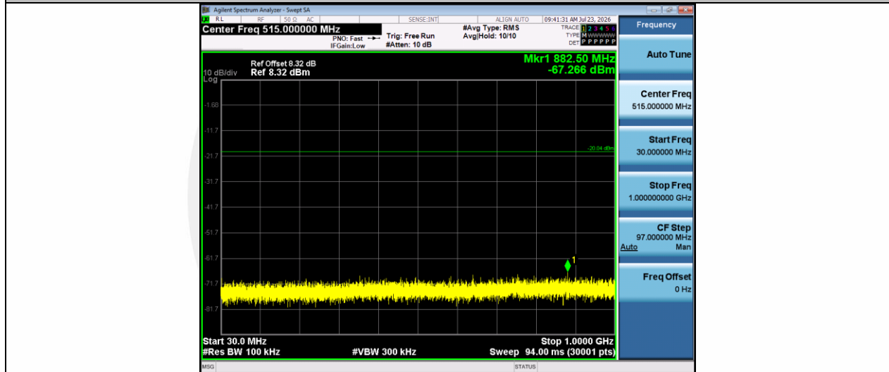
SRD-Ant1-2441-30~1000-PASS
