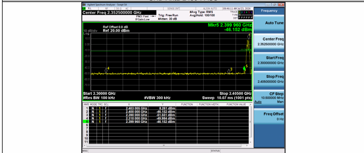
SRD-Ant1-Hop_2402-PASS
