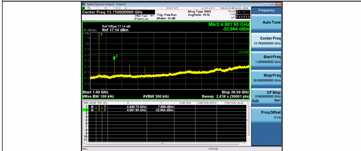
SRD-Ant1-2441-1000~26500-PASS
