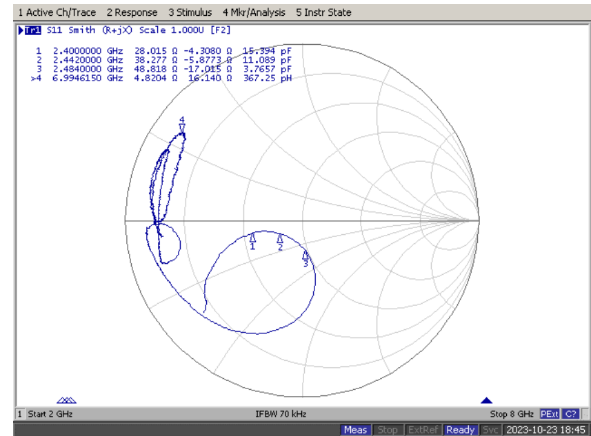
Smith chart
