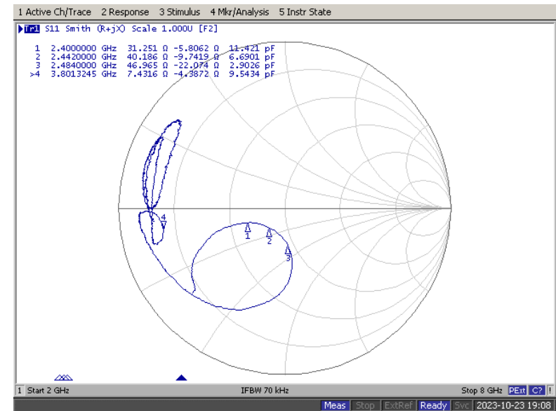
Smith chart
