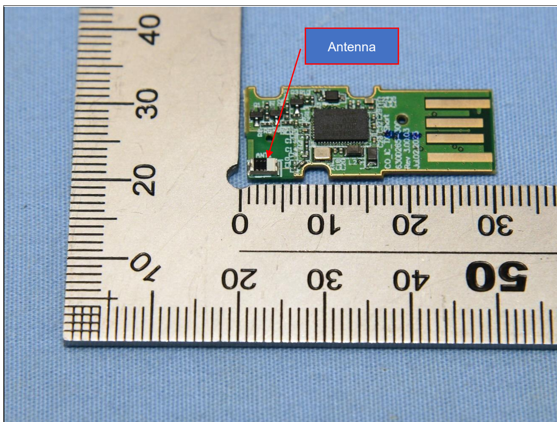
Type 2: For PC: without Encryption IC
