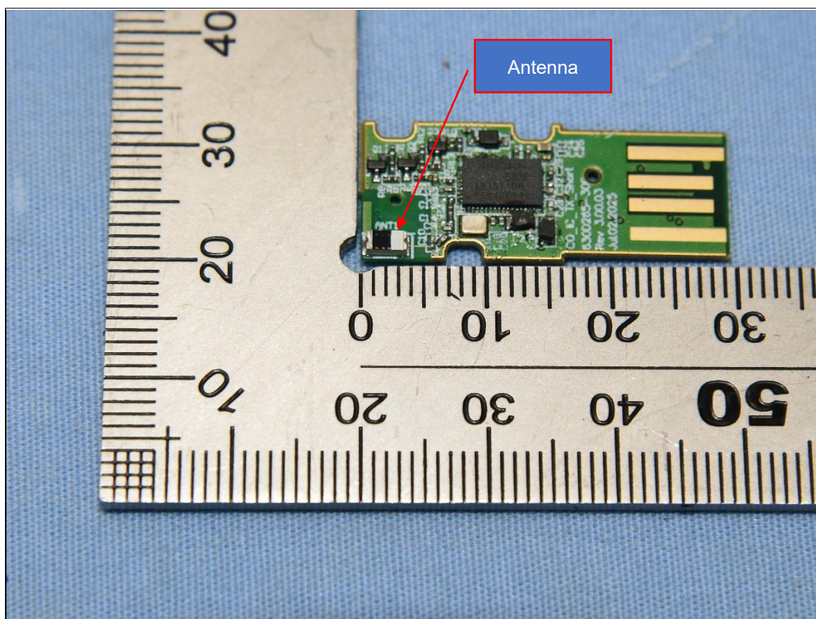
Type 1: For Xbox: with Encryprion IC
