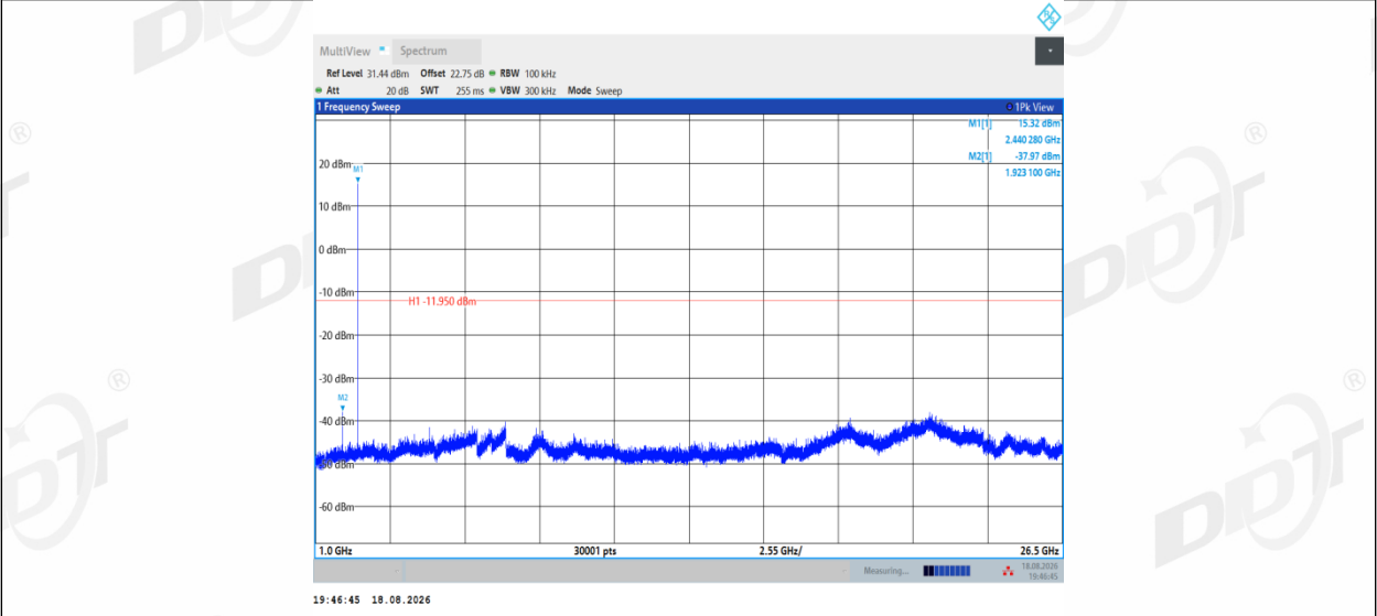
SRD_2M_Left side_2478_0~Reference
