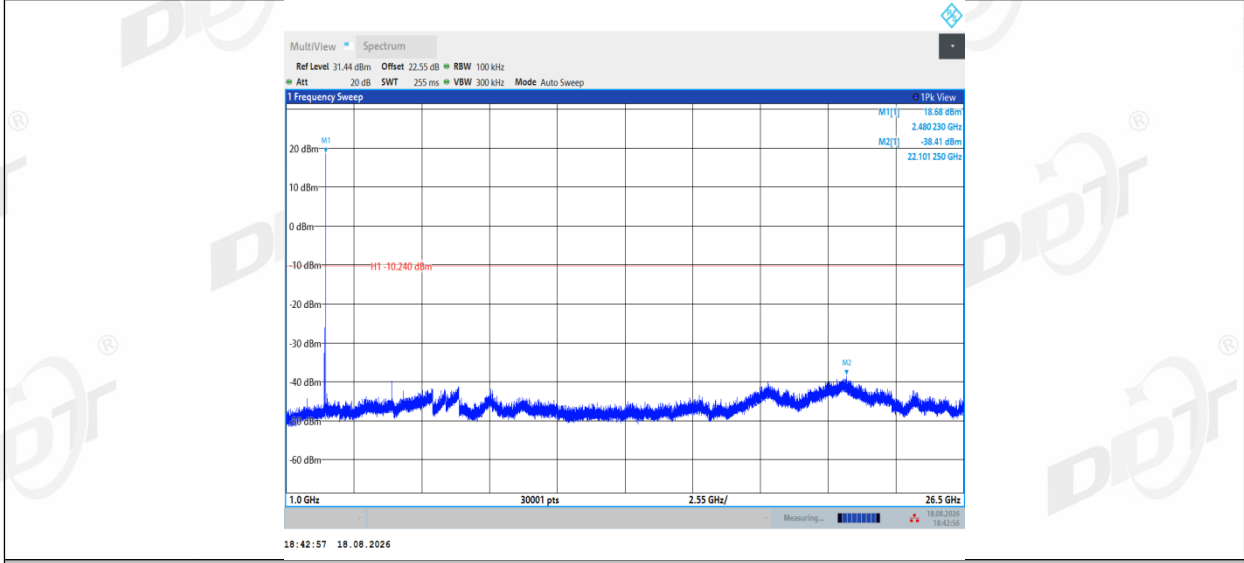
DH5_Right side_2480_0~Reference
