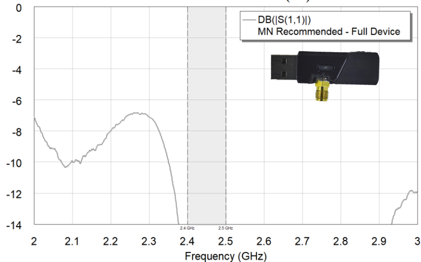
PEN FULL DEVICE S11(dB)
