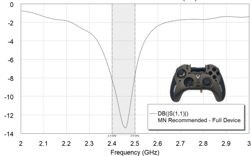
CONTROL FULL DEVICE S11(dB)
