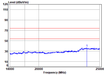
BLE_TX_CH_M_Horizontal
