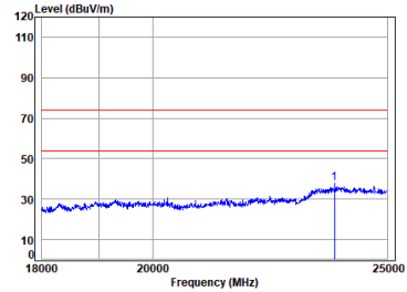
BLE_TX_CH_M_Vertical
