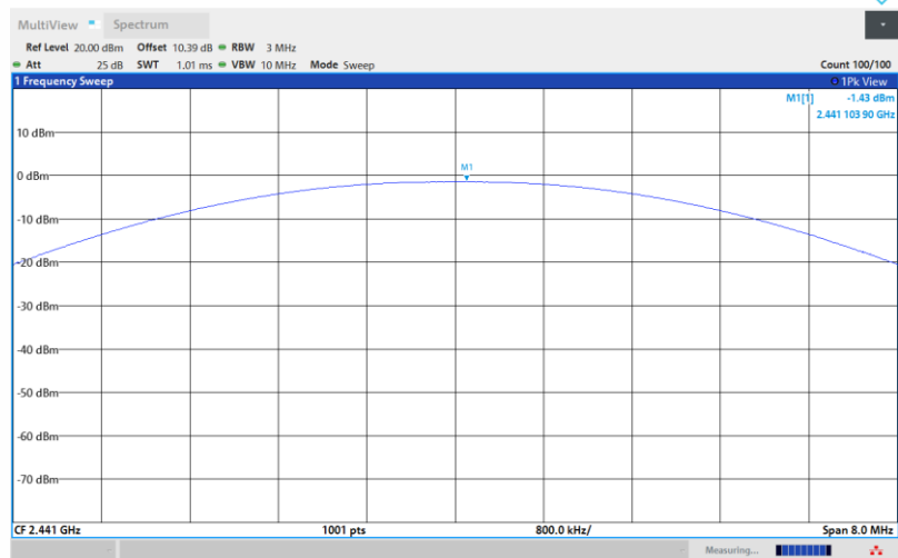
SRD-Ant1-2441-PASS
