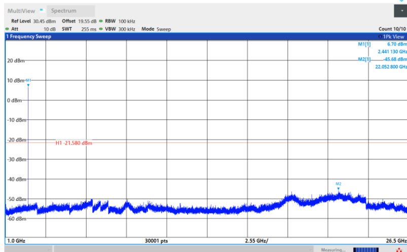
SRD-Ant1-2441-1000~26500-PASS
