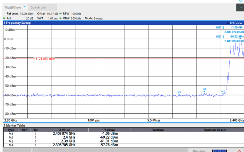
SRD-Ant1-Hop_2402-PASS
