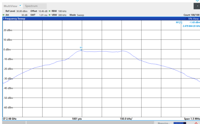
SRD-Ant1-2480-PASS
