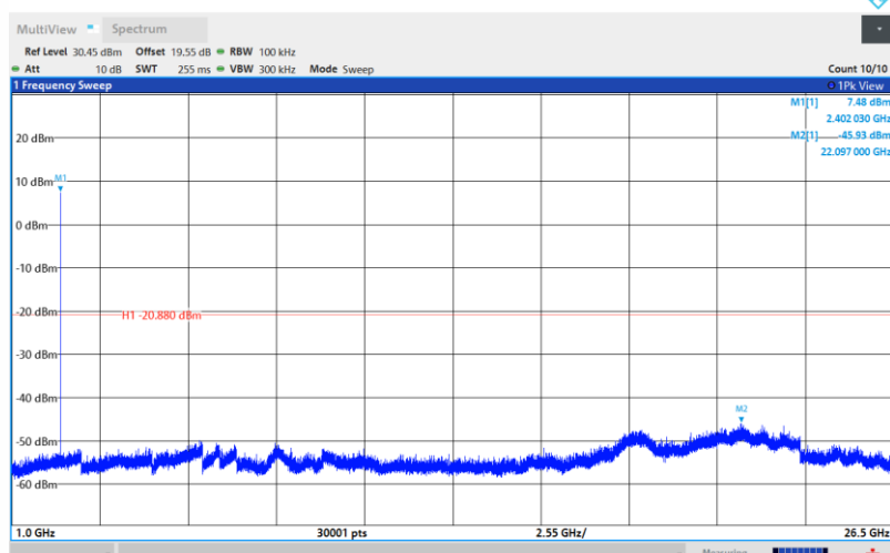
SRD-Ant1-2402-1000~26500-PASS
