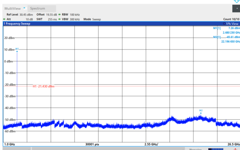
SRD-Ant1-2480-1000~26500-PASS
