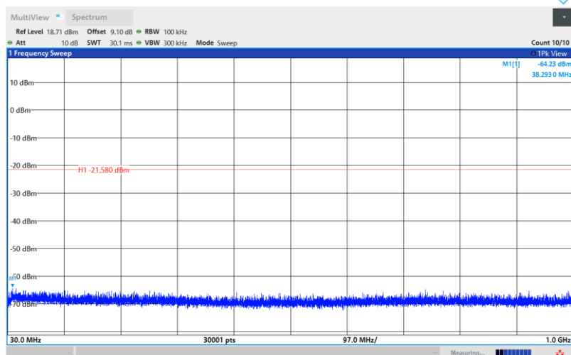
SRD-Ant1-2441-30~1000-PASS
