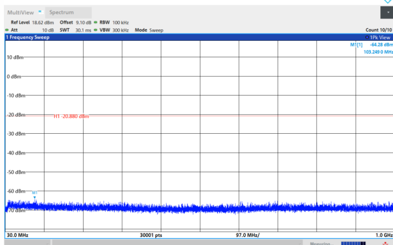
SRD-Ant1-2402-30~1000-PASS
