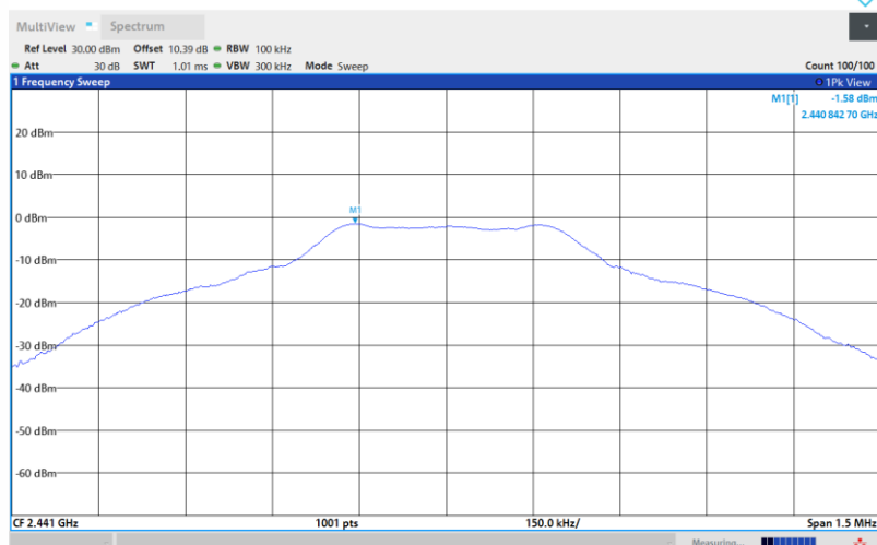
SRD-Ant1-2441-PASS
