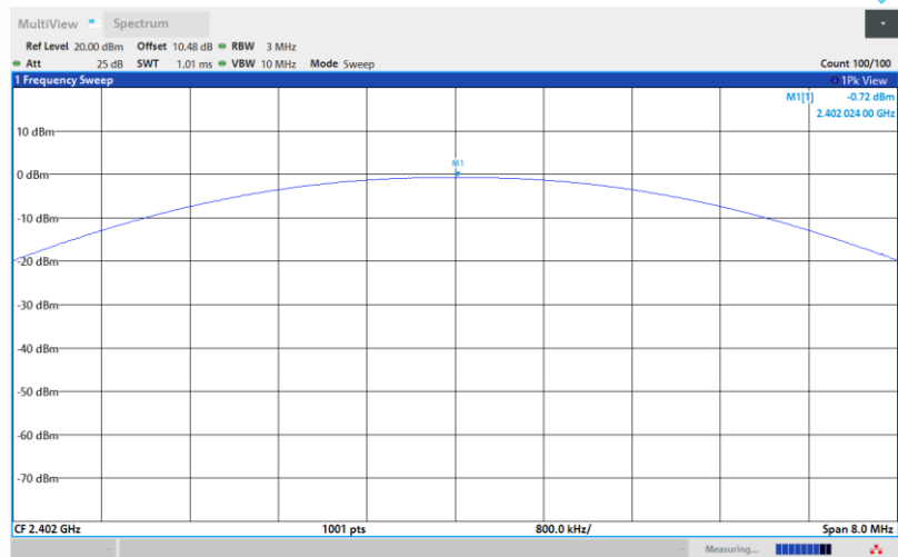
SRD-Ant1-2402-PASS
