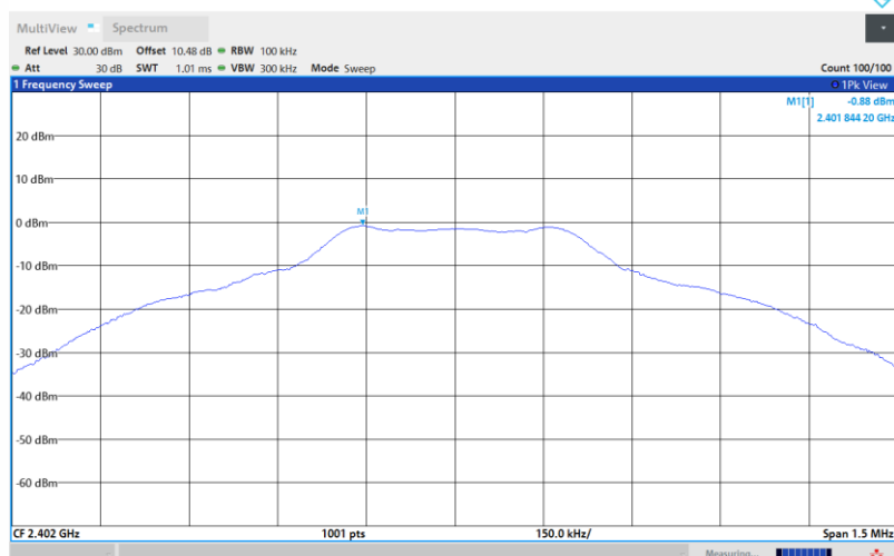
SRD-Ant1-2402-PASS
