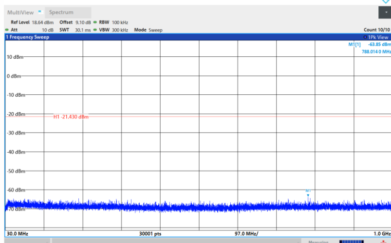
SRD-Ant1-2480-30~1000-PASS
