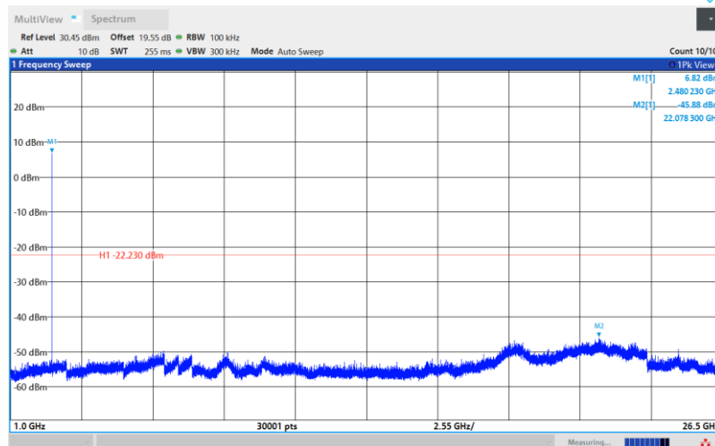
BLE_1M-Ant1-2480-1000~26500-PASS
