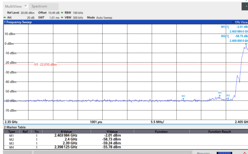
BLE_2M-Ant1-2404-PASS
