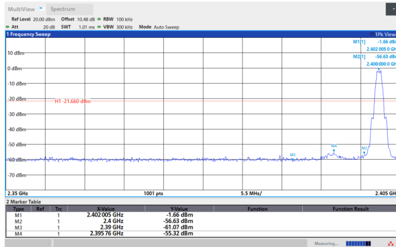
BLE_1M-Ant1-2402-PASS
