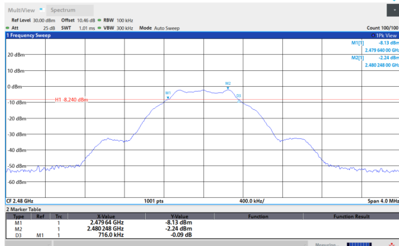
BLE_1M-Ant1-2480-PASS
