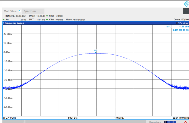
BLE_1M-Ant1-2440-PASS
