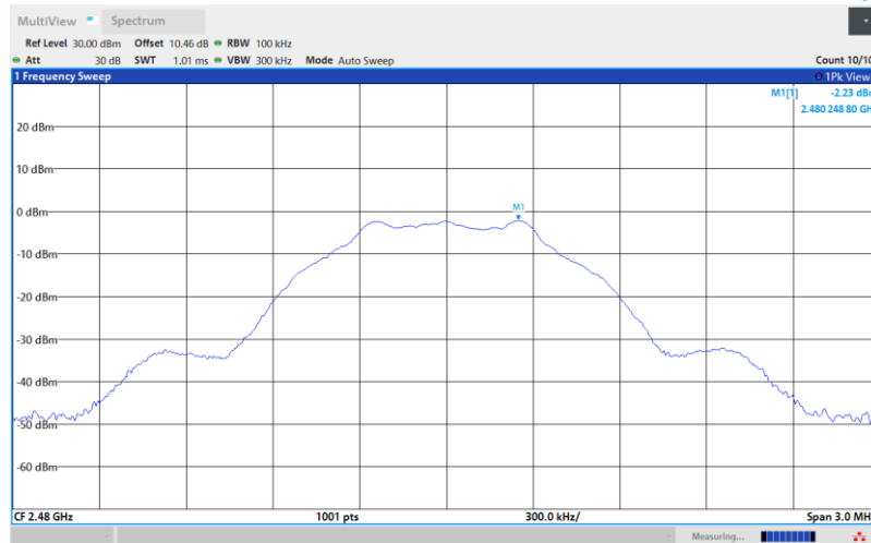
BLE_1M-Ant1-2480-0-Reference-PASS
