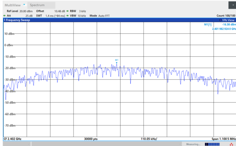
BLE_1M-Ant1-2402-PASS
