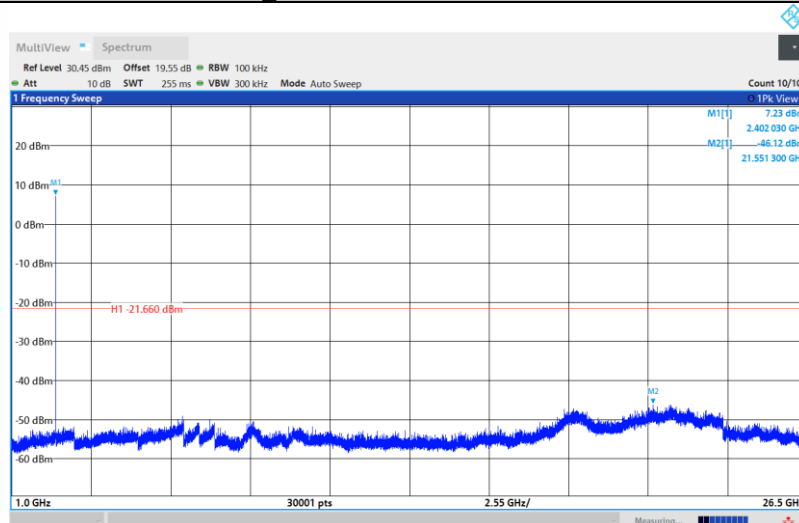
BLE_1M-Ant1-2402-1000~26500-PASS
