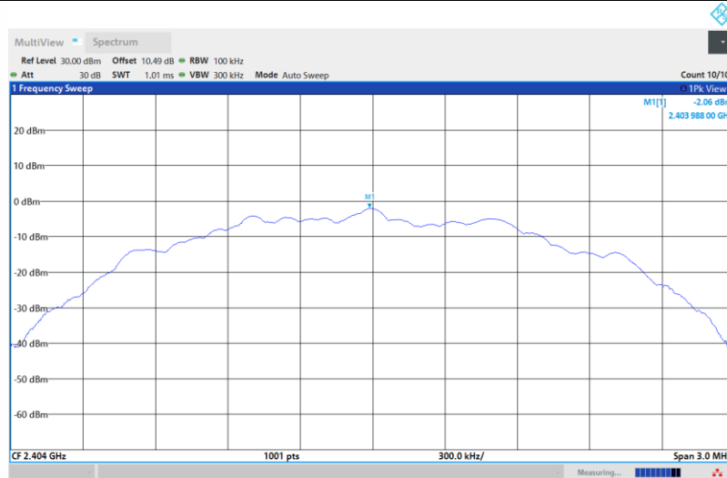
BLE_2M-Ant1-2404-0-Reference-PASS
