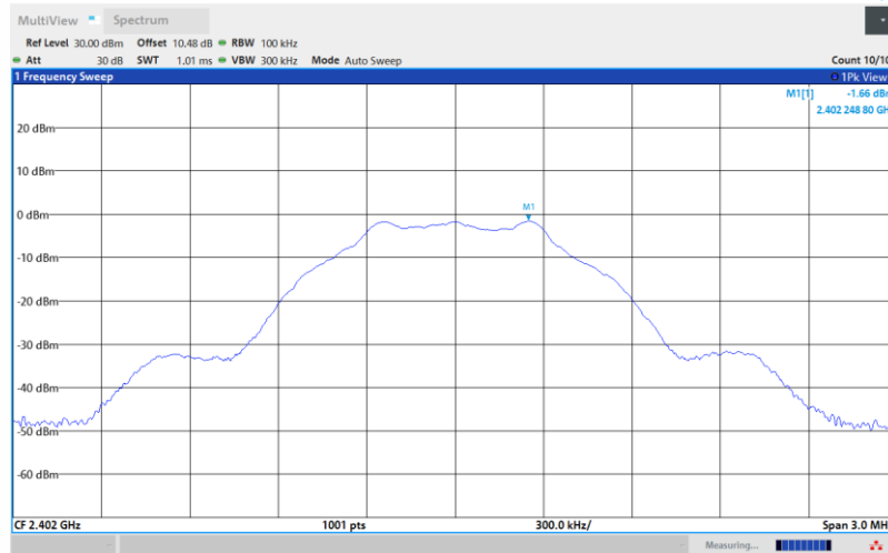
BLE_1M-Ant1-2402-0-Reference-PASS
