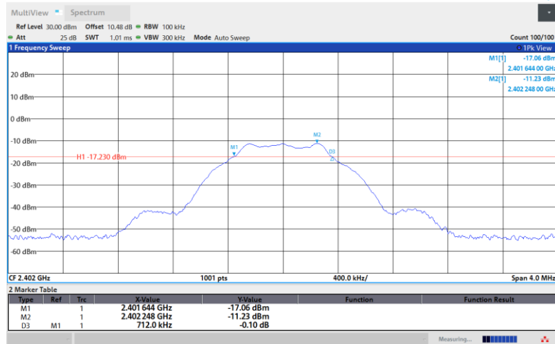
BLE_1M-Ant1-2402-PASS
