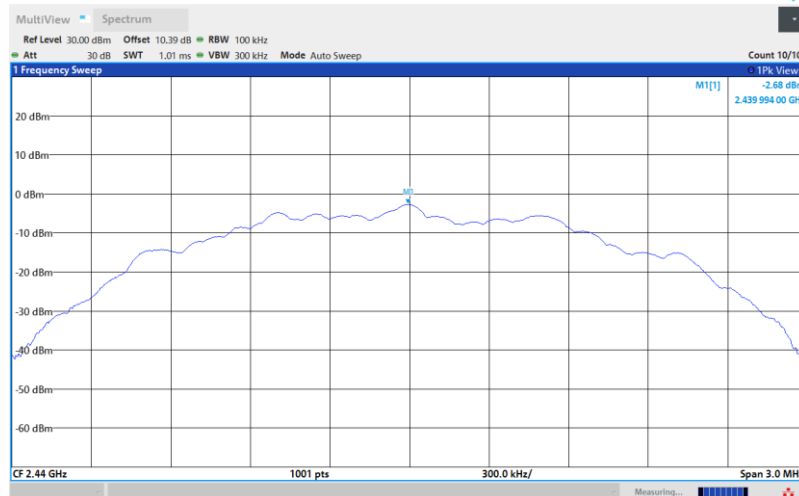
BLE_2M-Ant1-2440-0-Reference-PASS
