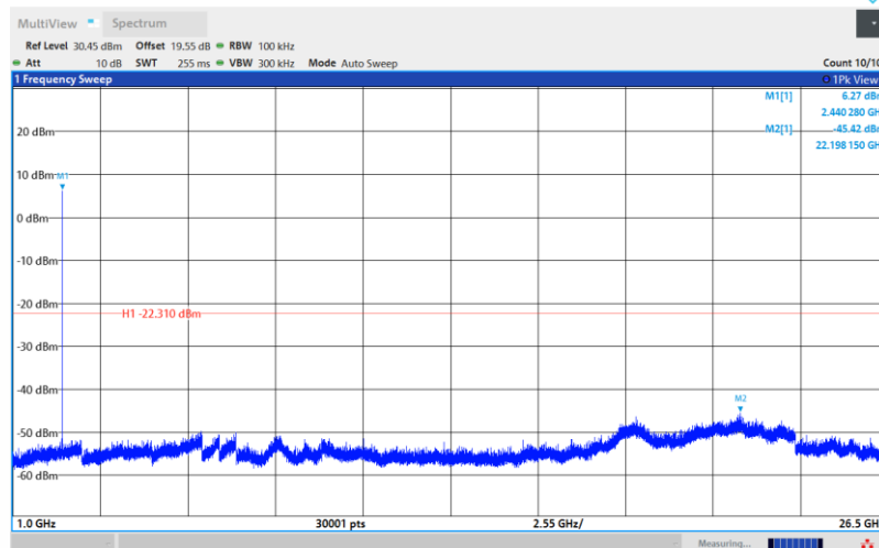
BLE_1M-Ant1-2440-1000~26500-PASS
