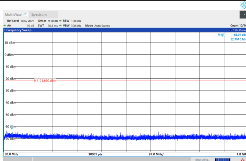
BLE_1M-Ant1-2402-30~1000-PASS
