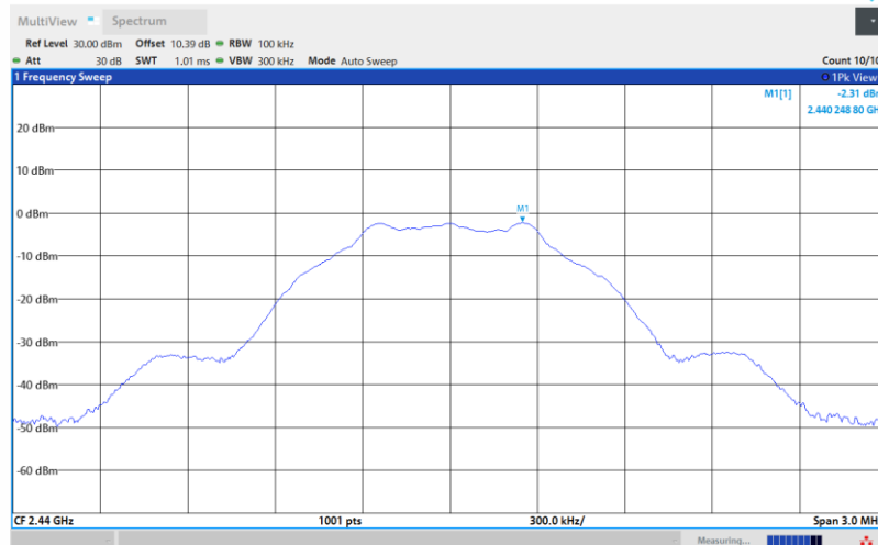
BLE_1M-Ant1-2440-0-Reference-PASS
