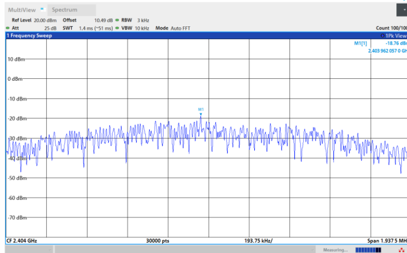
BLE_2M-Ant1-2404-PASS
