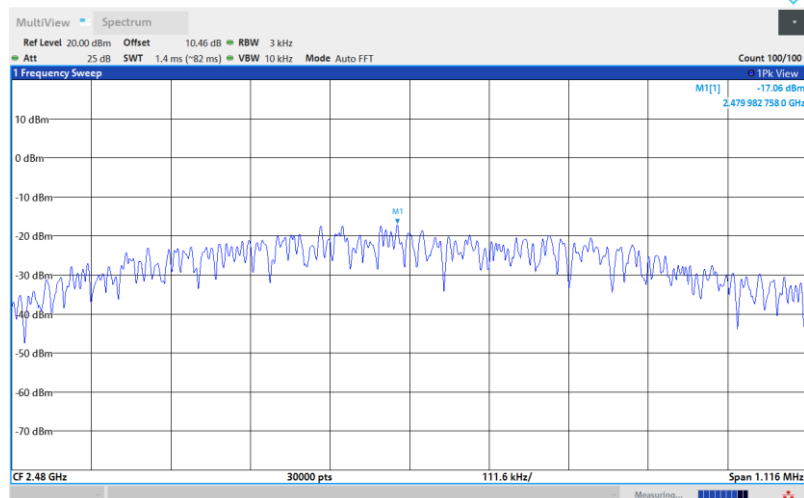
BLE_1M-Ant1-2480-PASS
