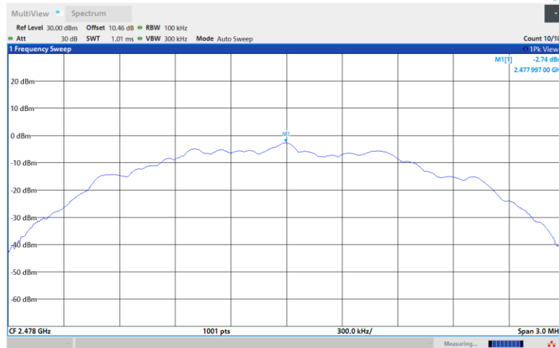
BLE_2M-Ant1-2478-0-Reference-PASS
