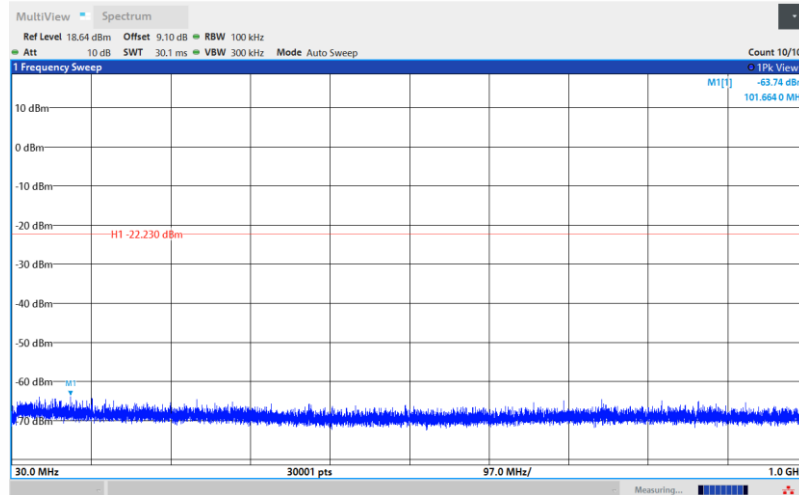
BLE_1M-Ant1-2480-30~1000-PASS
