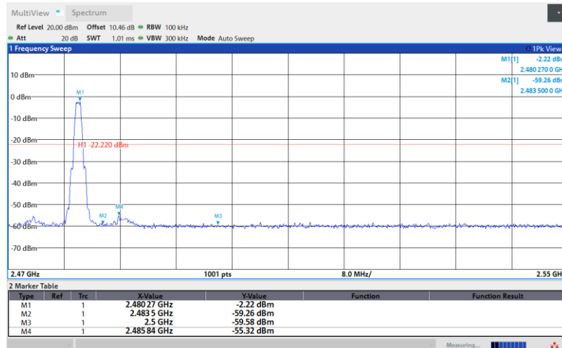
BLE_1M-Ant1-2480-PASS
