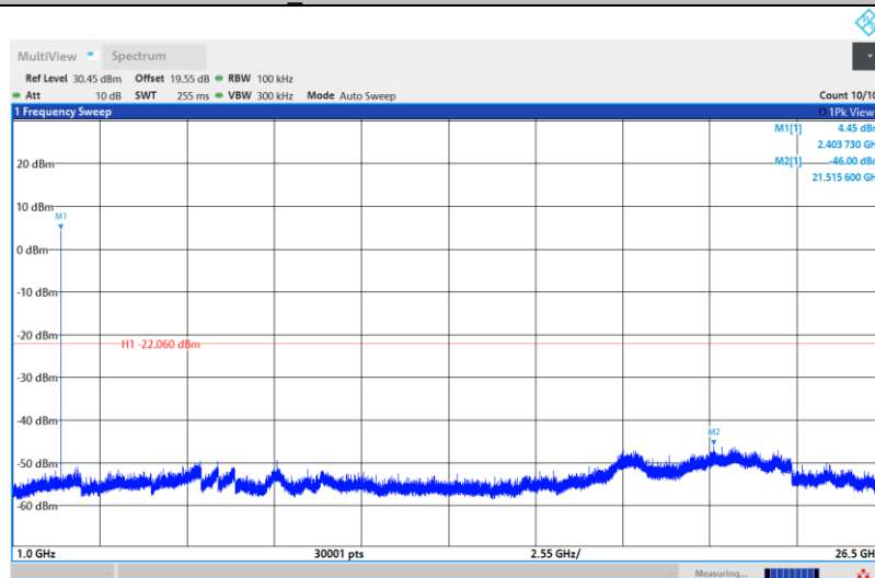
BLE_2M-Ant1-2404-1000~26500-PASS
