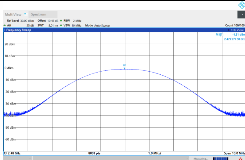
BLE_1M-Ant1-2480-PASS
