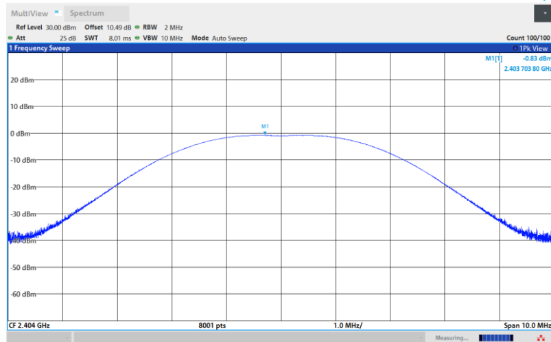
BLE_2M-Ant1-2404-PASS
