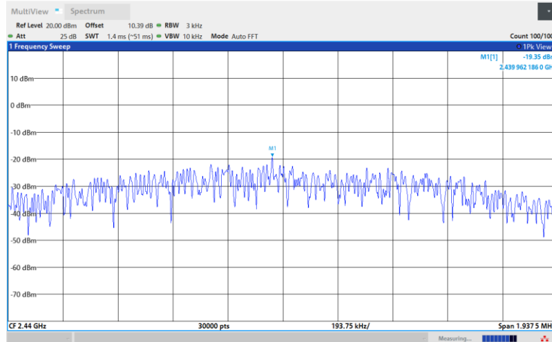
BLE_2M-Ant1-2440-PASS
