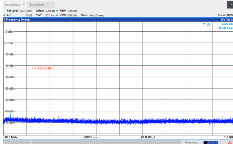
BLE_1M-Ant1-2440-30~1000-PASS
