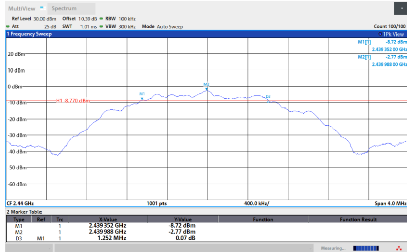
BLE_2M-Ant1-2440-PASS
