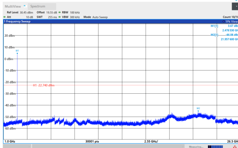
BLE_2M-Ant1-2478-1000~26500-PASS
