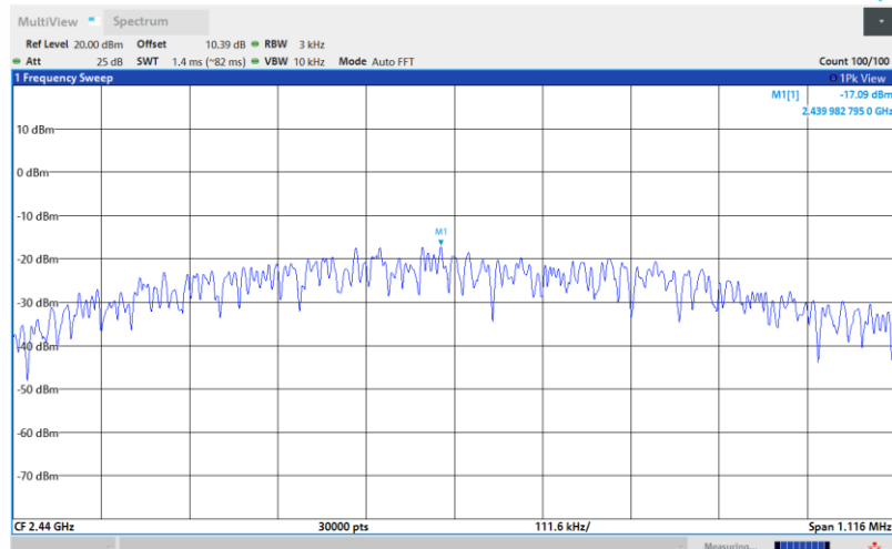
BLE_1M-Ant1-2440-PASS
