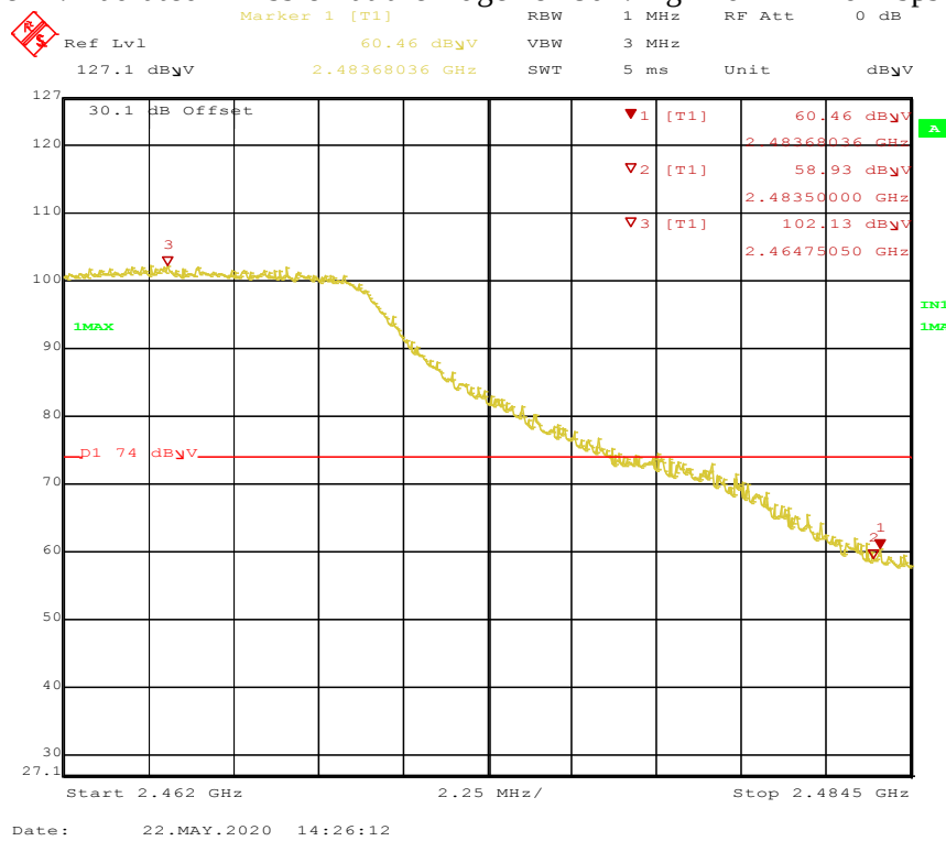
Figure 73: Radiated Emission at the Edge for 802.11g-2462 MHz-6 Mbps-V-Pk
