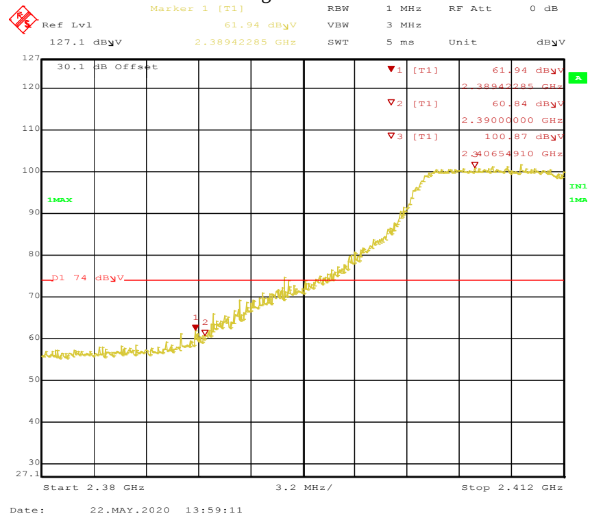
Figure 75: Radiated Emission at the Edge for 802.11n HT20-2412 MHz-6.5 Mbps-V-Pk
