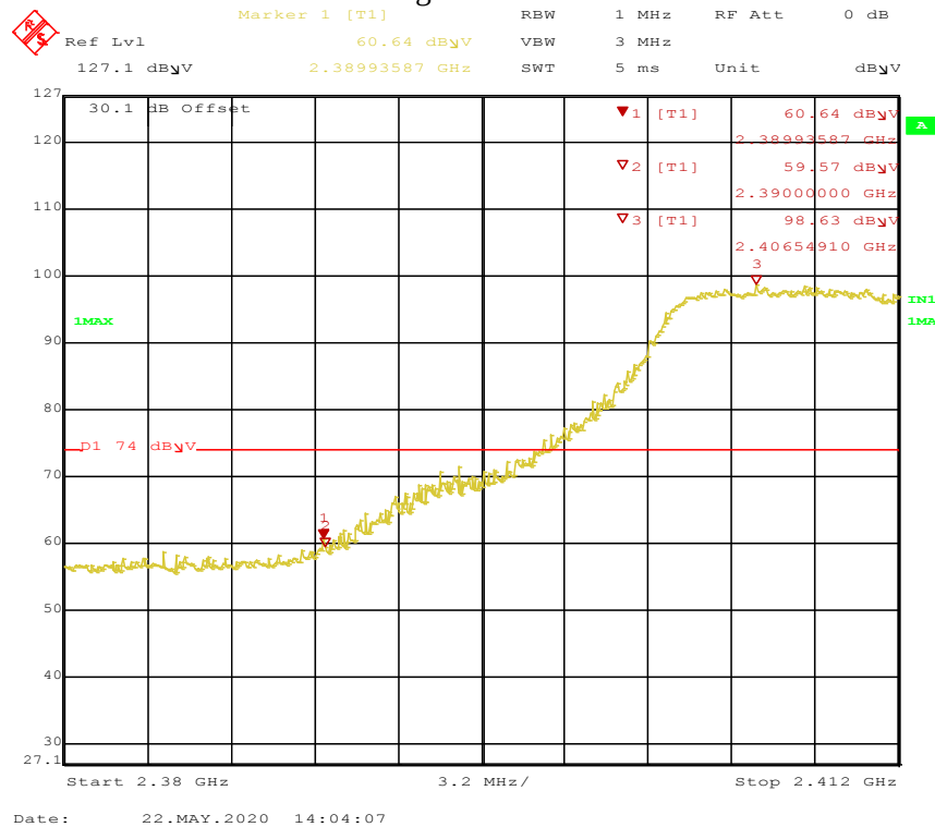
Figure 77: Radiated Emission at the Edge for 802.11n HT20-2412 MHz-6.5 Mbps-H-Pk
