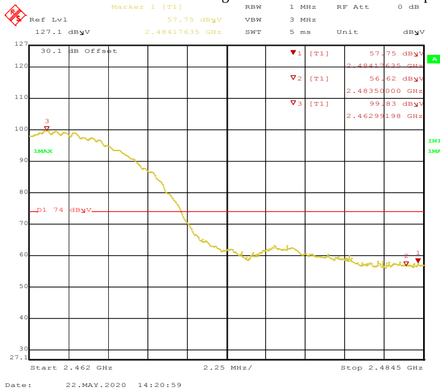
Figure 65: Radiated Emission at the Edge for 802.11b-2462 MHz-1 Mbps-V-Pk
