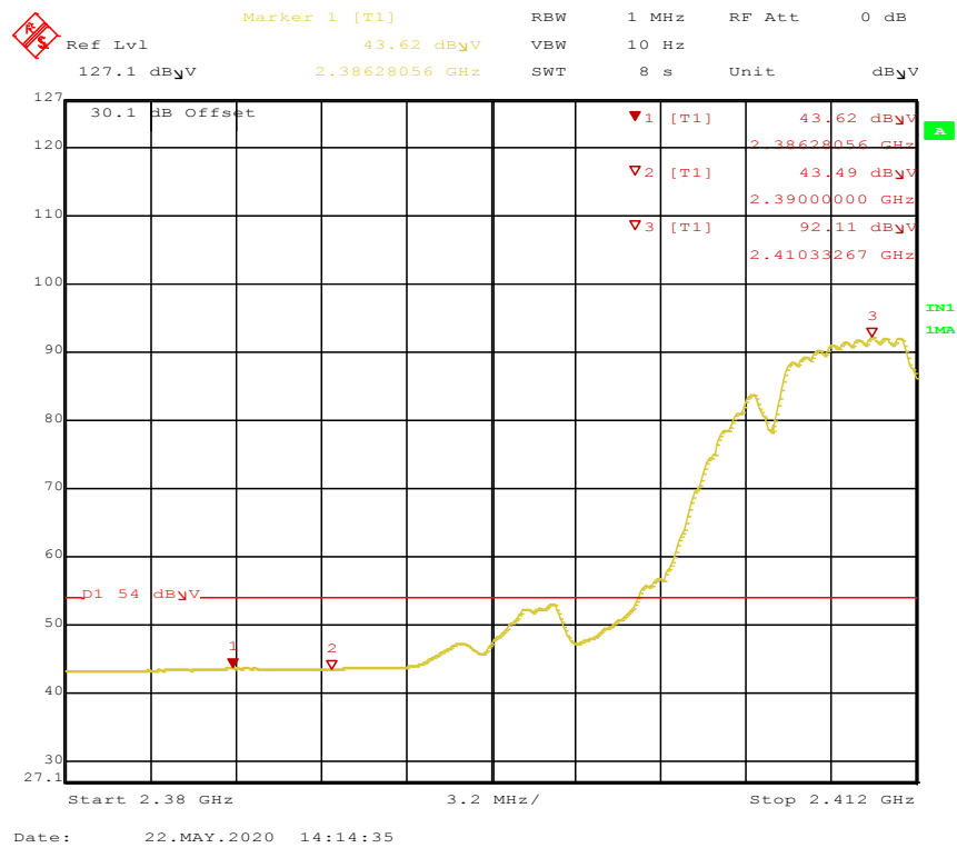
Figure 60: Radiated Emission at the Edge for 802.11b-2412 MHz-1 Mbps-H-Ave
