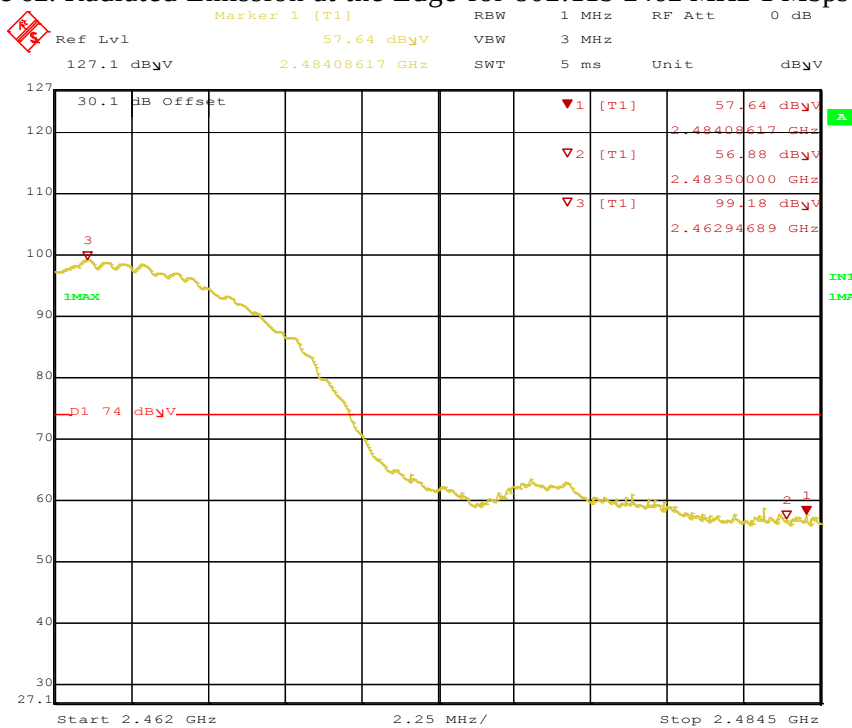
Figure 63: Radiated Emission at the Edge for 802.11b-2462 MHz-1 Mbps-H-Pk
