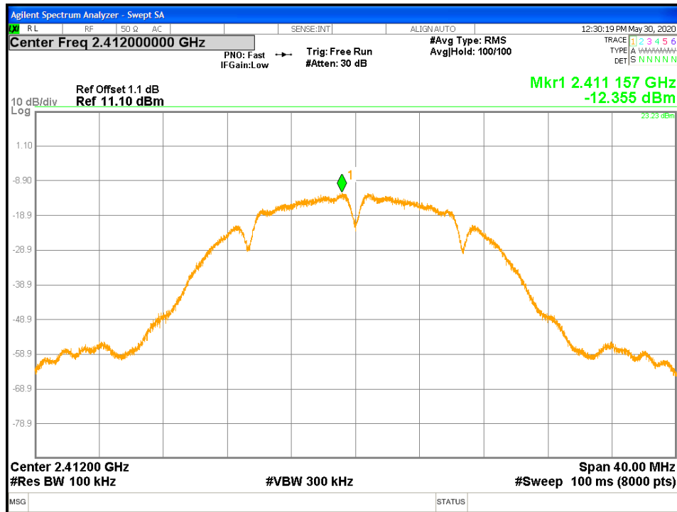
Figure 31: Maximum Power Spectral Density-2412 MHz-802.11b-1 Mbps
