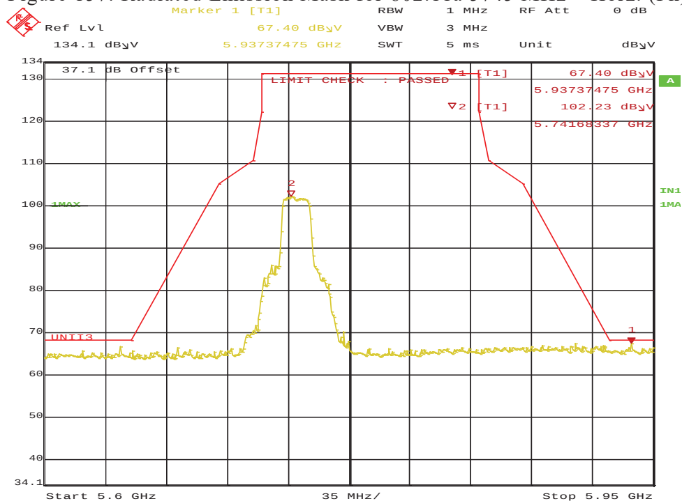
Figure 158: Radiated Emission Mask for 802.11a 5745 MHz – Vert (Pk)
