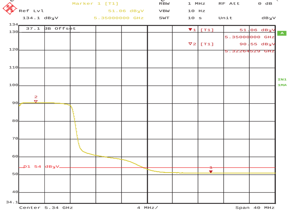
Figure 133: Radiated Emission 5350.0 MHz Edge for 802.11a 5320 MHz – Horiz. (Pk)
