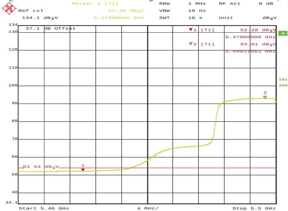
Figure 145: Radiated Emission 5470.0 MHz Edge for 802.11n HT20 5500 MHz – Horiz. (Pk)
