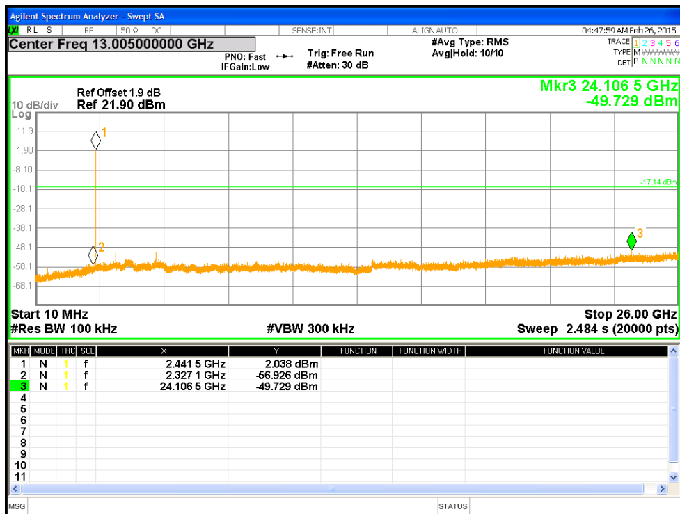
Figure 16: Out of Band Emission Requirements at 2442 MHz – DH5
