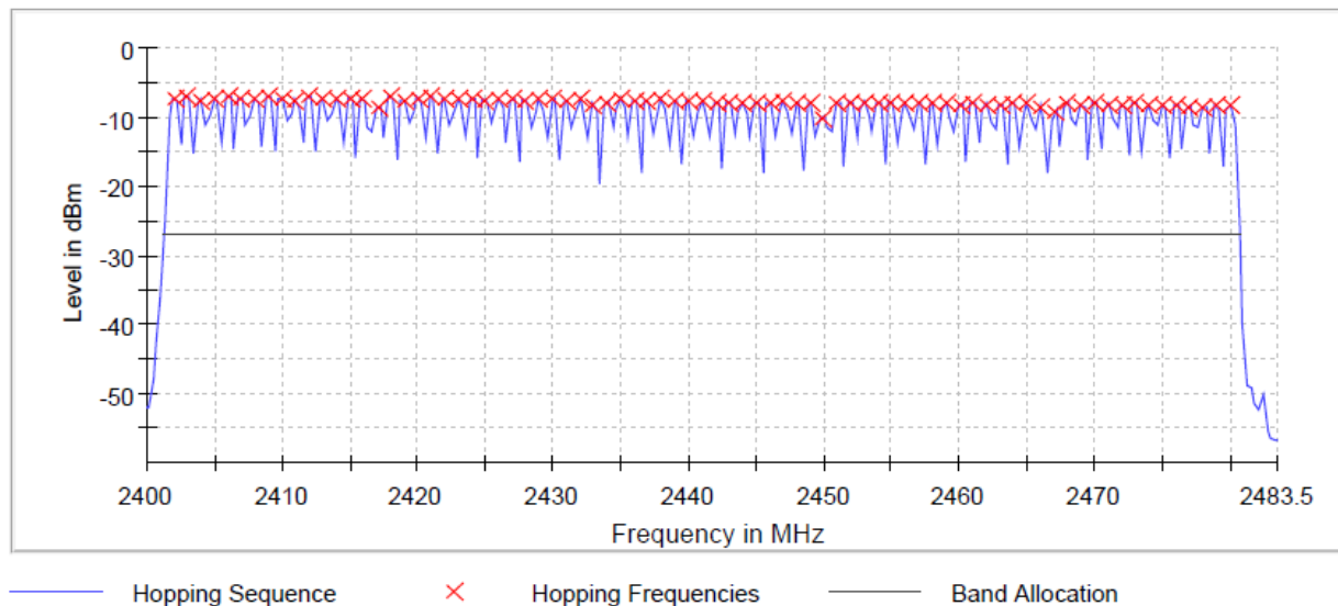
Figure 10: Number of Operating Channels (79)
