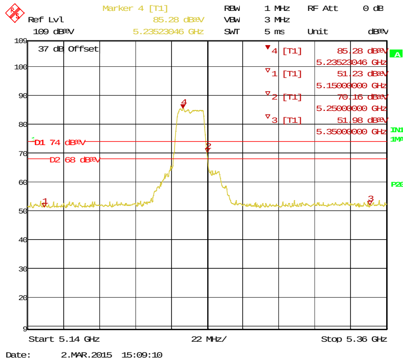
Figure 19: Bandedge-5240 MHz-11a-V-Pk
