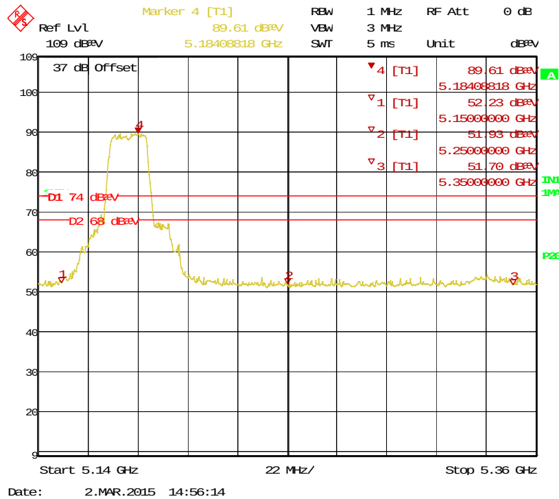
Figure 13: Bandedge-5180 MHz-11a-H-Pk
