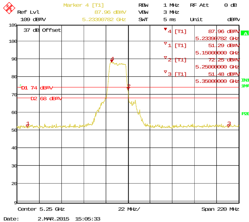
Figure 17: Bandedge-5240 MHz-11a-H-Pk
