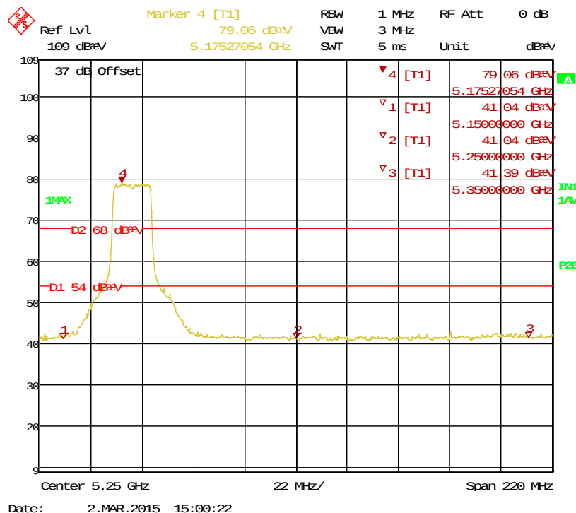
Figure 16: Bandedge-5180 MHz-11a-V-Ave
