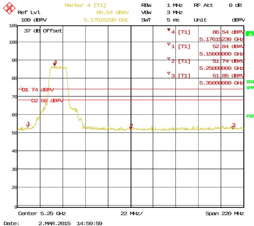
Figure 15: Bandedge-5180 MHz-11a-V-pk
