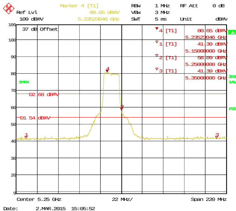
Figure 18: Bandedge-5240 MHz-11a-H-Ave
