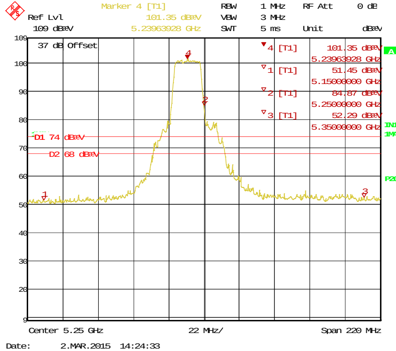
Figure 14: Bandedge-5240 MHz-11a-H-Pk
