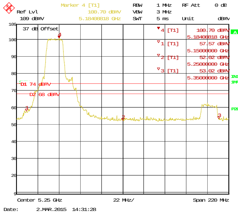
Figure 10: Bandedge-5180 MHz-11a-H-Pk
