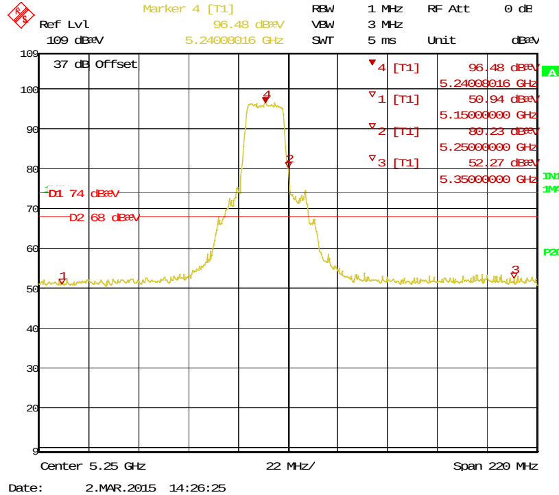
Figure 16: Bandedge-5240 MHz-11a-V-Pk
