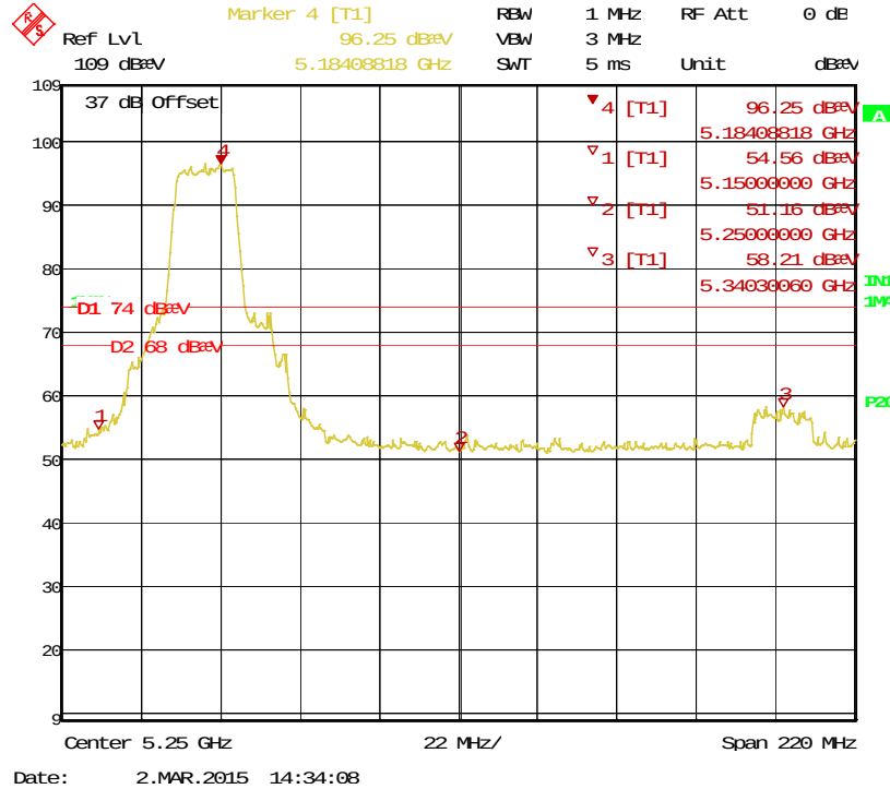
Figure 12: Bandedge-5180 MHz-11a-V-pk
