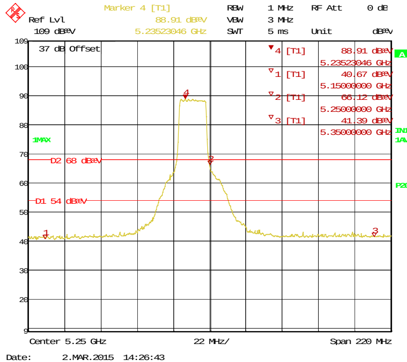
Figure 17: Bandedge-5240 MHz-V-Ave
