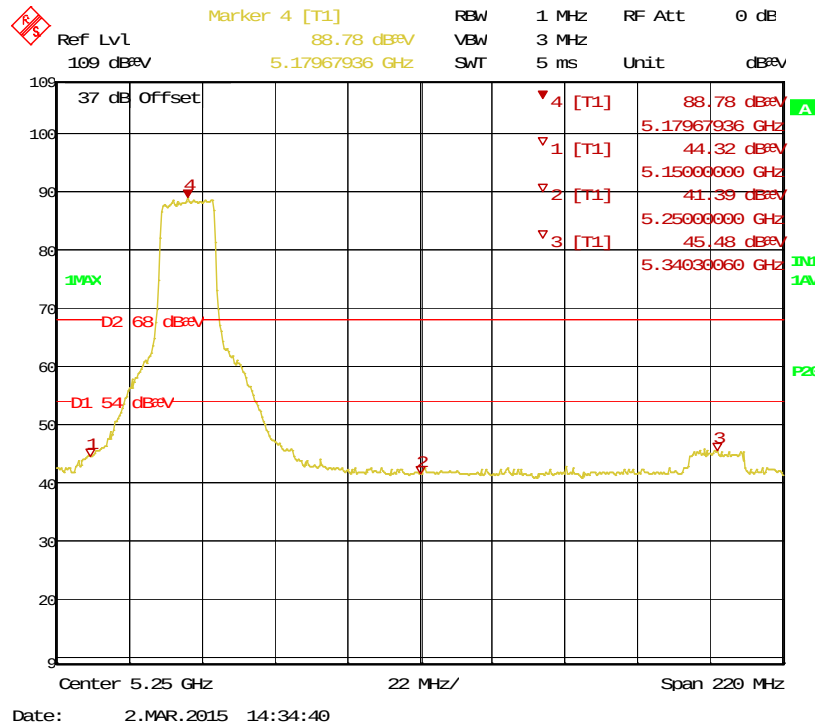
Figure 13: Bandedge-5180 MHz-11a-V-Ave
