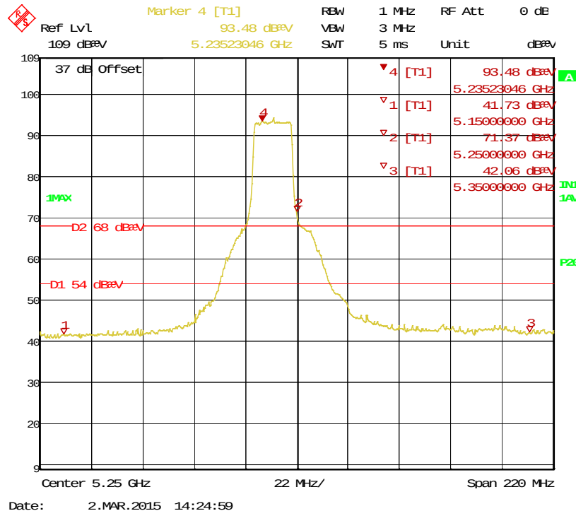
Figure 15: Bandedge-5240 MHz-11a-H-Ave
