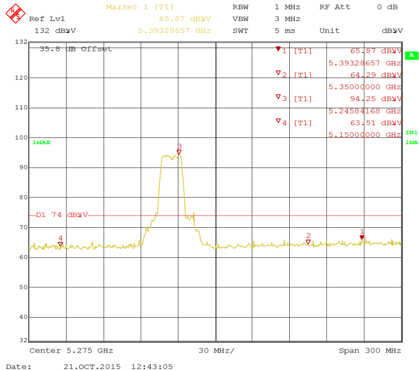
Figure 23: Radiated Emission 5350 MHz Edge for 11a 5240 MHz – Vert. (Pk)
