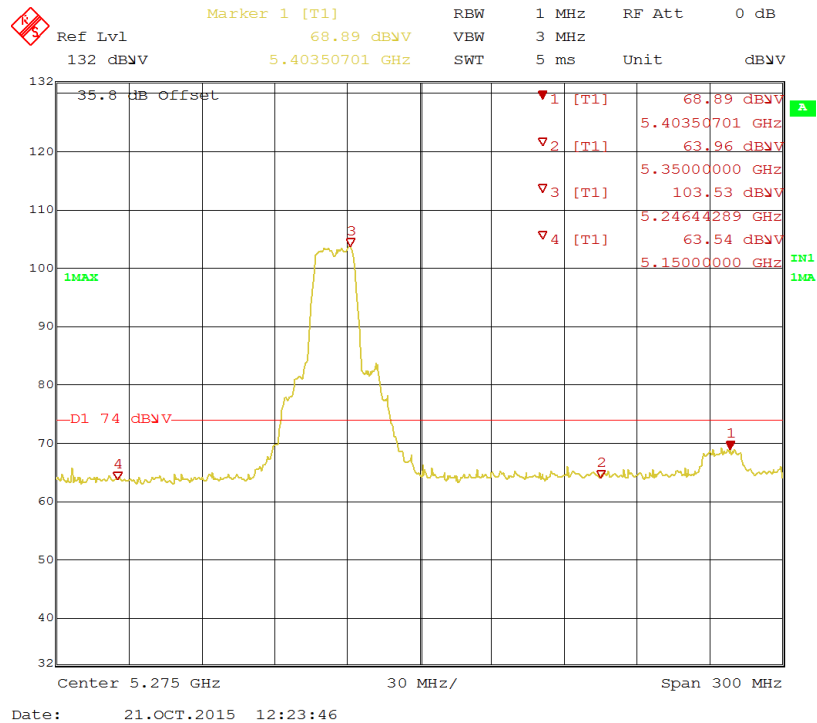
Figure 21: Radiated Emission 5350 MHz Edge for 11a 5240 MHz – Horz. (Pk)
