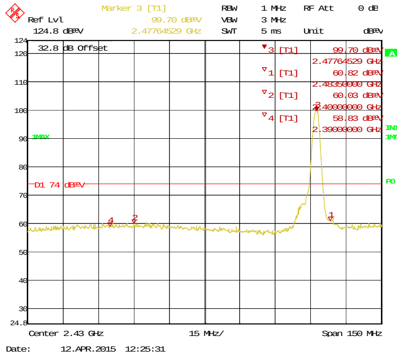
Figure 25: Bandedge-2477.35 MHz-V-Pk
