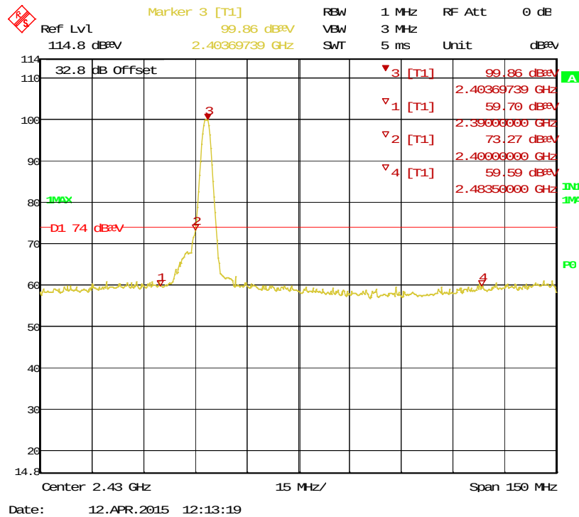
Figure 21: Bandedge-2403.35 MHz-V-pk
