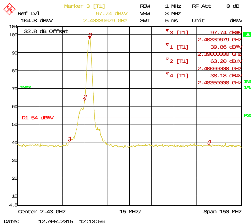
Figure 22: Bandedge-2403.35 MHz-V-Ave
