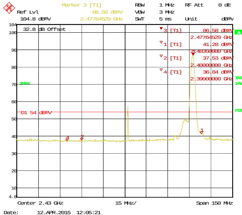
Figure 23: Bandedge-2477.35 MHz-V-Ave
