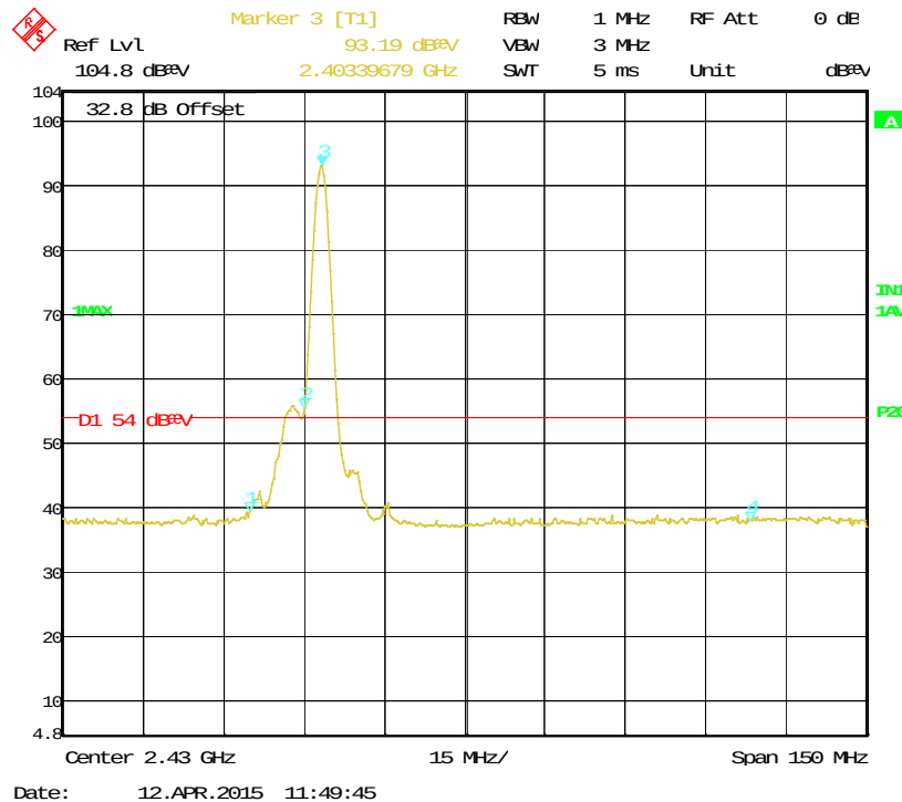
Figure 19: Bandedge-2403.35 MHz-V-Ave
