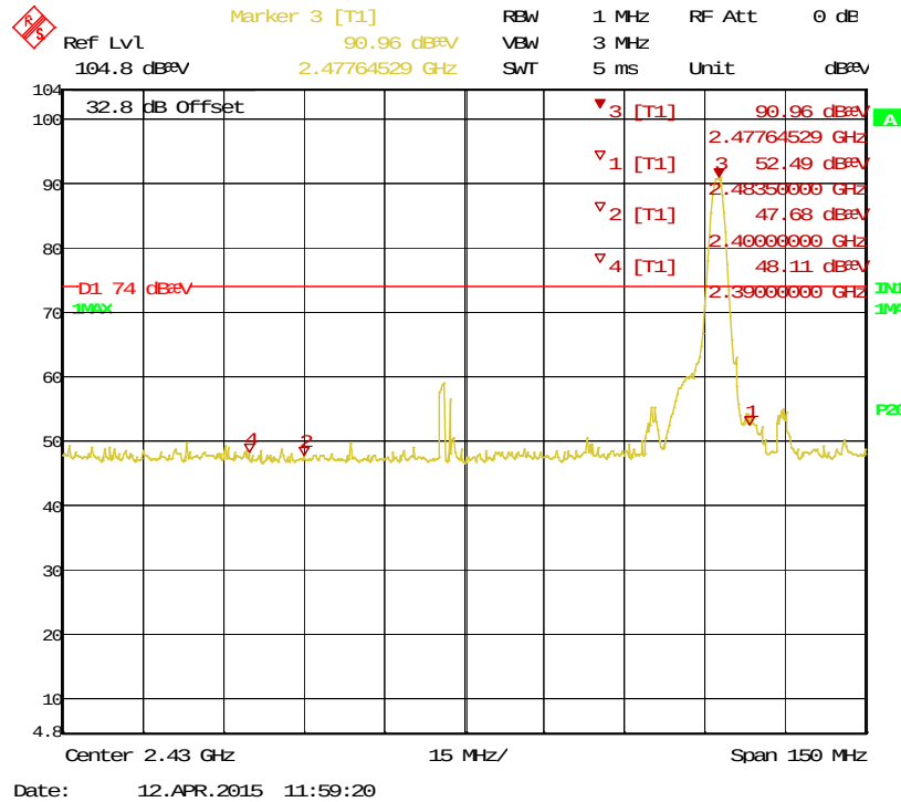
Figure 20: Bandedge-2477.35 MHz-H-Pk
