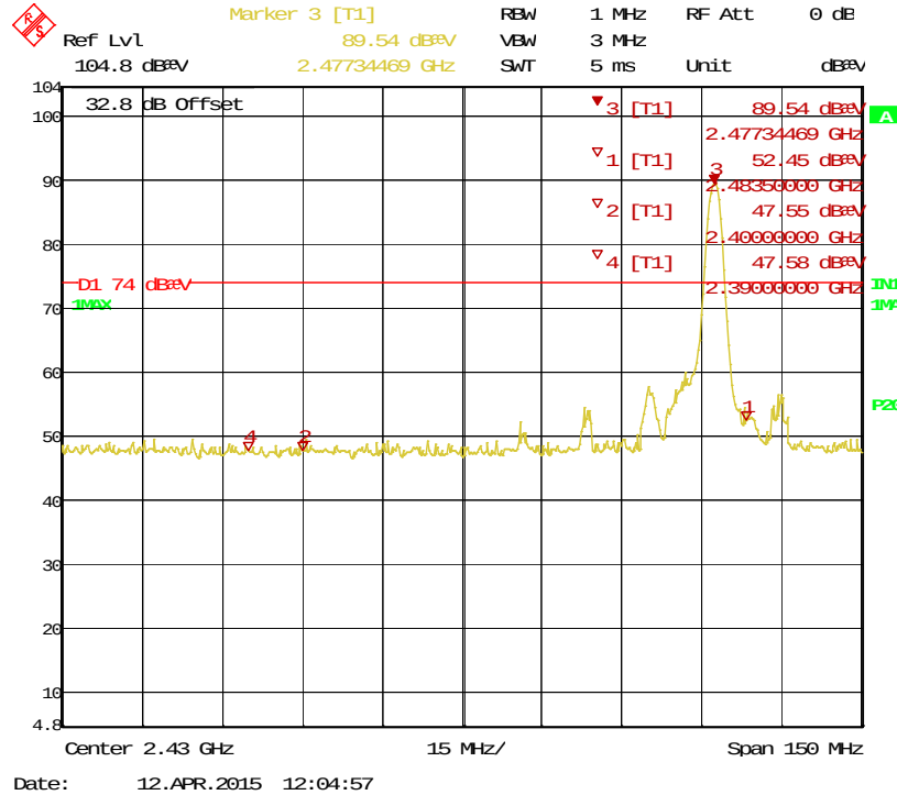
Figure 22: Bandedge-2477.35 MHz-V-Pk
