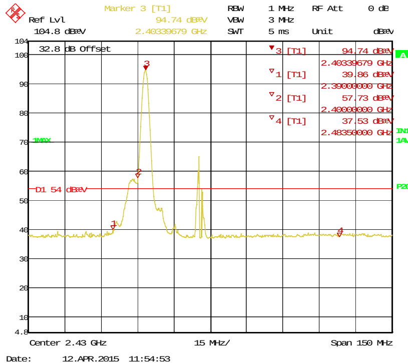
Figure 17: Bandedge-2403.35 MHz-H-Ave
