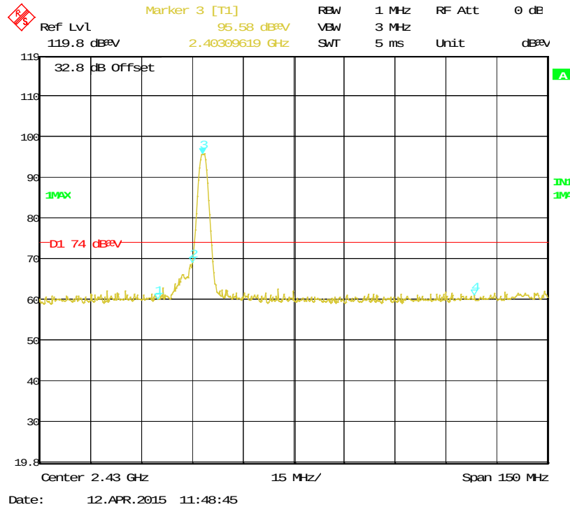
Figure 18: Bandedge-2403.35 MHz-V-pk
