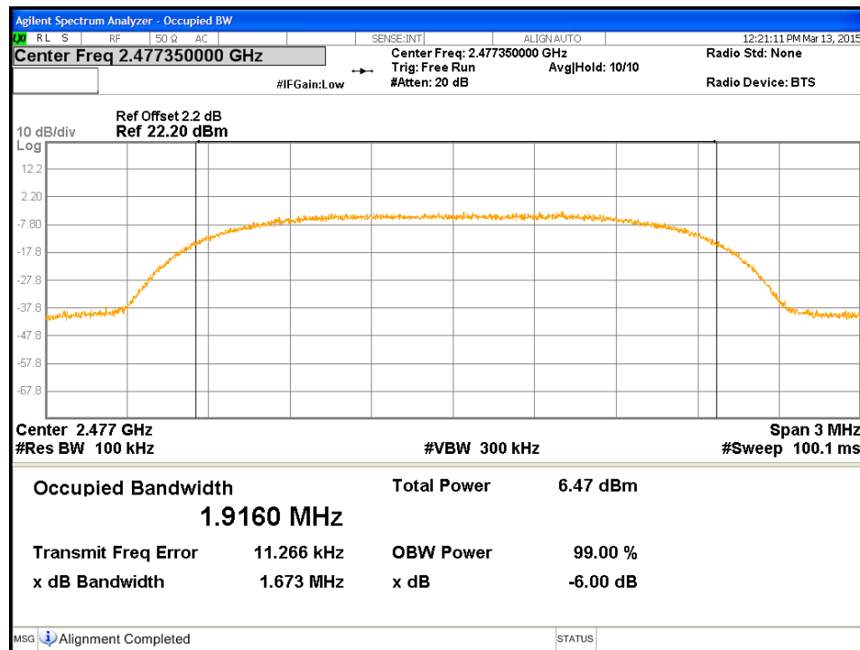
Figure 6: Bandwidth-Transmitter -2477.35MHz
