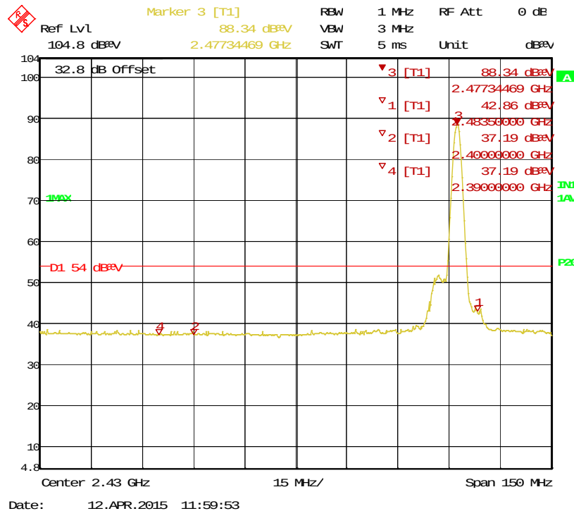
Figure 21: Bandedge-2477.35 MHz-H-Ave
