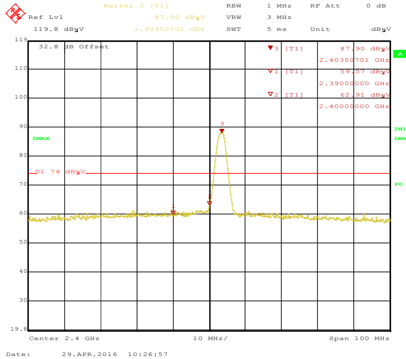
Figure 21: Bandedge-2403.35 MHz-V-Pk
