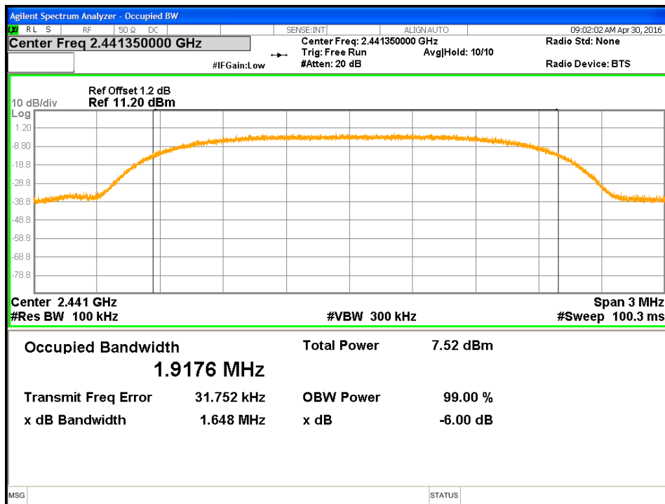
Figure 8: 99% Bandwidth-Transmitter -2441.35 MHz
