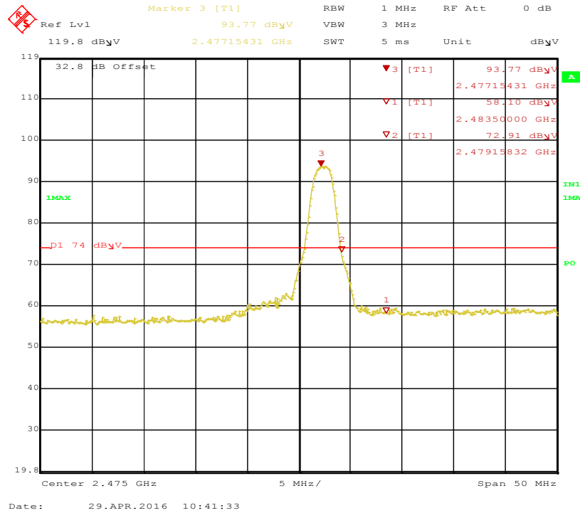
Figure 23: Bandedge-2477.35 MHz-H-Pk
