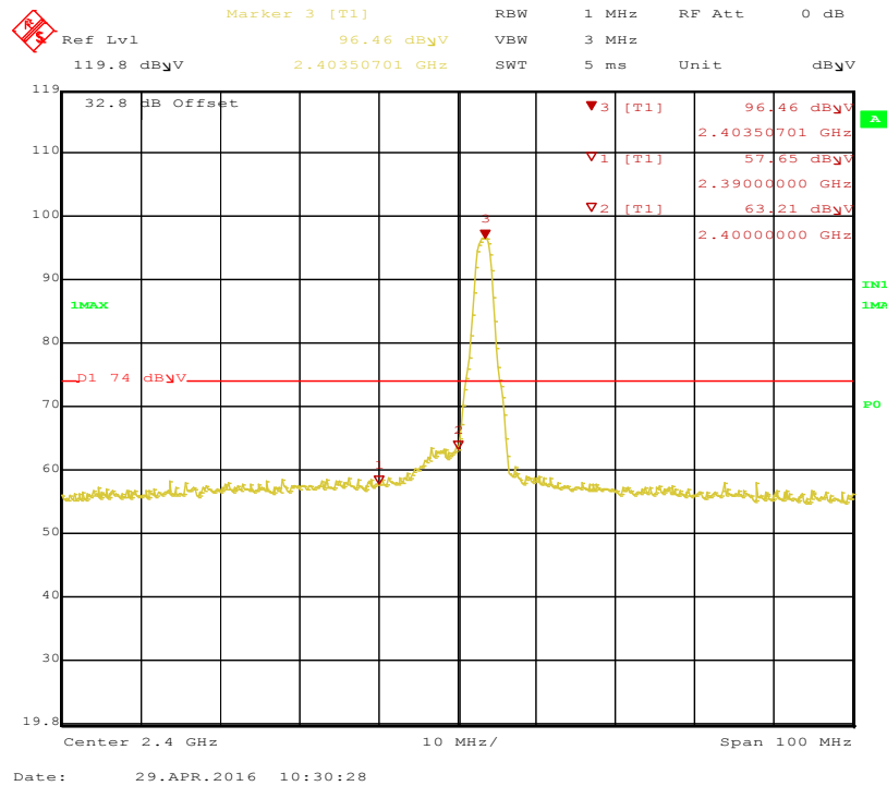
Figure 19: Bandedge-2403.35 MHz-H-Pk
