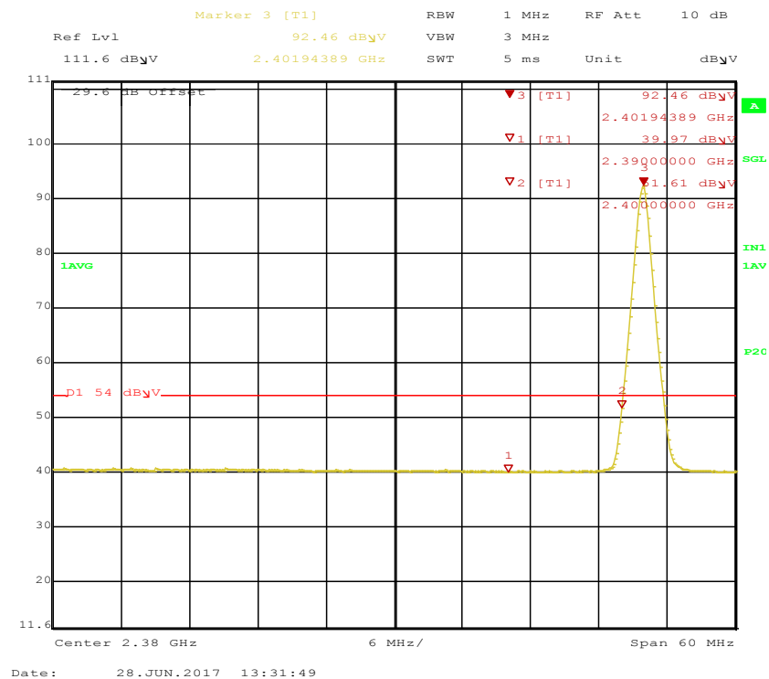
Figure 54: Radiated Emission at the Edge for BLE, 2402 MHz – Horizontal (Avg)
