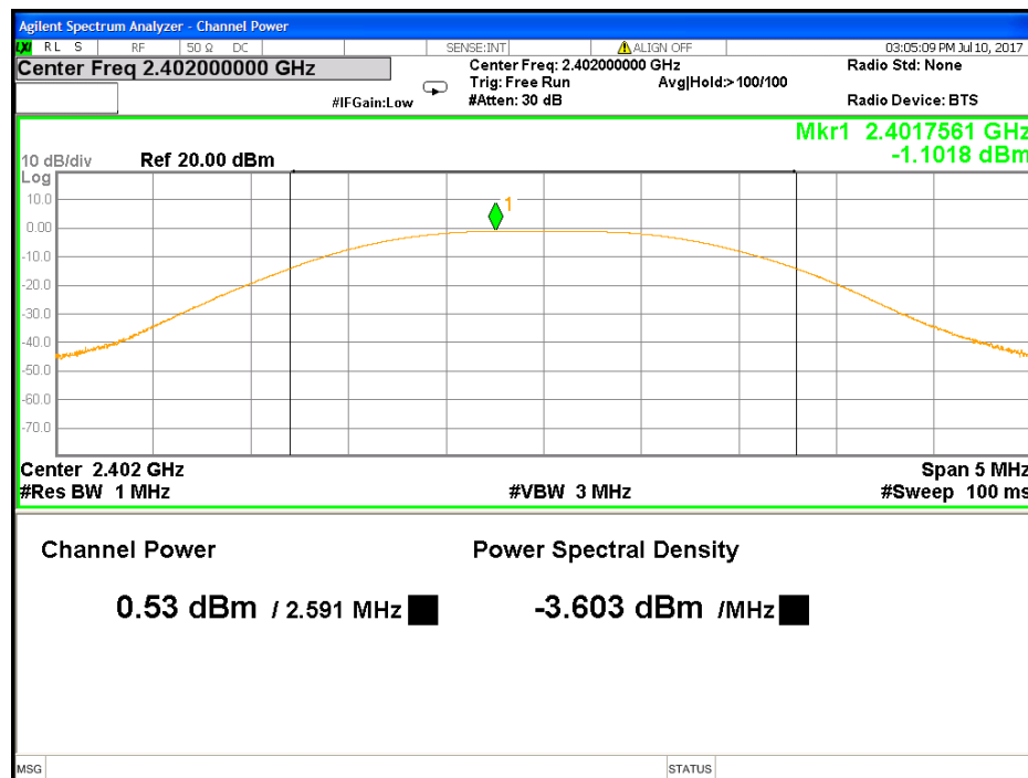
Figure 10: Maximum Transmitted Power at 2402 MHz, BLE
