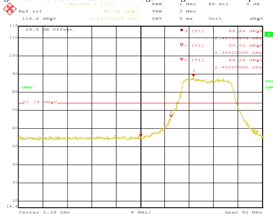
Figure 66: Radiated Emission at the Edge for 11g-2412 MHz-6 Mbps-V-Ave
