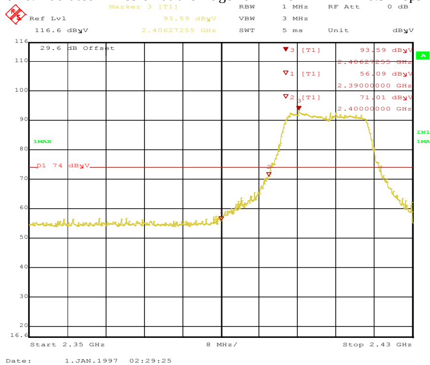
Figure 77: Radiated Emission at the Edge for HT20-2412 MHz-6.5 Mbps-H-Pk
