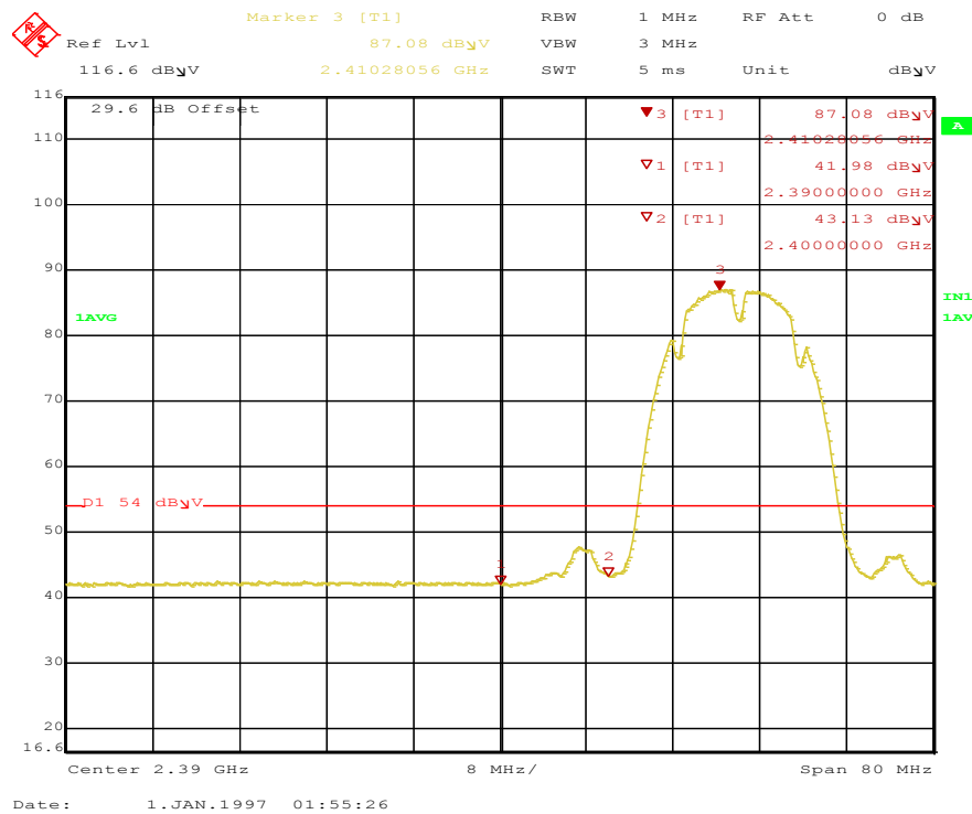
Figure 60: Radiated Emission at the Edge for 11b-2412 MHz-1 Mbps-H-Ave
