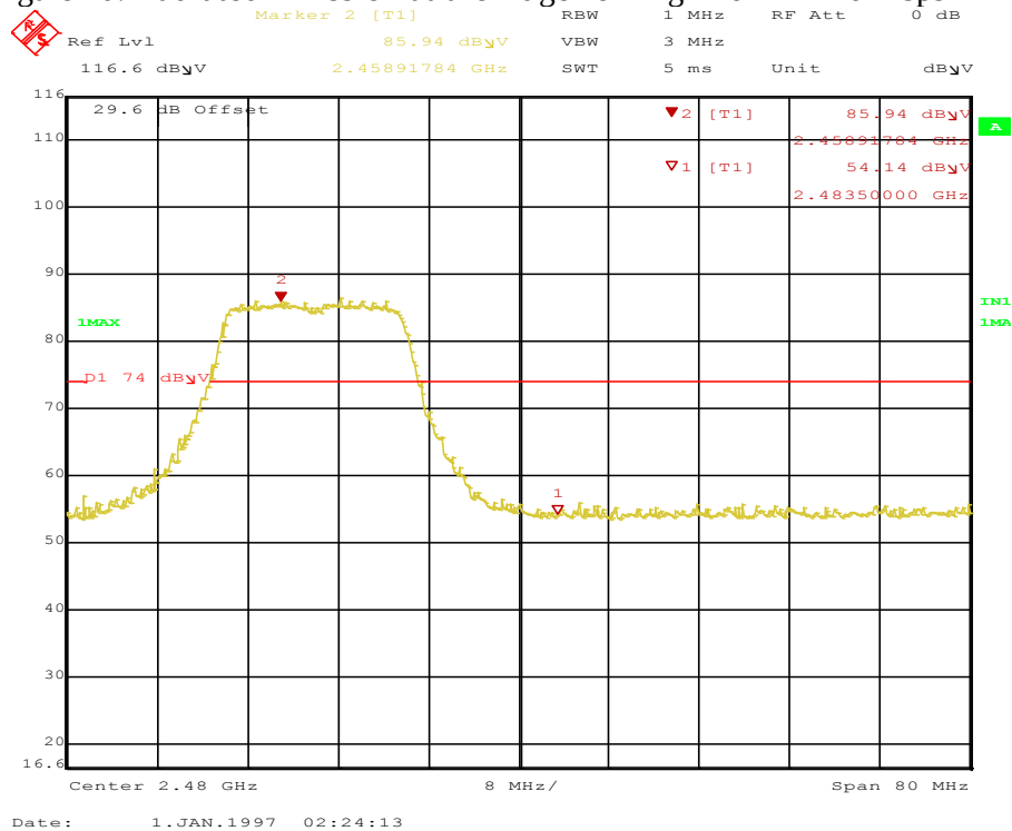
Figure 71: Radiated Emission at the Edge for 11g-2462 MHz-6 Mbps-H-Pk
