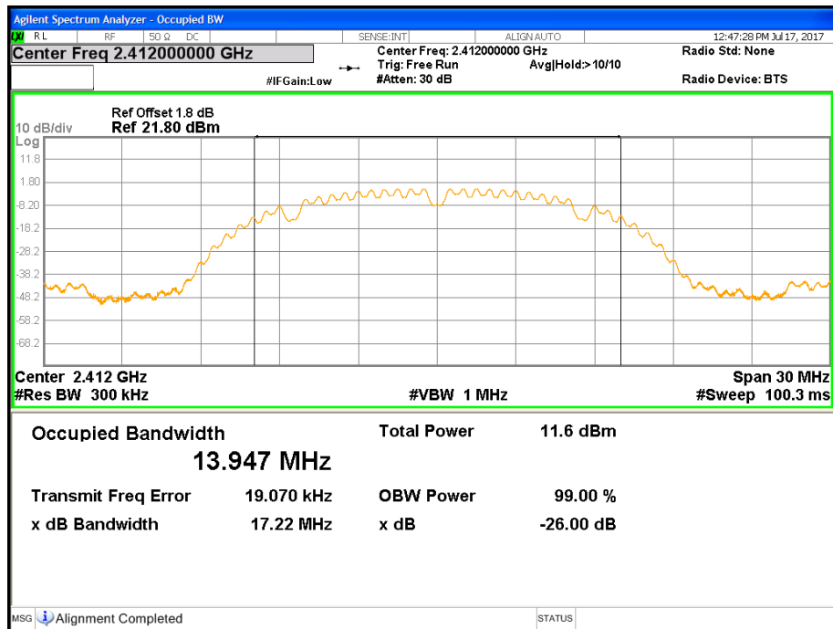
Figure 16: 99% Bandwidth-802.11b-2412 MHz
