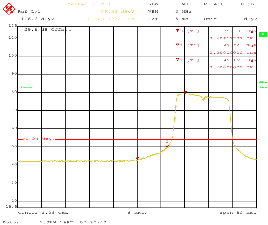
Figure 74: Radiated Emission at the Edge for HT20-2412 MHz-6.5 Mbps-V-Ave
