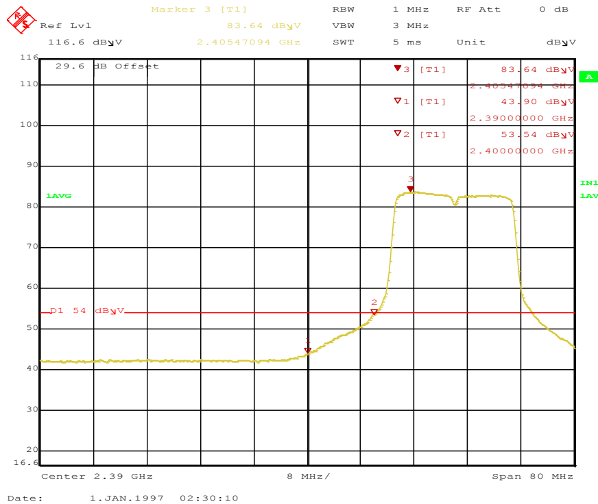
Figure 76: Radiated Emission at the Edge for HT20-2412 MHz-6.5 Mbps-H-Ave
