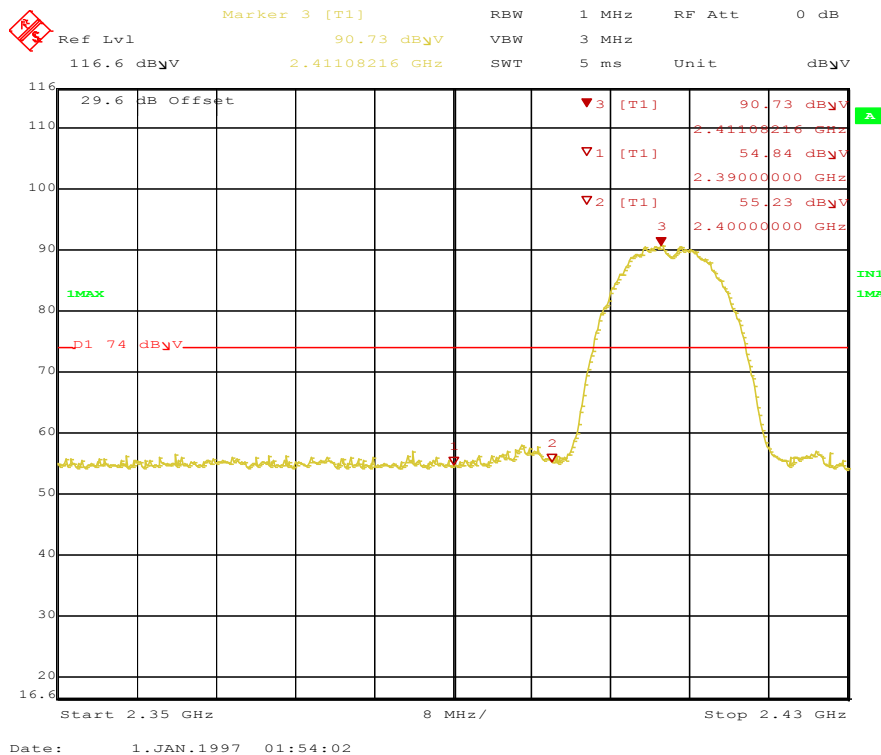
Figure 61: Radiated Emission at the Edge for 11b-2412 MHz-1 Mbps-H-Pk
