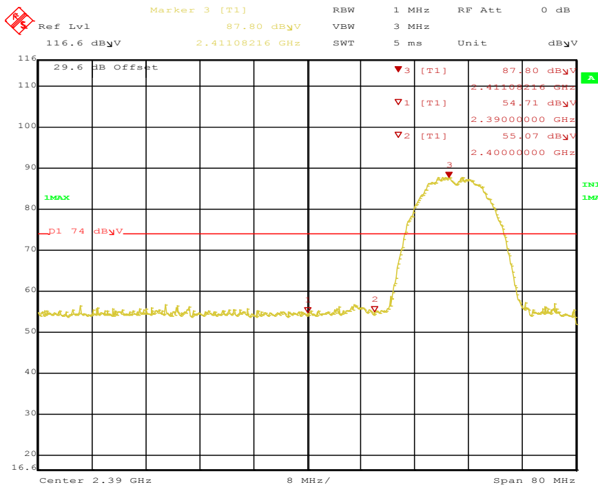
Figure 59: Radiated Emission at the Edge for 11b-2412 MHz-1 Mbps-V-Pk
