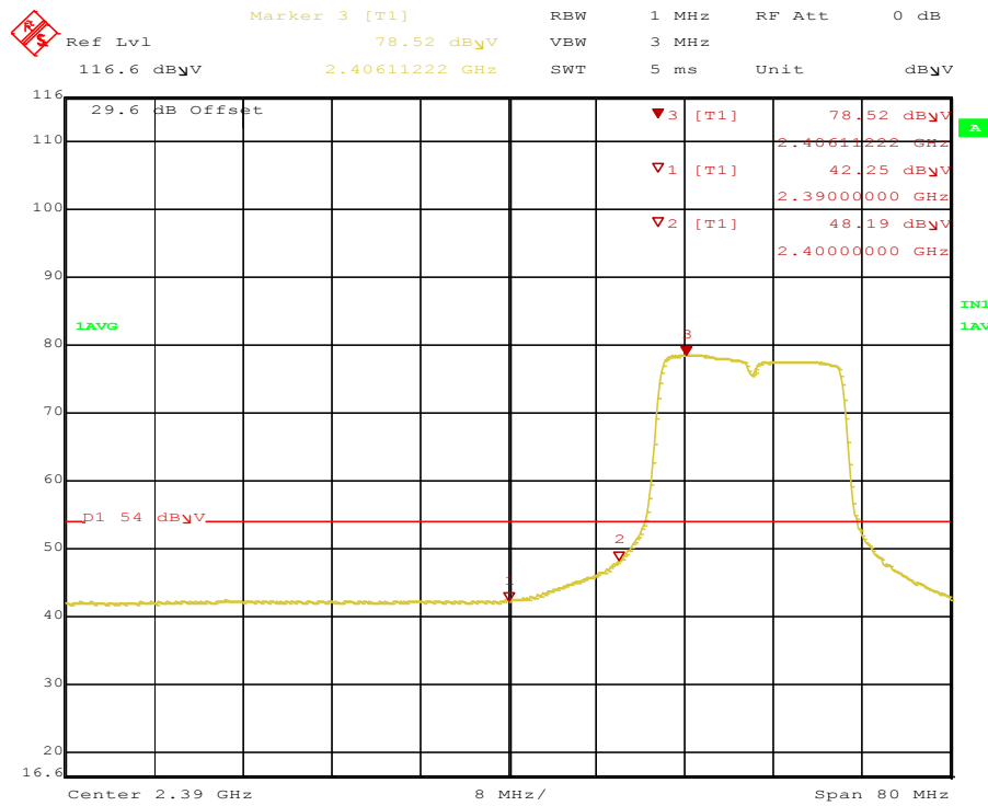
Figure 66: Radiated Emission at the Edge for 11g-2412 MHz-6 Mbps-V-Ave
