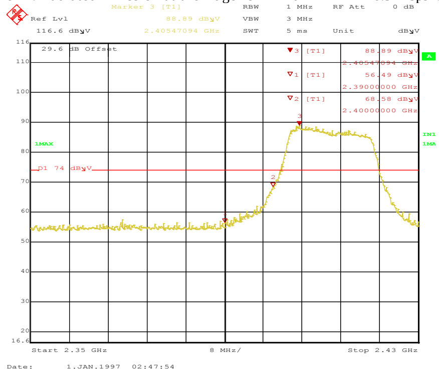
Figure 75: Radiated Emission at the Edge for HT20-2412 MHz-6.5 Mbps-V-Pk
