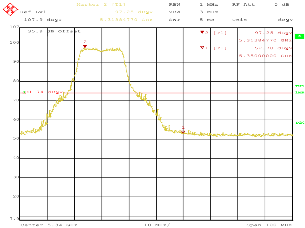
Figure 133: Radiated Emission 5350.0 MHz Edge for 11a 5320 MHz – Horz. (Pk)
