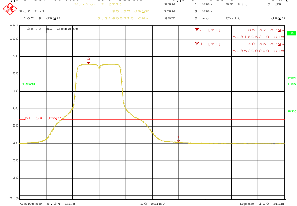
Figure 136: Radiated Emission 5350.0 MHz Edge for 11a 5320 MHz – Vert. (Ave)
