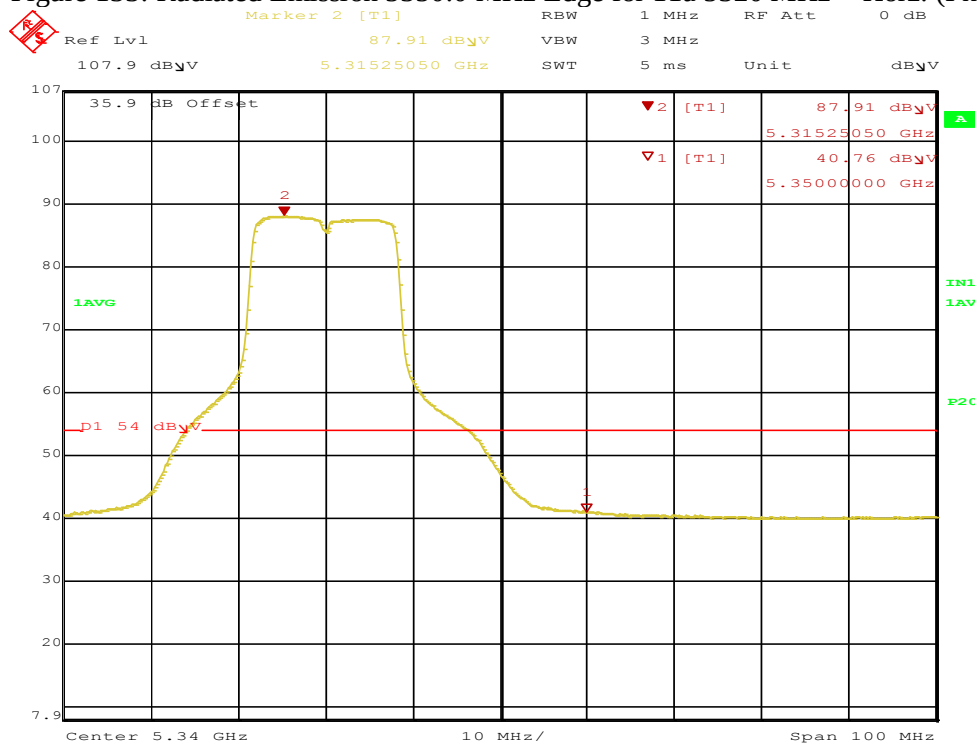
Figure 133: Radiated Emission 5350.0 MHz Edge for 11a 5320 MHz – Horz. (Pk)
