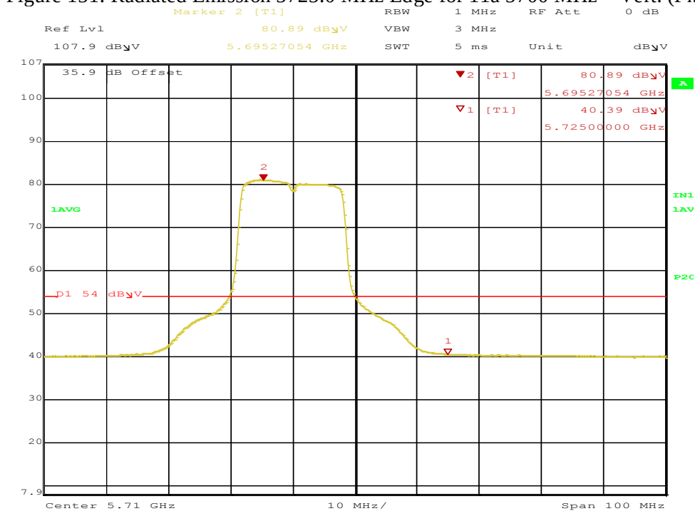
Figure 152: Radiated Emission 5725.0 MHz Edge for 11a 5700 MHz – Vert. (Ave)
