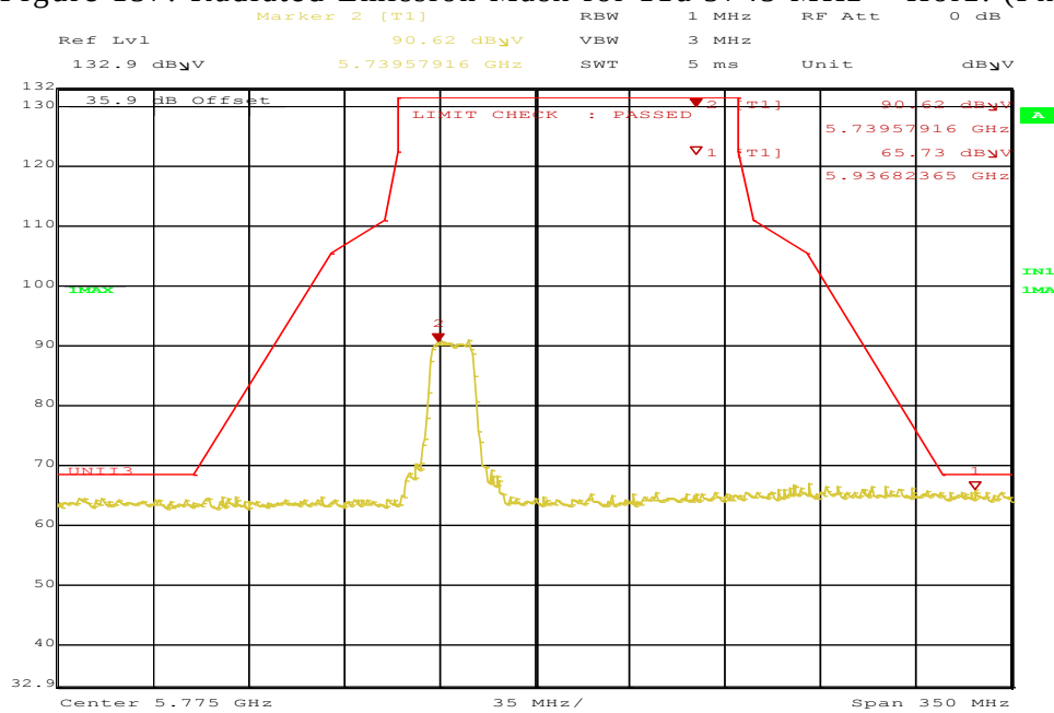
Figure 158: Radiated Emission Mask for 11a 5745 MHz – Vert (Pk)
