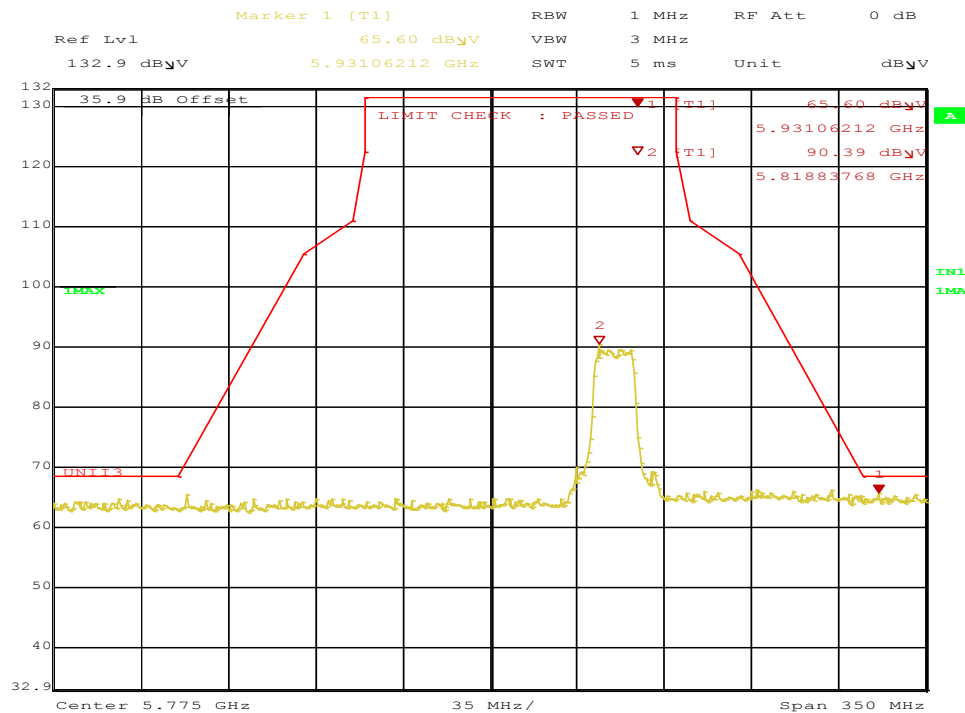
Figure 159: Radiated Emission Mask for 11a 5825 MHz – Horz. (Pk)
