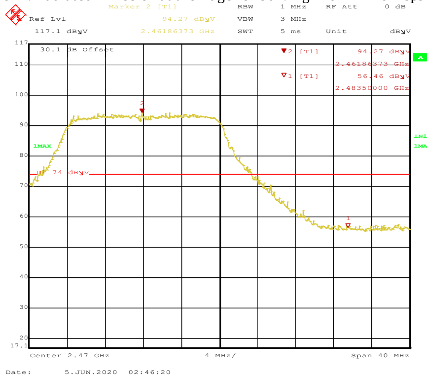
Figure 73: Radiated Emission at the Edge for 802.11g-2462 MHz-6 Mbps-V-Pk
