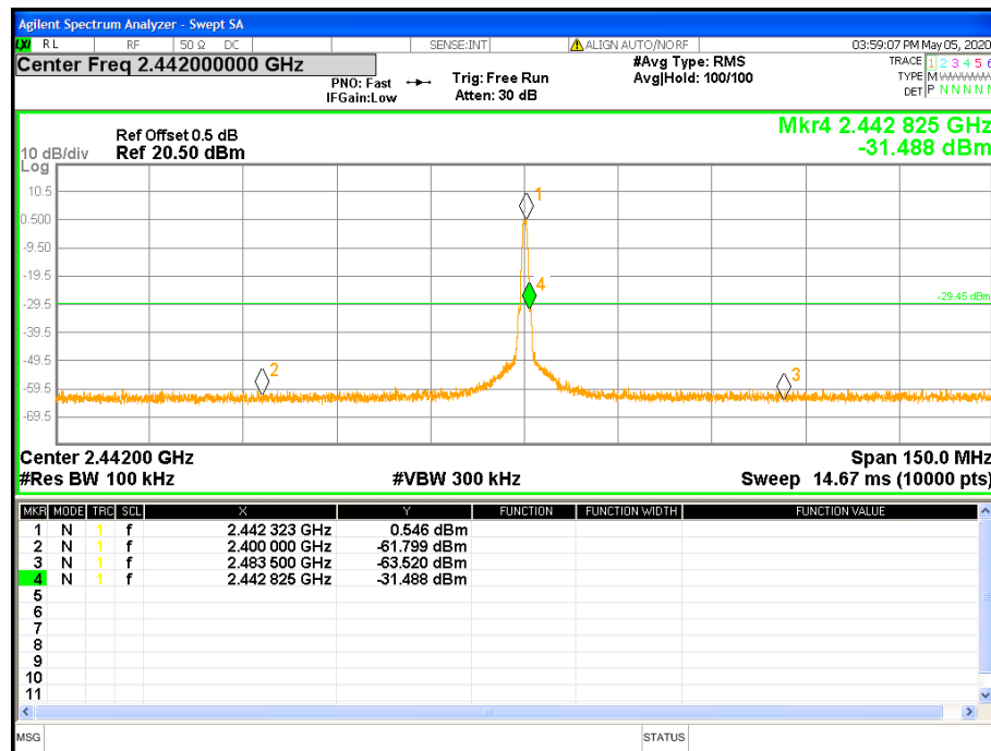
Figure 16: Conducted Band Edge at 2442 MHz-Transmitter
