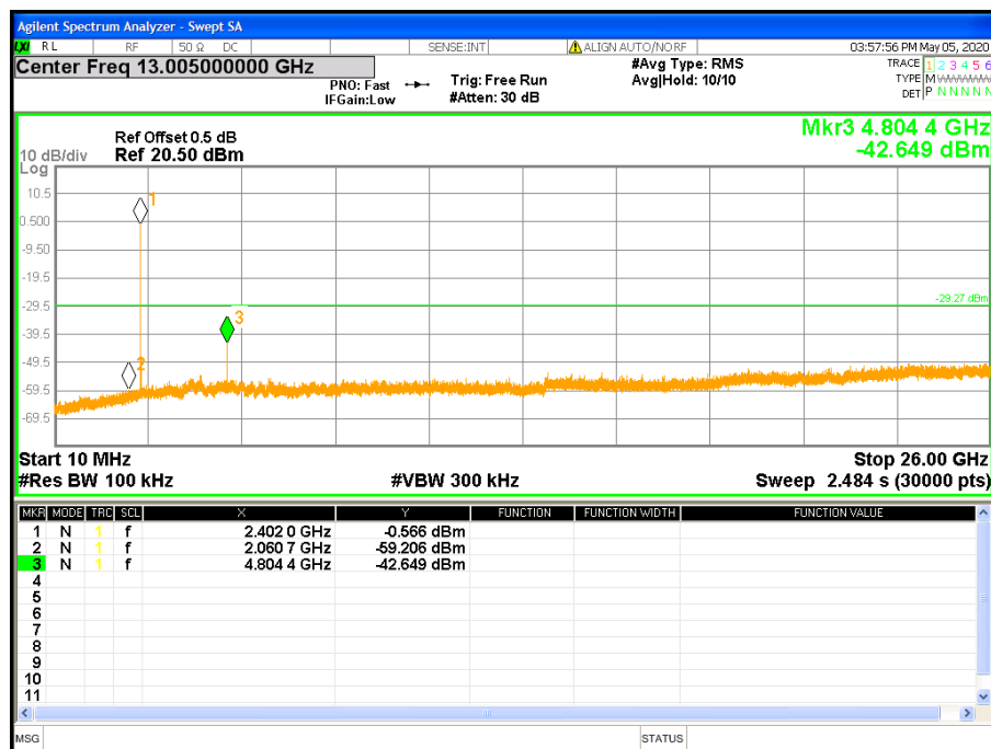
Figure 15: Out of band Emission at 2402 MHz-Transmitter
