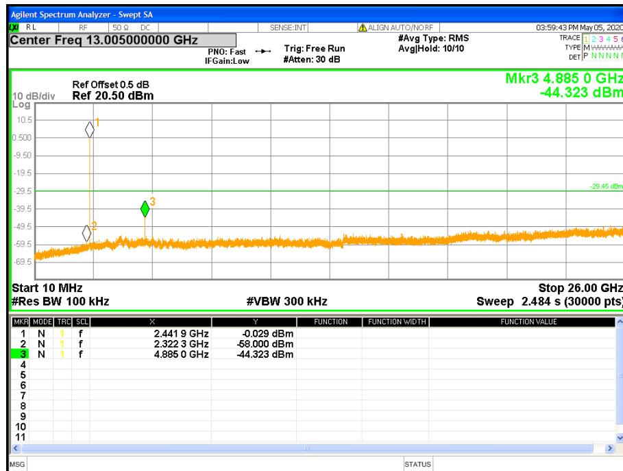
Figure 17: Out of band Emission at 2442 MHz-Transmitter
