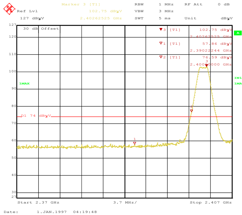
Figure 24: Band-edge-2402 MHz-H-Pk
