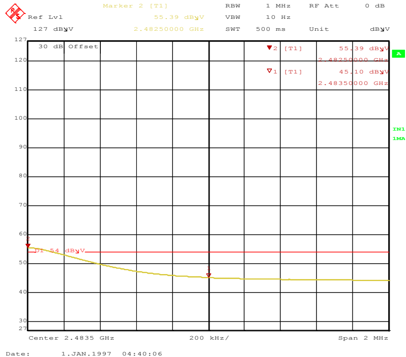
Figure 31: Band-edge-2480 MHz-V-Ave-2 MHz Span
