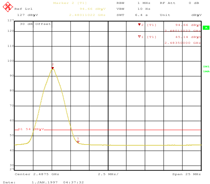
Figure 29: Band-edge-2480 MHz-V-Ave
