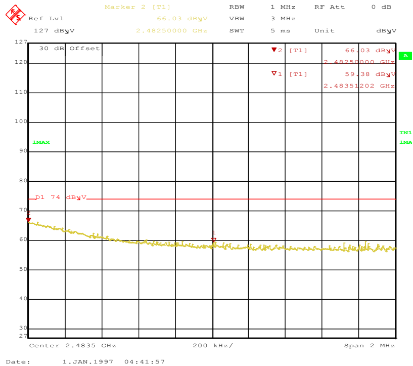
Figure 30: Band-edge-2480 MHz-V-Pk-2 MHz Span
