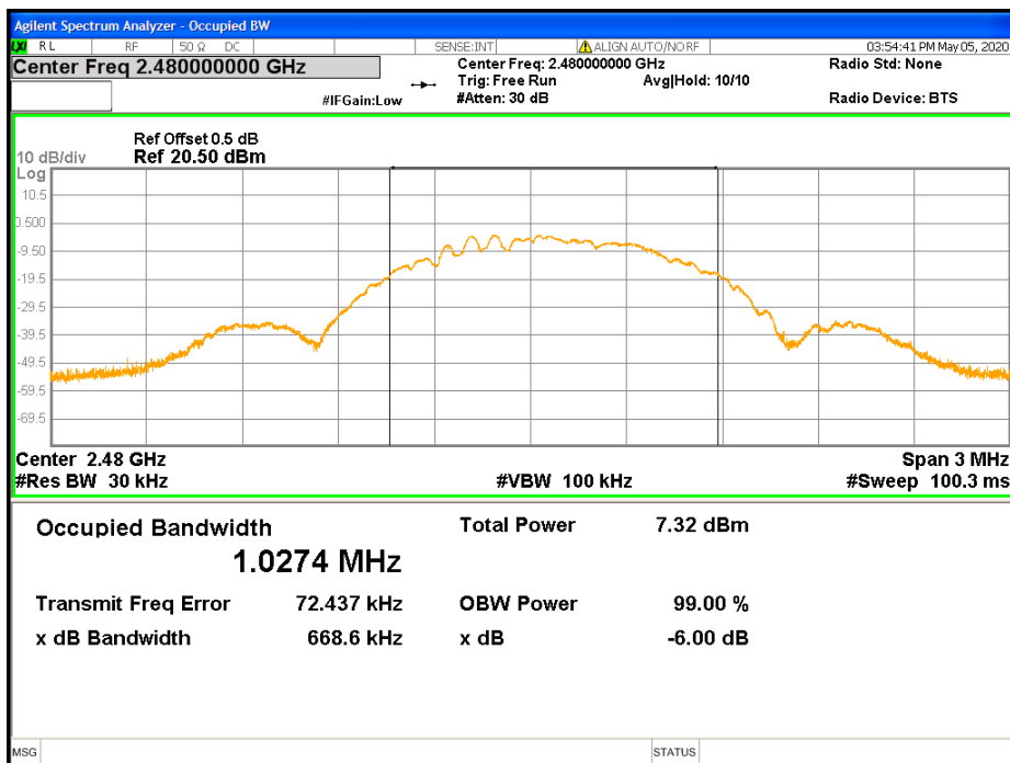
Figure 10: 99% Bandwidth-Transmitter -2480 MHz
