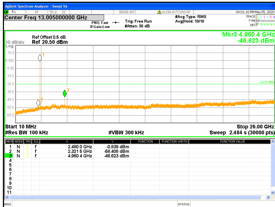
Figure 19: Out of band Emission at 2480 MHz-Transmitter
