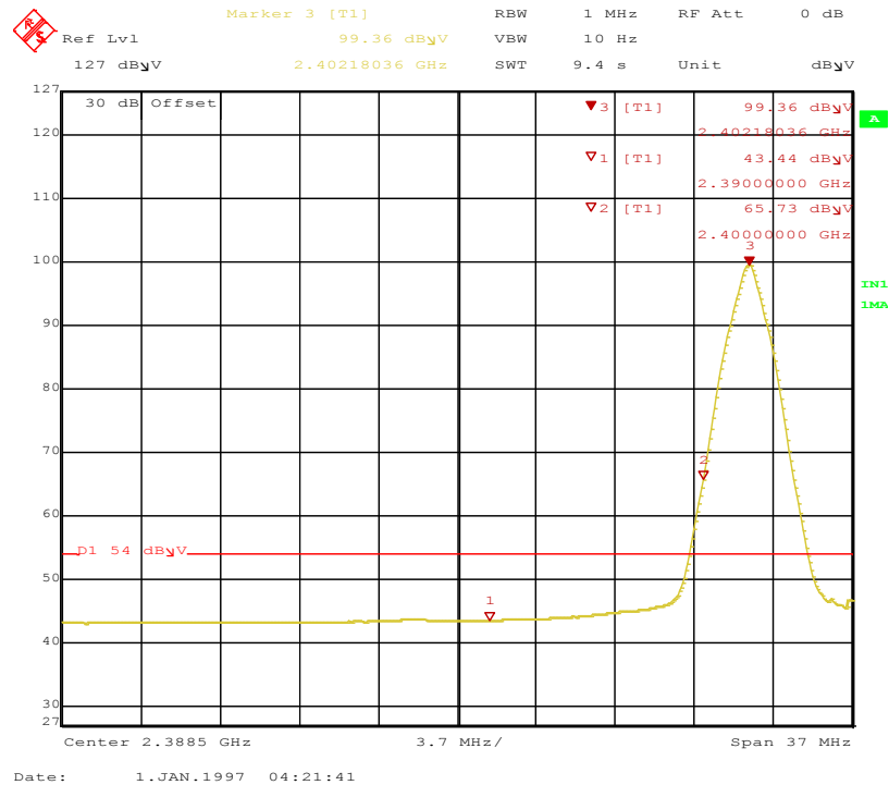
Figure 25: Band-edge-2402 MHz-H-Ave
