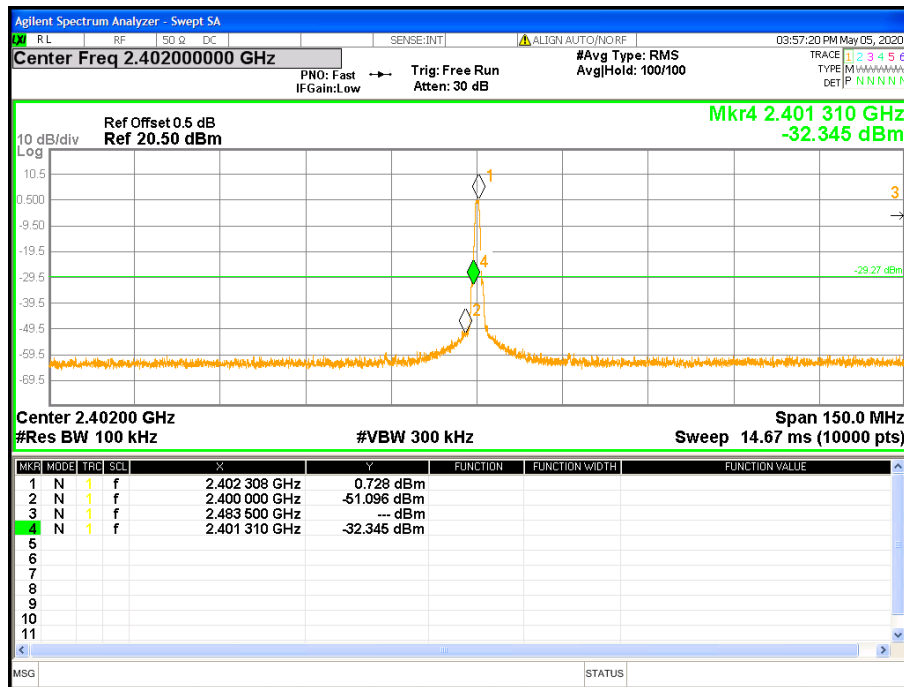
Figure 14: Conducted Band Edge at 2402 MHz-Transmitter
