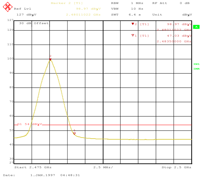
Figure 33: Band-edge-2480 MHz-H-Ave
