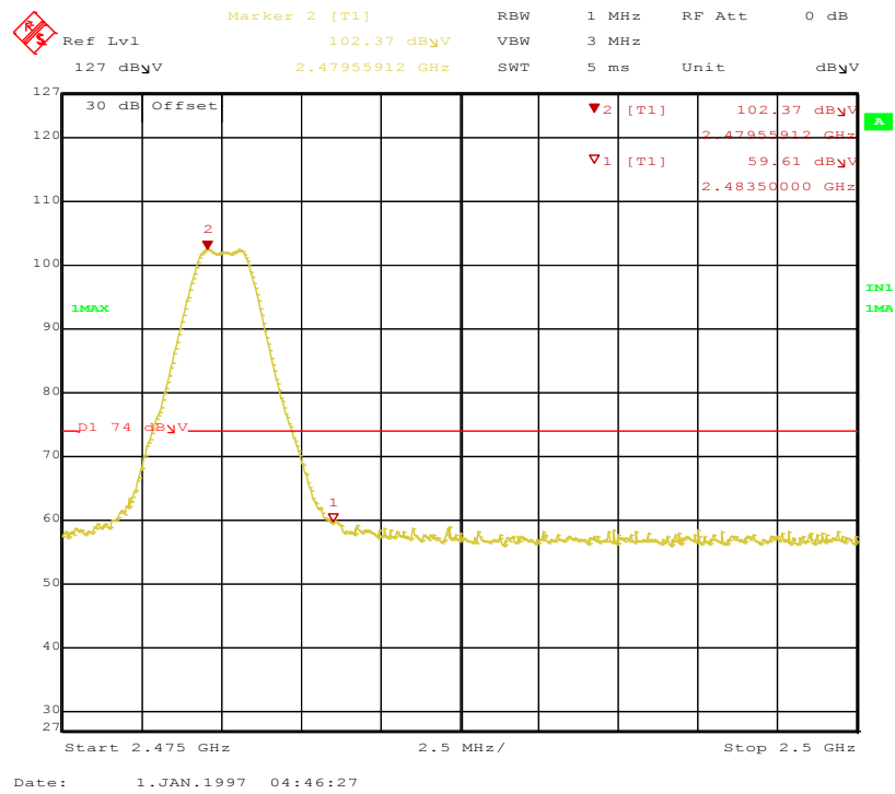
Figure 32: Band-edge-2480 MHz-H-Pk
