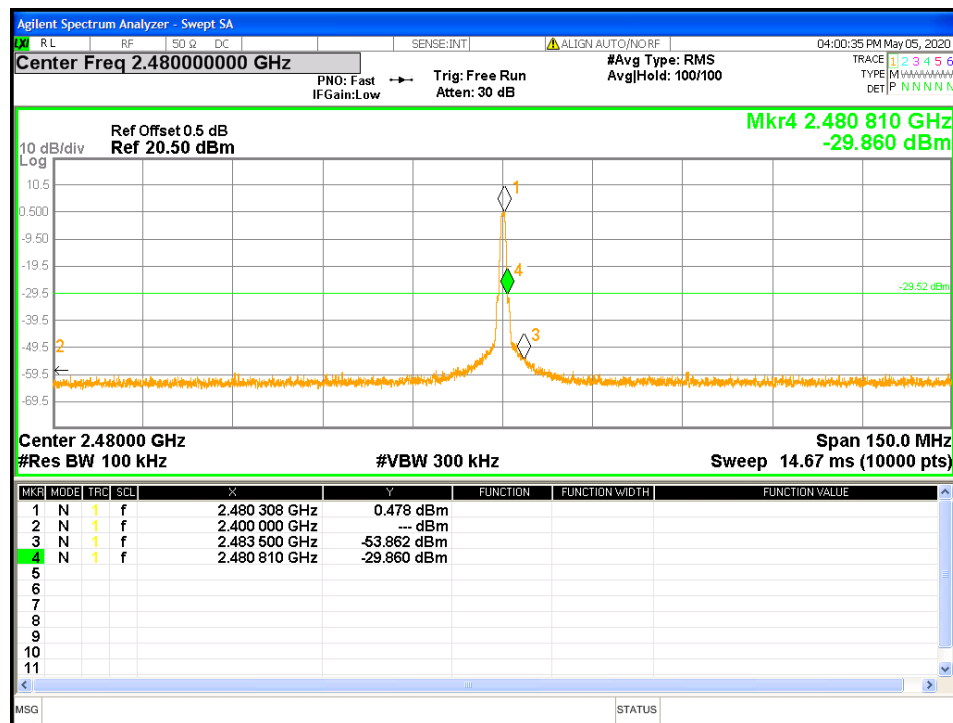
Figure 18: Conducted Band Edge at 2480 MHz-Transmitter
