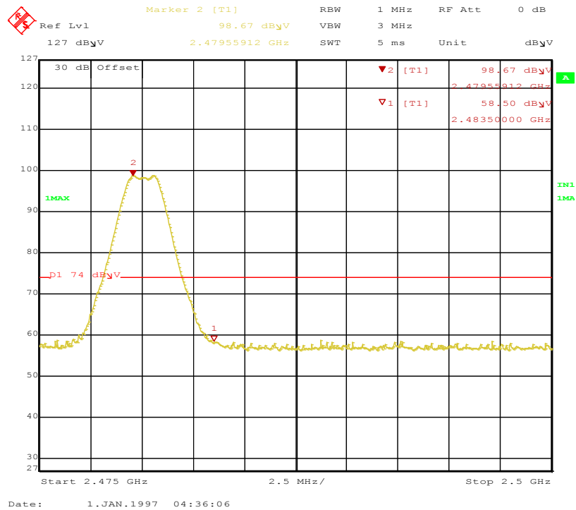
Figure 28: Band-edge-2480 MHz-V-Pk
