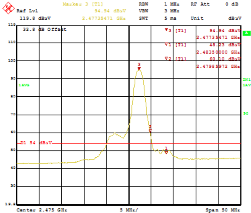
Figure 25: Bandedge-2477.35 MHz-H-Ave
