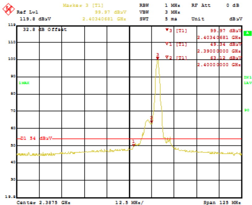
Figure 23: Bandedge-2403.35 MHz-V-Ave
