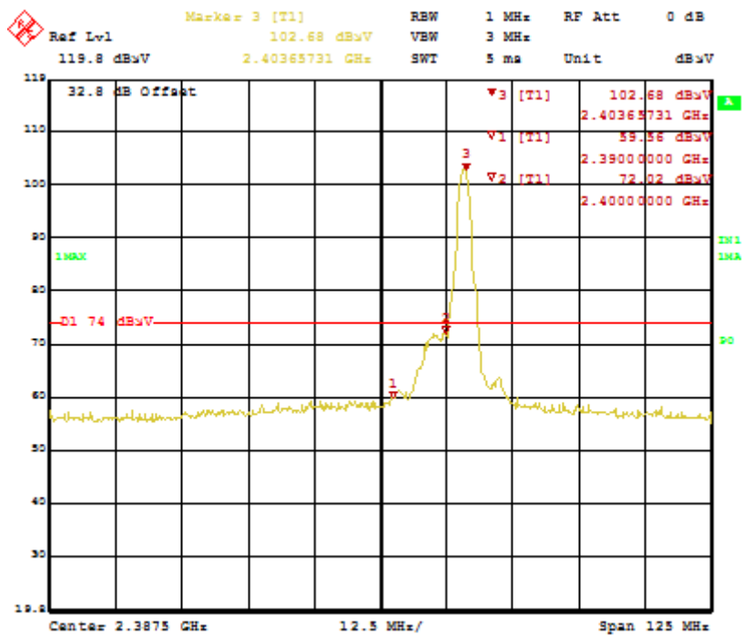
Figure 22: Bandedge-2403.35 MHz-V-Pk
