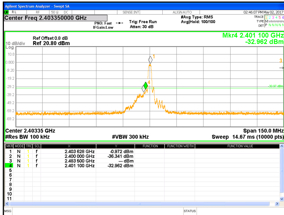
Figure 14: Conducted Band Edge at 2403.35 MHz-Transmitter
