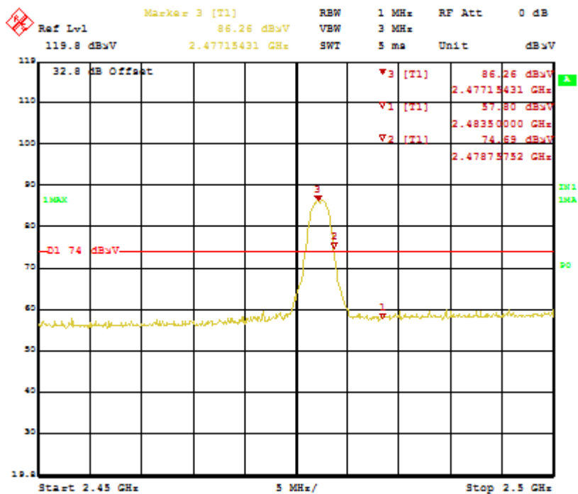
Figure 26: Bandedge-2477.35 MHz-V-Pk
