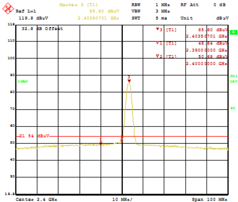
Figure 23: Bandedge-2403.35 MHz-V-Ave
