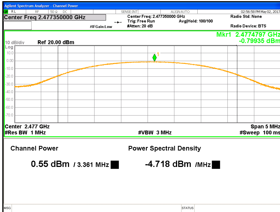
Figure 4: Maximum Conducted Output Power at 2477.35 MHz - USB Transmitter
