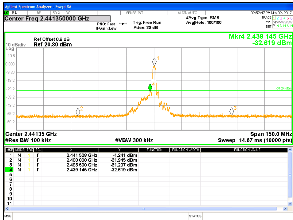
Figure 16: Conducted Band Edge-2441.35 MHz-Transmitter
