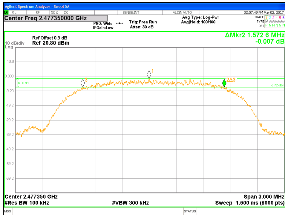
Figure 7: DTS Bandwidth-Transmitter -2477.35 MHz
