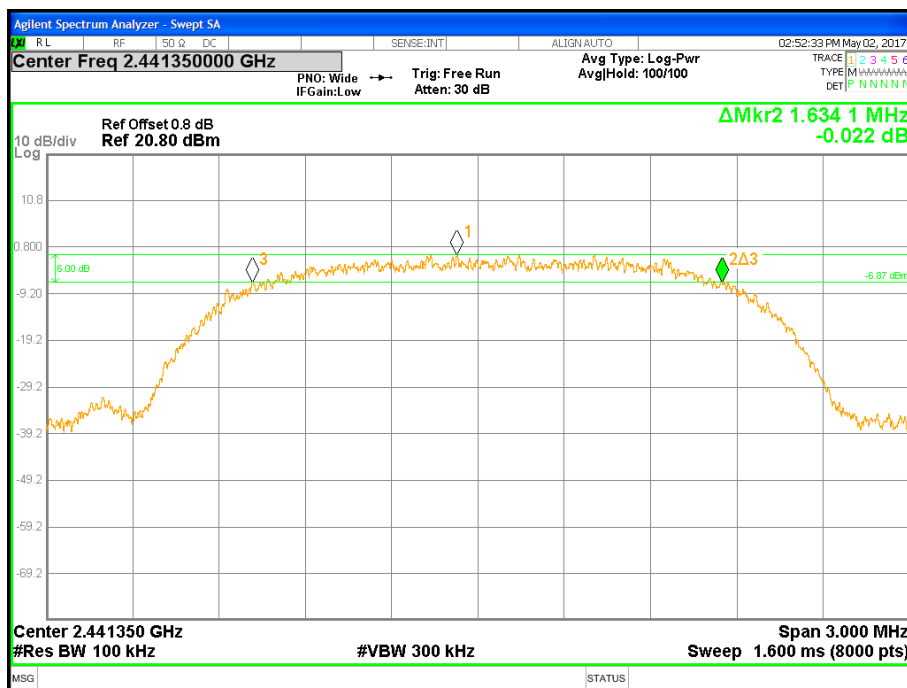
Figure 6: DTS Bandwidth-Transmitter -2441.35 MHz
