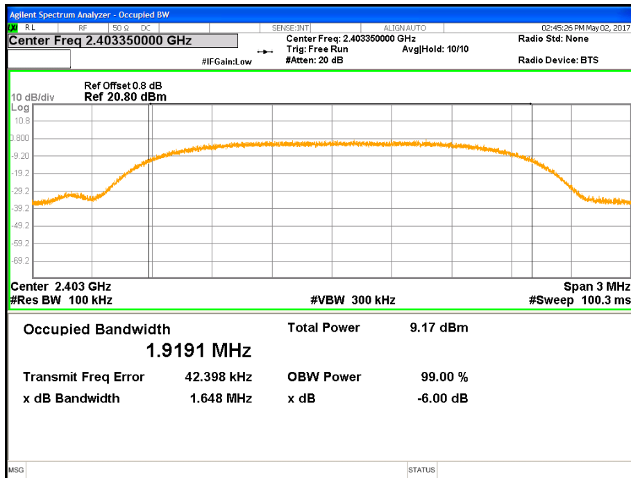
Figure 8: 99% Bandwidth-Transmitter -2403.35 MHz
