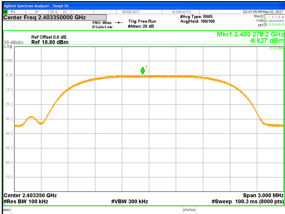
Figure 11: Maximum Power Spectral Density-2403.35 MHz-Transmitter
