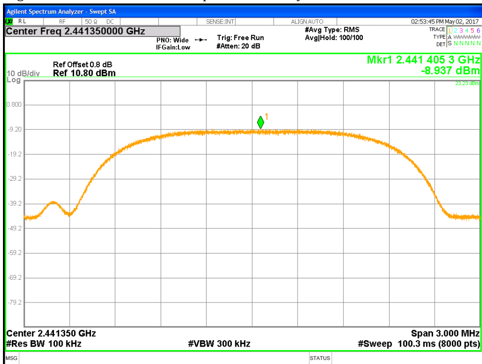
Figure 12: Maximum Power Spectral Density-2441.35 MHz-Transmitter
