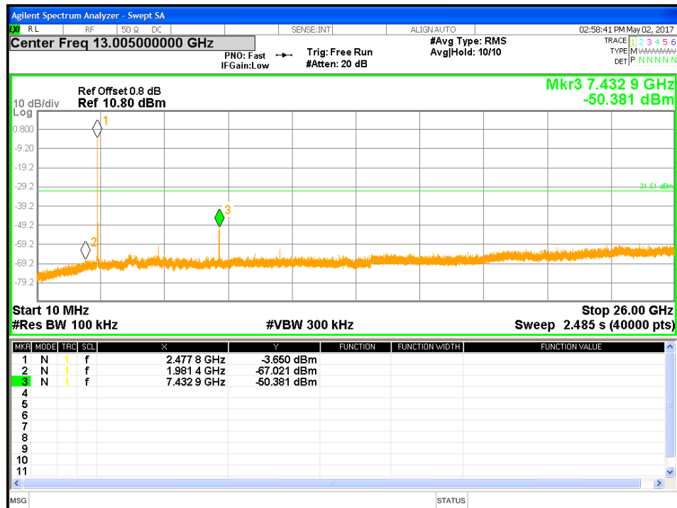
Figure 19: Out of band Emission-2477.35 MHz-Transmitter
