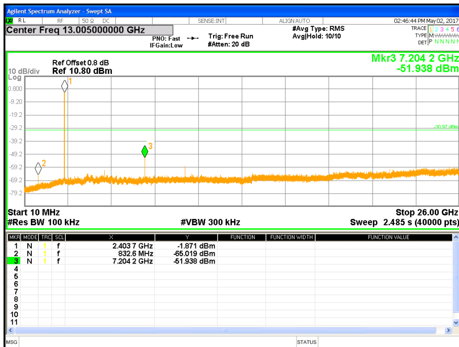
Figure 15: Out of band Emission-2403.35 MHz-Transmitter
