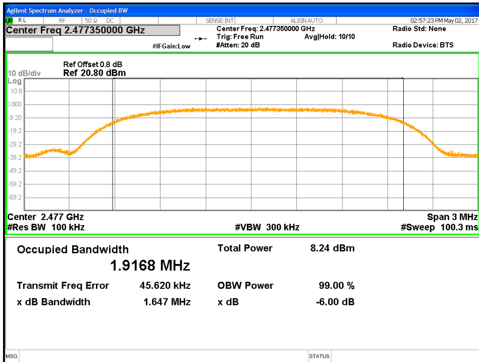
Figure 10: 99% Bandwidth-Transmitter -2477.35 MHz
