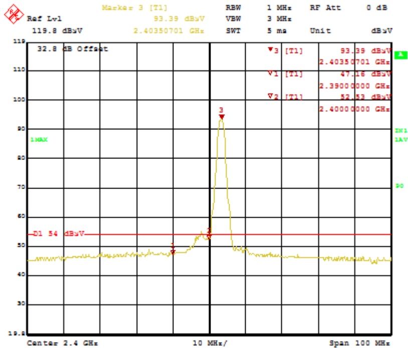
Figure 21: Bandedge-2403.35 MHz-H-Ave
