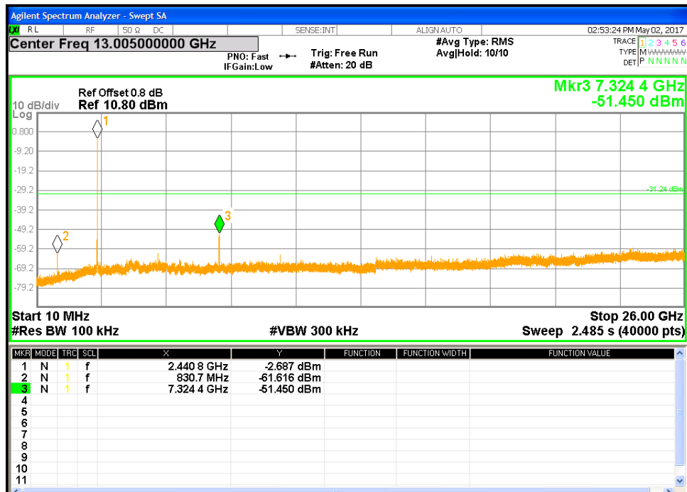
Figure 17: Out of band Emission-2441.35 MHz-Transmitter
