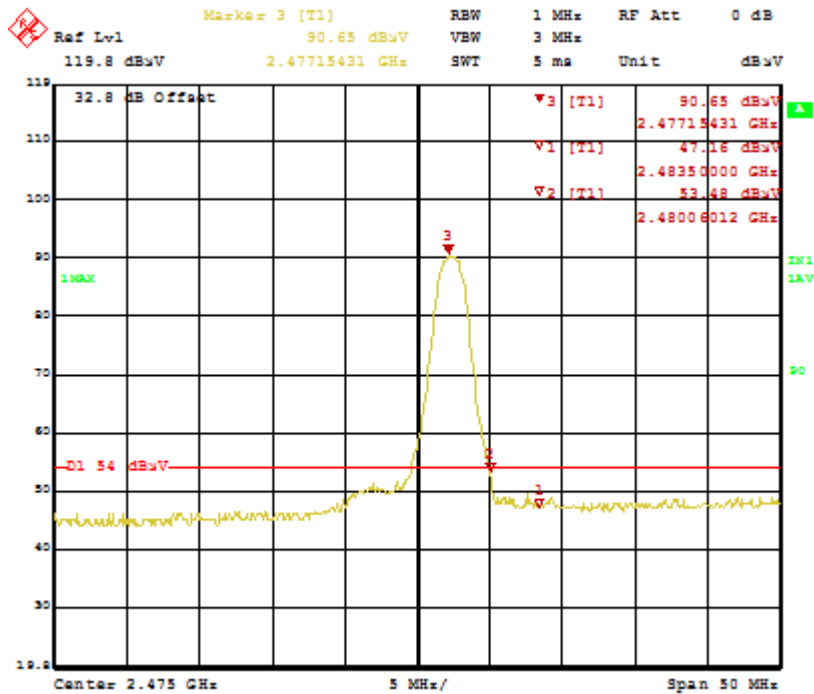
Figure 25: Bandedge-2477.35 MHz-H-Ave
