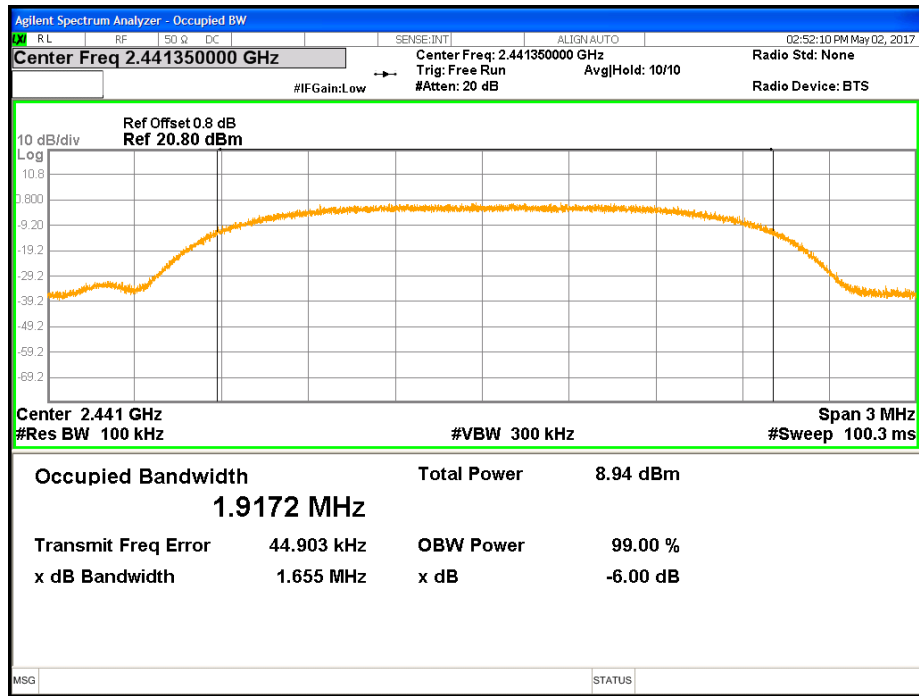
Figure 9: 99% Bandwidth-Transmitter -2441.35 MHz
