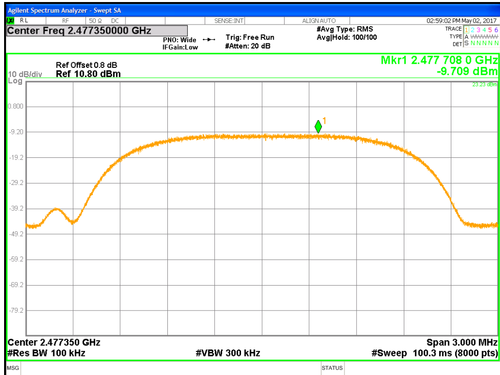
Figure 13: Maximum Power Spectral Density-2477.35 MHz-Transmitter
