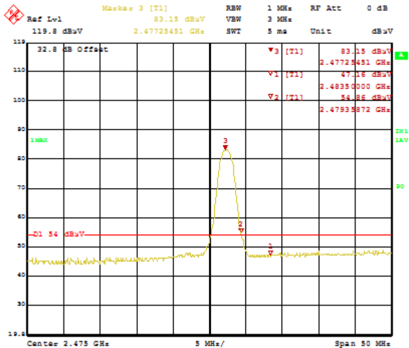
Figure 27: Bandedge-2477.35 MHz-V-Ave
