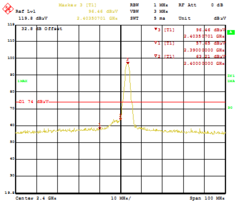
Figure 20: Bandedge-2403.35 MHz-H-Pk
