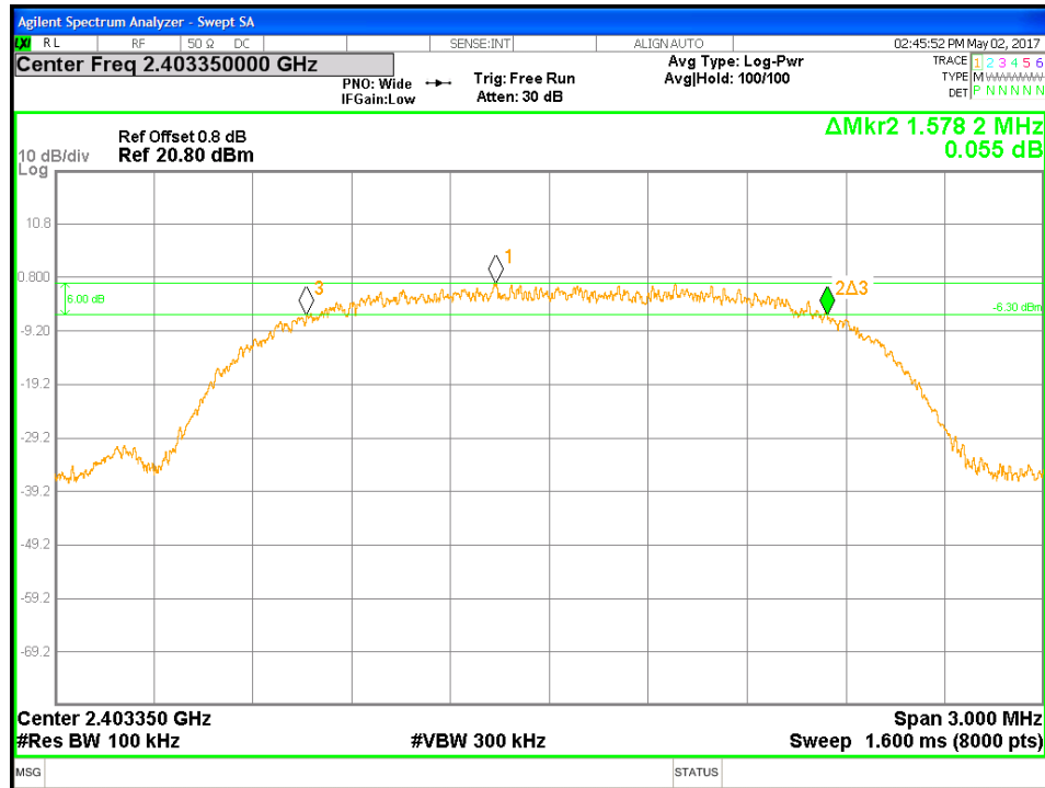
Figure 5: DTS Bandwidth-Transmitter -2403.35 MHz
