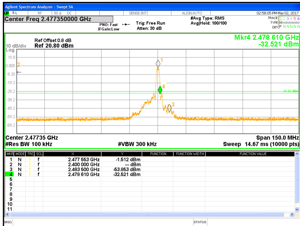
Figure 18: Conducted Band Edge-2477.35 MHz-Transmitter
