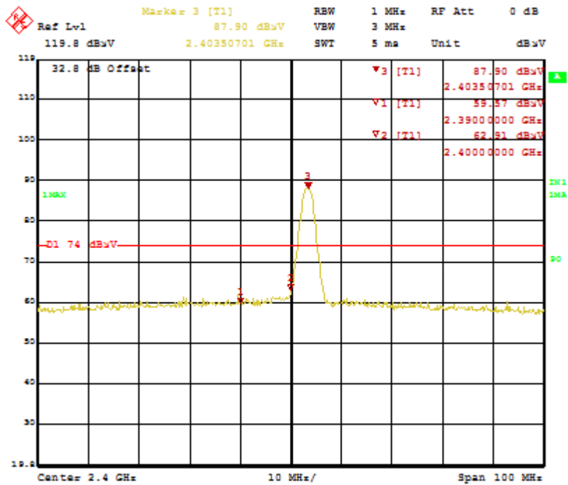
Figure 22: Bandedge-2403.35 MHz-V-Pk
