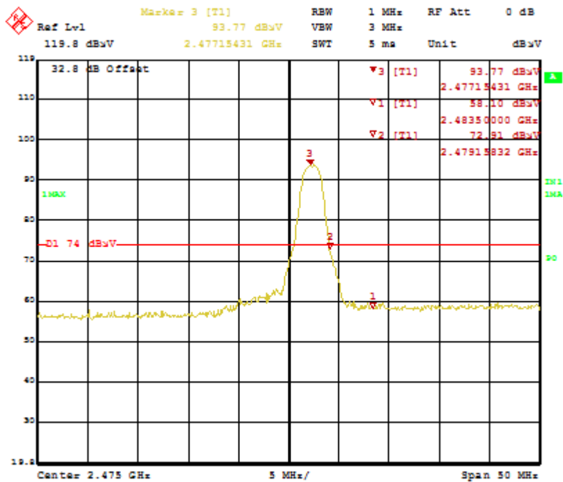
Figure 24: Bandedge-2477.35 MHz-H-Pk
