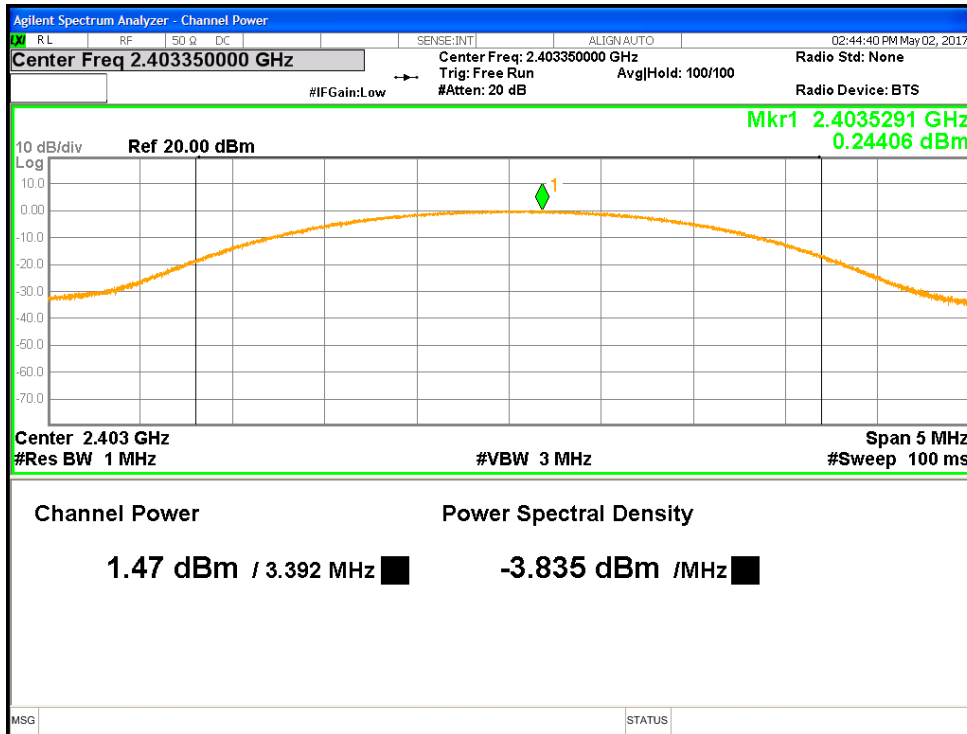
Figure 2: Maximum Transmitted Power, 2403.35 MHz- USB Transmitter
