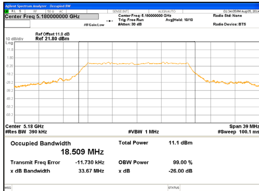
Figure 4: Occupied Bandwidth-5180 MHz-11a-6Mbps
