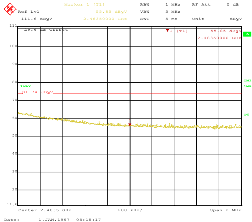
Figure 59: Radiated Emission at the Edge at 2DH1 - 2480 MHz – 2 MHz Span – Horz. (Pk)
