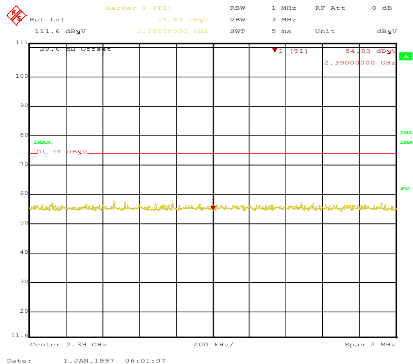
Figure 83: Radiated Emission at the Edge for BLE, 2402 MHz – 2 MHz Span –Vertical (Pk)
