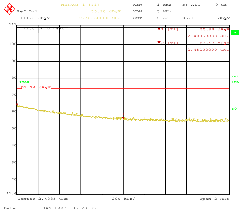
Figure 63: Radiated Emission at the Edge at 2DH1 - 2480 MHz – 2 MHz Span – Vertical (Pk)
