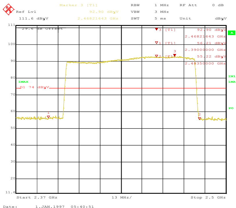
Figure 65: Radiated Emission at the Edge for 2DH1 Hopping – Horizontal (Pk)
