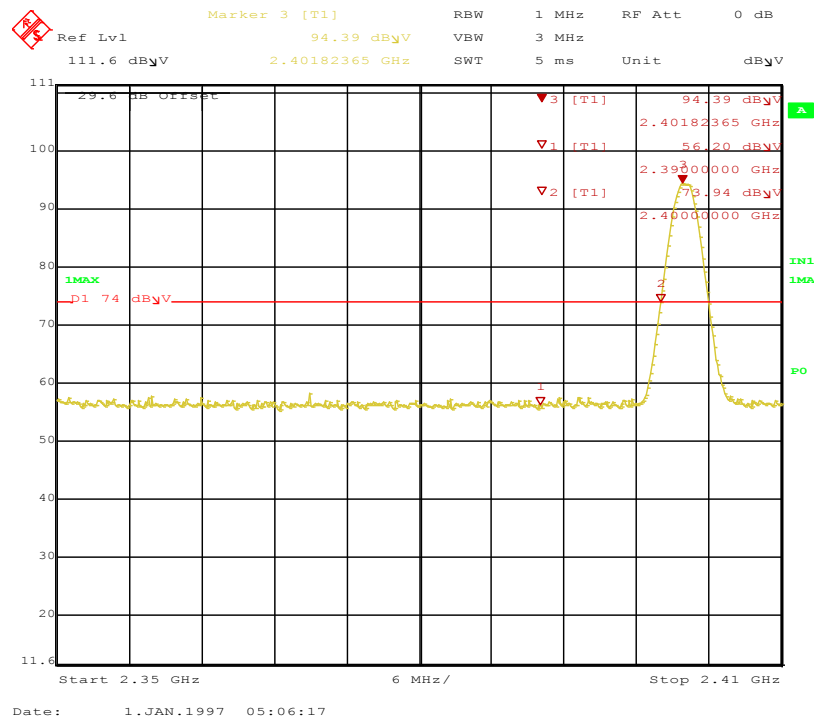
Figure 53: Radiated Emission at the Edge at 2DH1 - 2402 MHz – Vertical (Pk)
