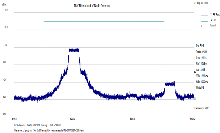
Figure 13: Measured Band-edge for 802.11a-6 Mbps at 5200 MHz
