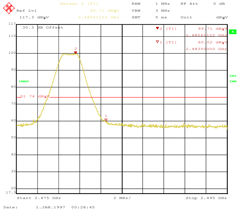
Figure 24: Band-edge-2480 MHz-V-Pk
