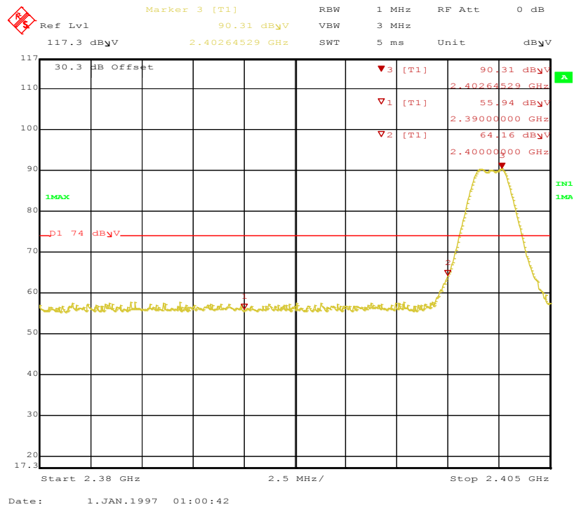
Figure 22: Band-edge-2402 MHz-H-Pk
