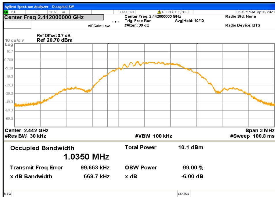
Figure 9: 99% Bandwidth-Headset -2442 MHz
