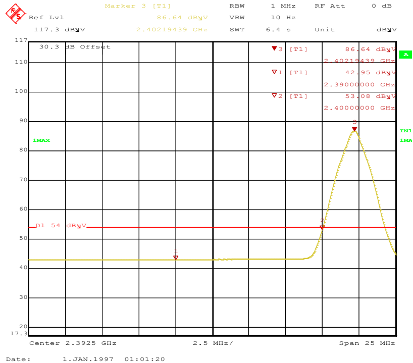
Figure 23: Band-edge-2402 MHz-H-Ave
