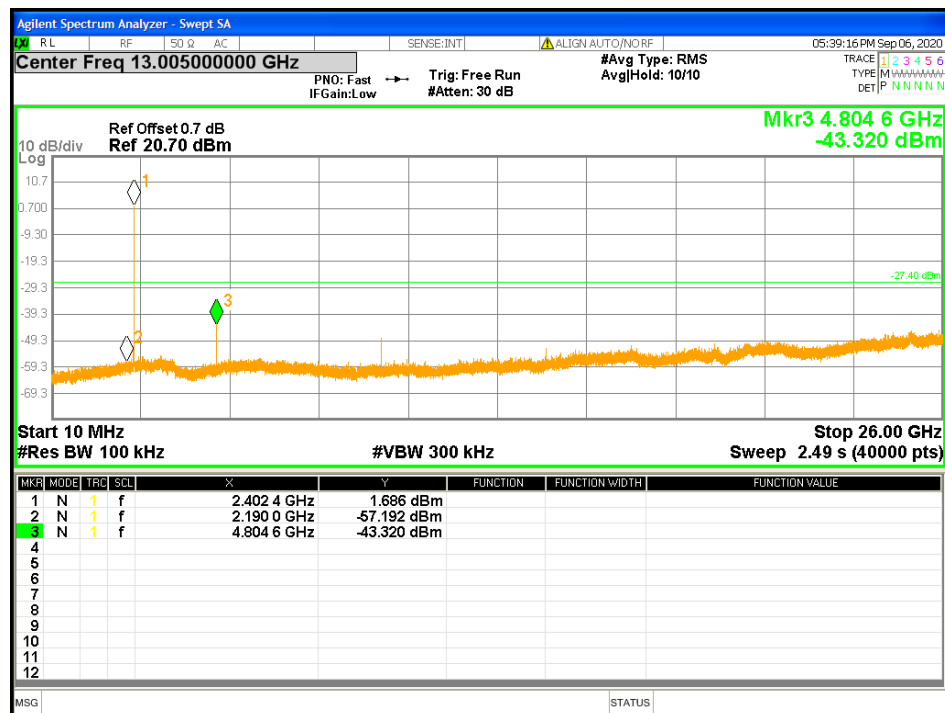
Figure 15: Out of band Emission at 2402 MHz
