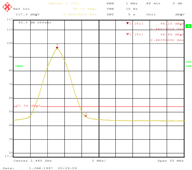
Figure 25: Band-edge-2480 MHz-V-Ave
