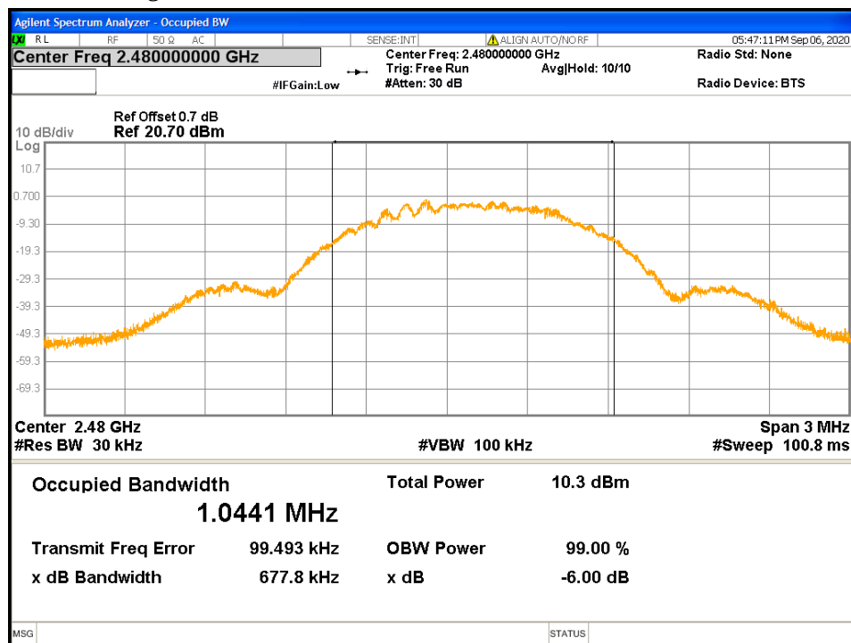
Figure 10: 99% Bandwidth-Headset -2480 MHz
