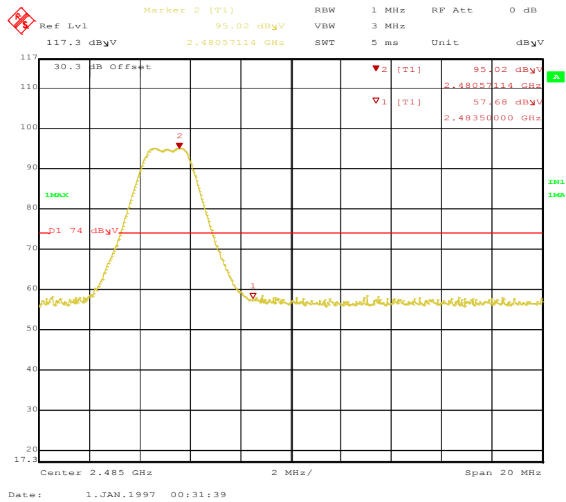
Figure 26: Band-edge-2480 MHz-H-Pk
