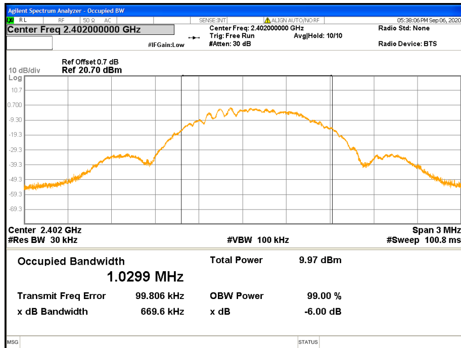
Figure 8: 99% Bandwidth-Headset -2402 MHz
