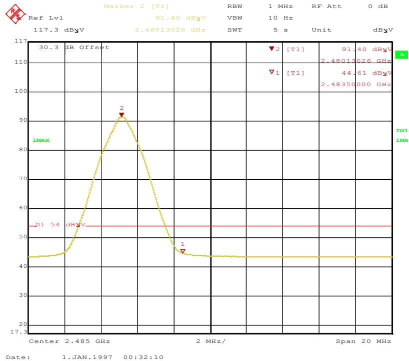
Figure 27: Band-edge-2480 MHz-H-Ave
