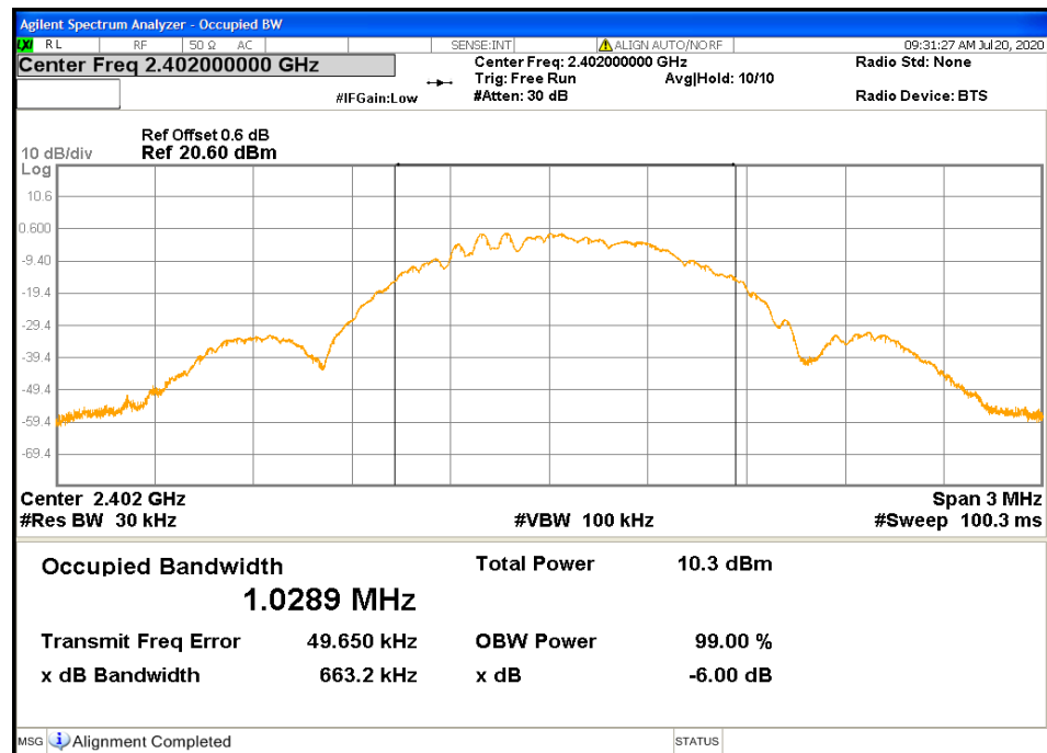
Figure 8: 99% Bandwidth-Headset -2402 MHz
