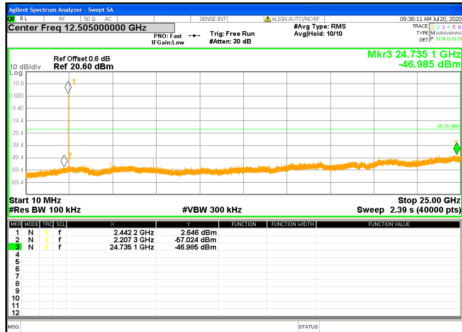
Figure 17: Out of band Emission at 2442 MHz-Headset
