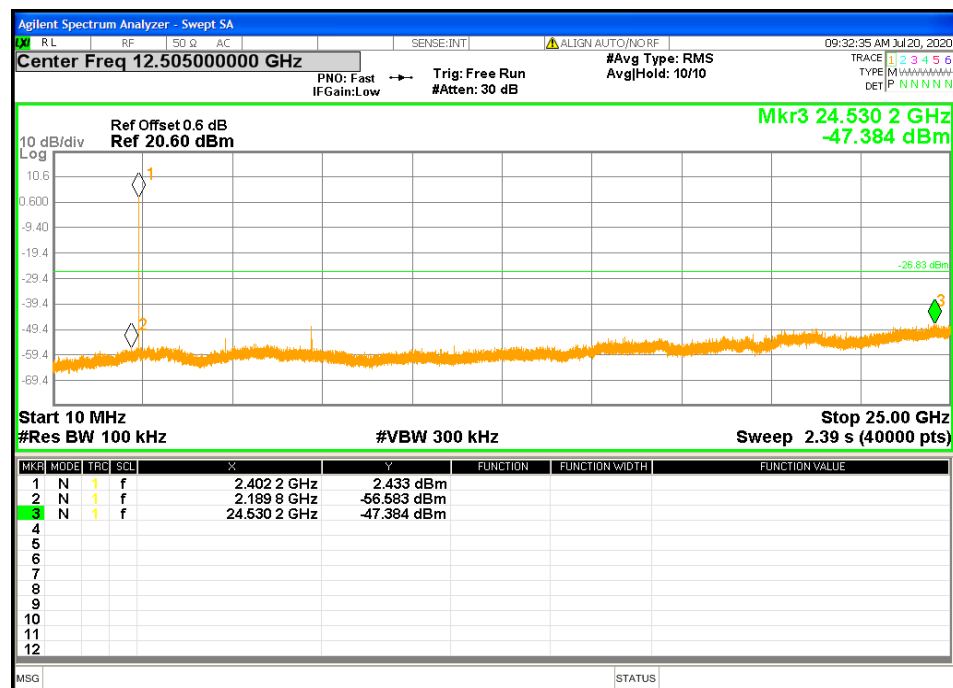
Figure 15: Out of band Emission at 2402 MHz-Headset
