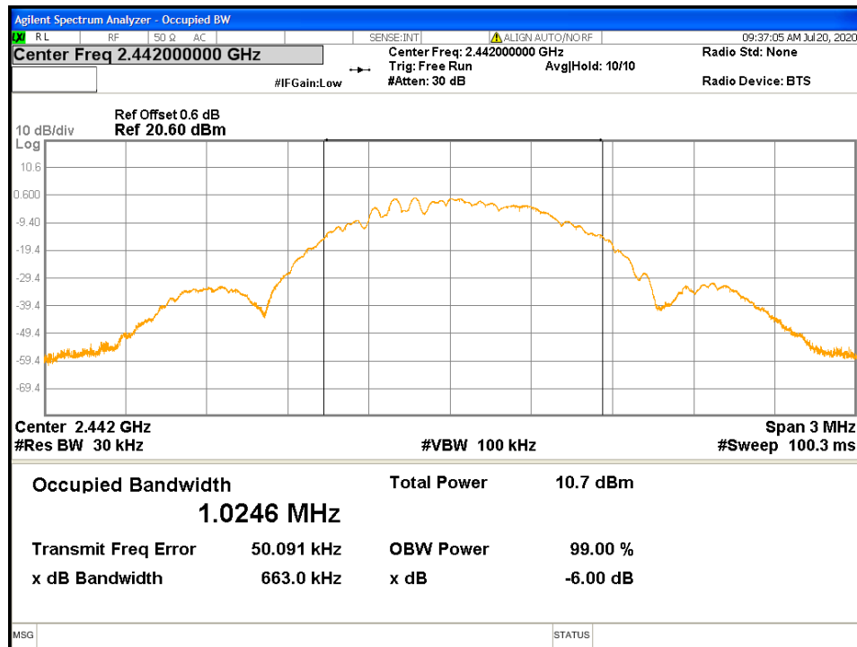
Figure 9: 99% Bandwidth-Headset -2442 MHz
