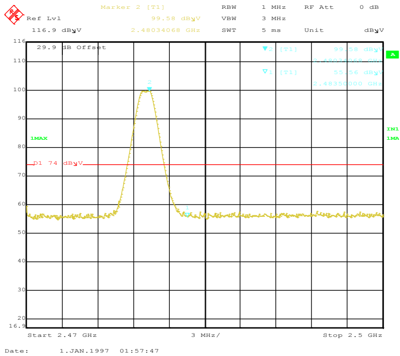
Figure 26: Band-edge-2480 MHz-H-Pk
