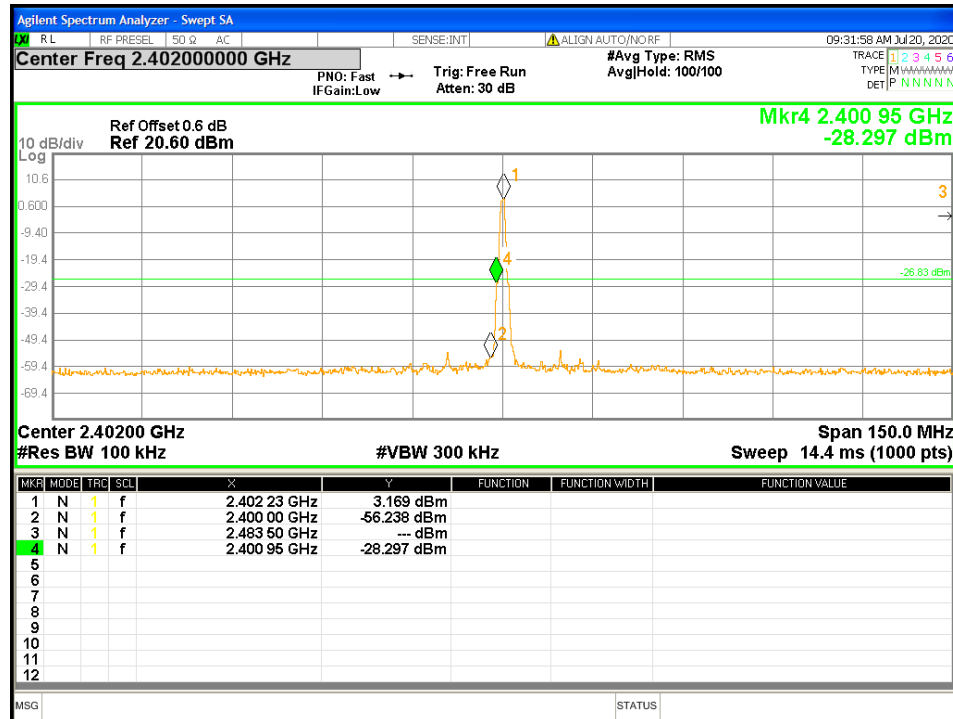
Figure 14: Conducted Band Edge at 2402 MHz-Headset
