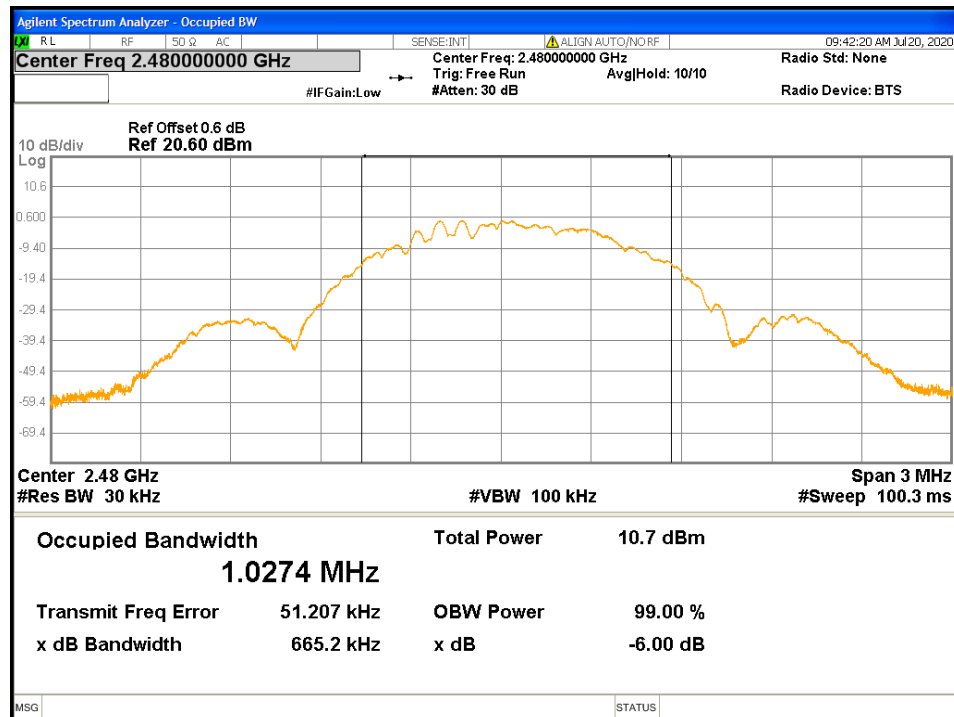
Figure 10: 99% Bandwidth-Headset -2480 MHz
