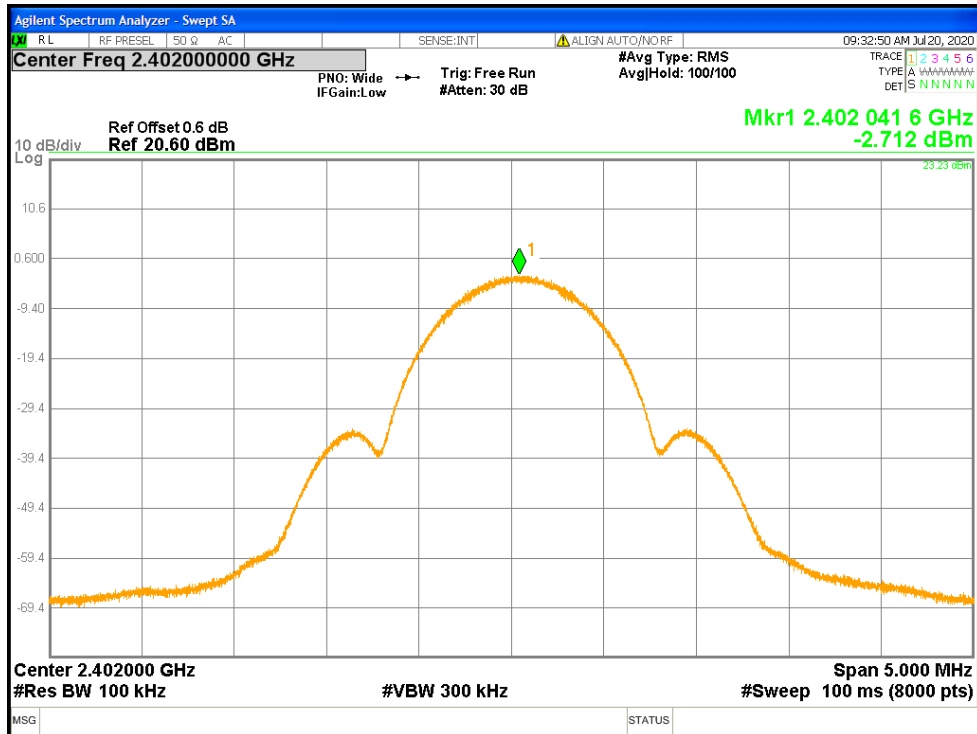
Figure 11: Maximum Power Spectral Density-2402 MHz-Headset
