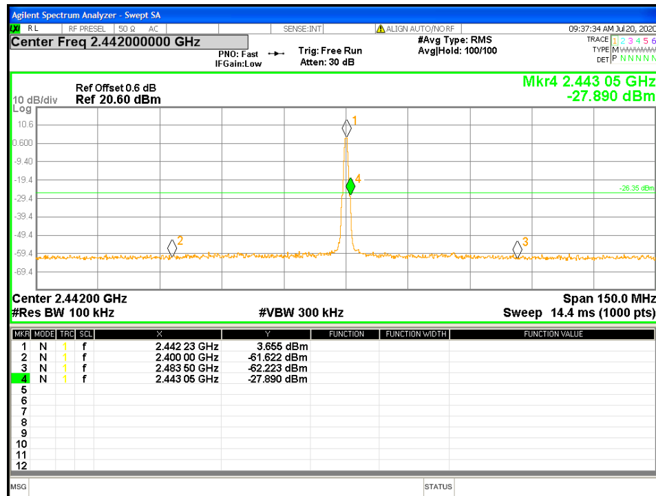
Figure 16: Conducted Band Edge at 2442 MHz-Headset
