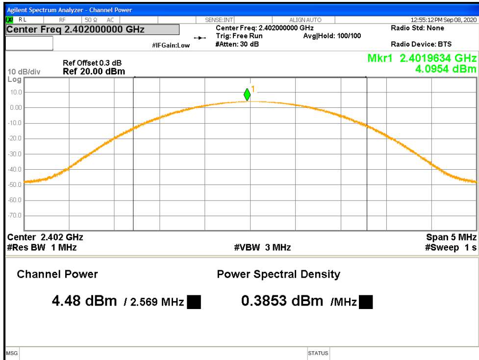
Figure 2: Maximum Conducted Output Power, 2402 MHz
