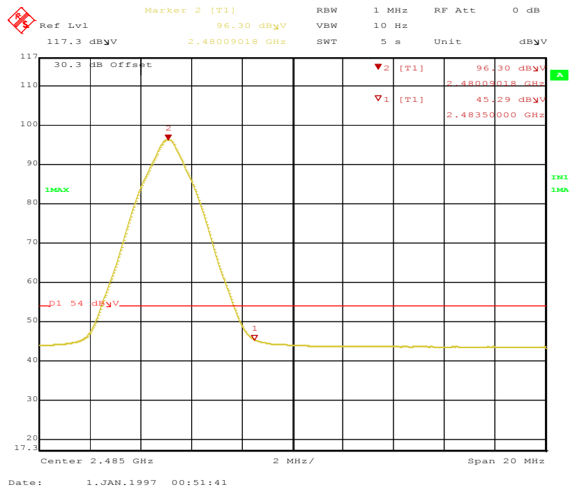
Figure 25: Band-edge-2480 MHz-V-Ave
