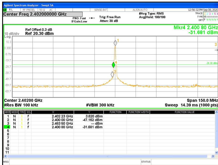
Figure 14: Conducted Band Edge at 2402 MHz
