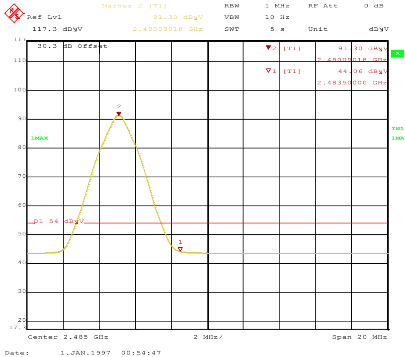
Figure 27: Band-edge-2480 MHz-H-Ave
