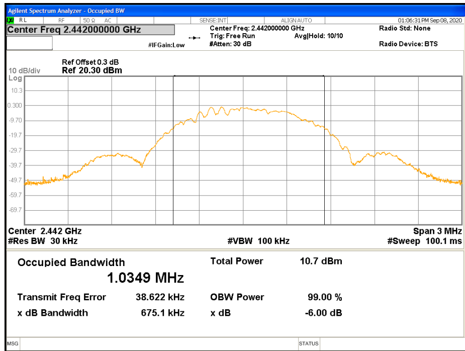
Figure 9: 99% Bandwidth-Transmitter -2442 MHz
