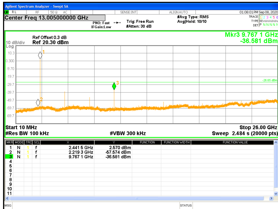
Figure 17: Out of band Emission at 2442 MHz
