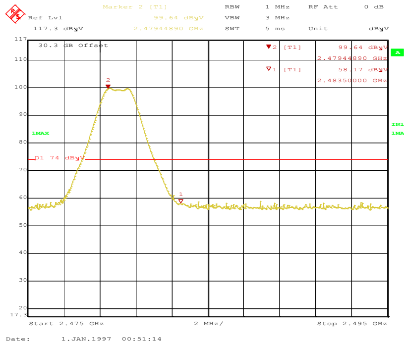
Figure 24: Band-edge-2480 MHz-V-Pk
