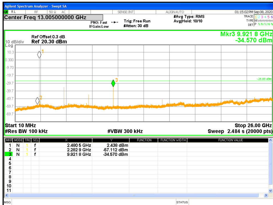
Figure 19: Out of band Emission at 2480 MHz
