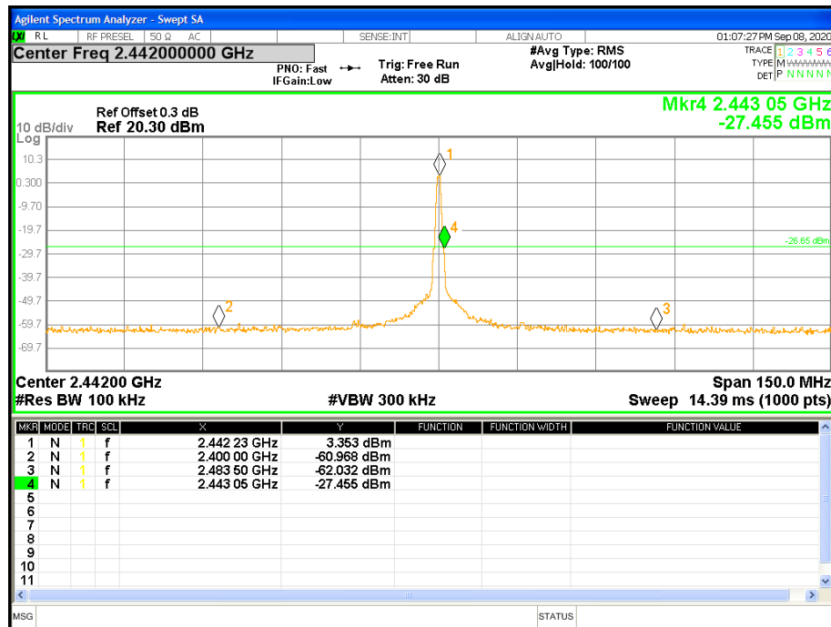
Figure 16: Conducted Band Edge at 2442 MHz
