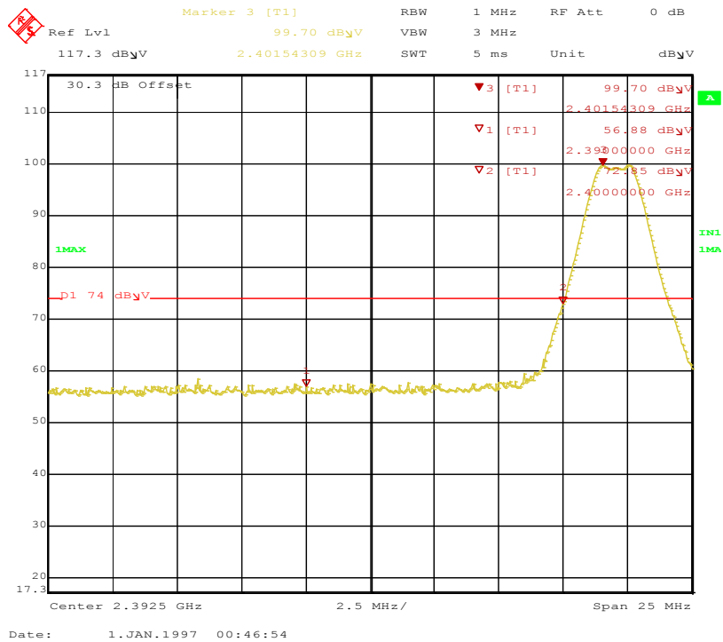
Figure 20: Band-edge-2402 MHz-V-Pk
