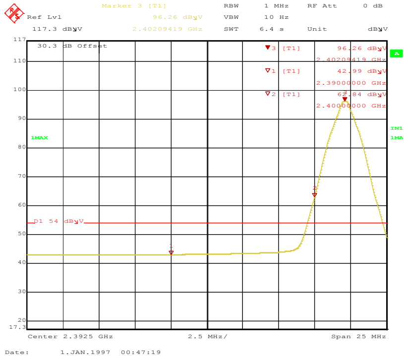
Figure 21: Band-edge-2402 MHz-V-Ave
