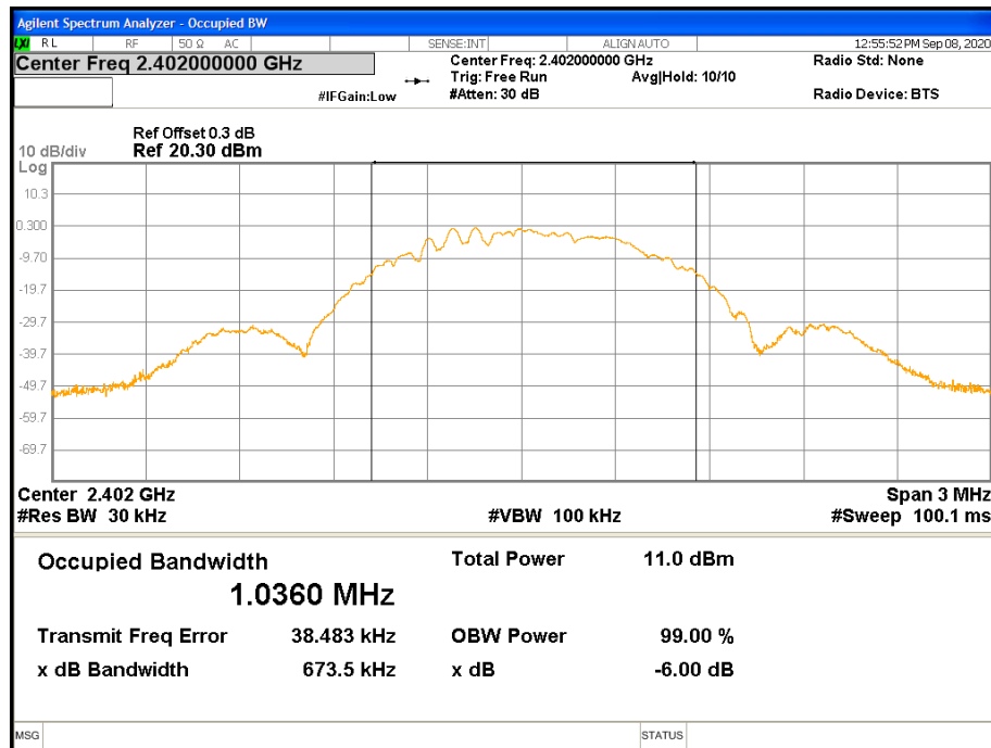
Figure 8: 99% Bandwidth-Transmitter -2402 MHz
