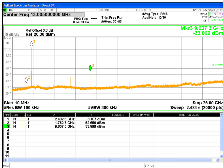
Figure 15: Out of band Emission at 2402 MHz
