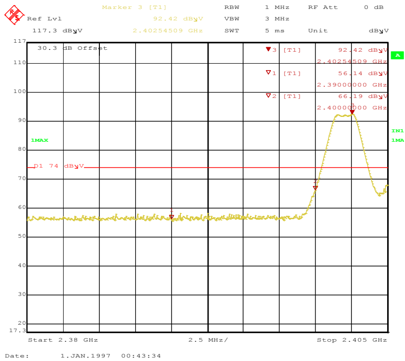
Figure 22: Band-edge-2402 MHz-H-Pk
