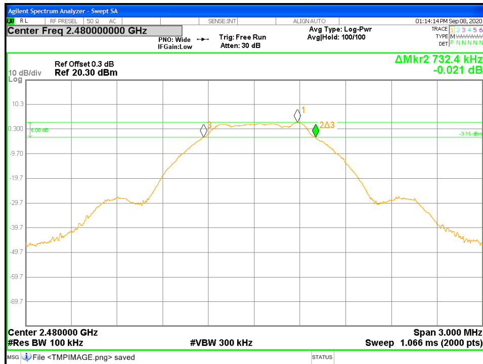
Figure 7: DTS Bandwidth-Transmitter -2480 MHz
