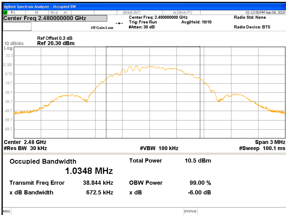
Figure 10: 99% Bandwidth-Transmitter -2480 MHz
