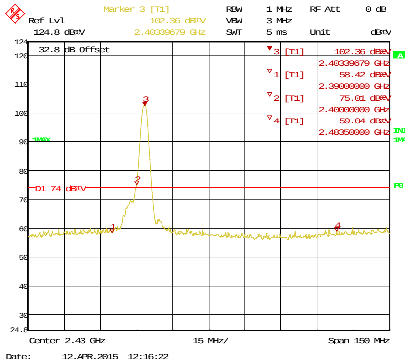
Figure 19: Bandedge-2403.35 MHz-H-Pk
