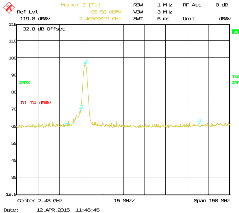
Figure 18: Bandedge-2403.35 MHz-V-pk
