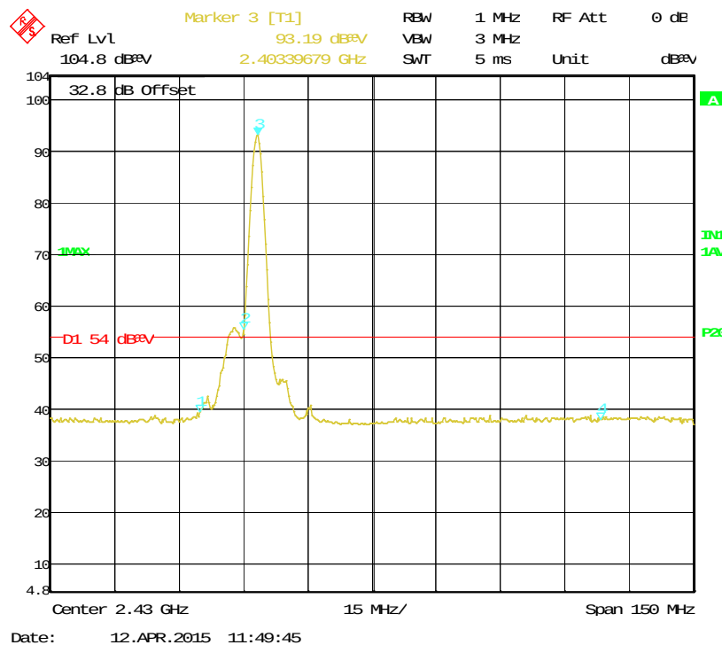
Figure 19: Bandedge-2403.35 MHz-V-Ave
