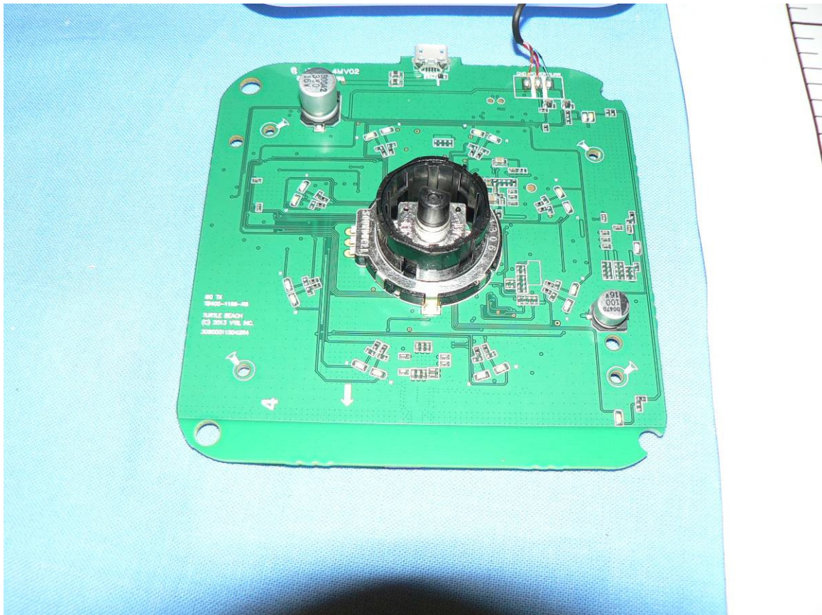
Main assy bottom view
