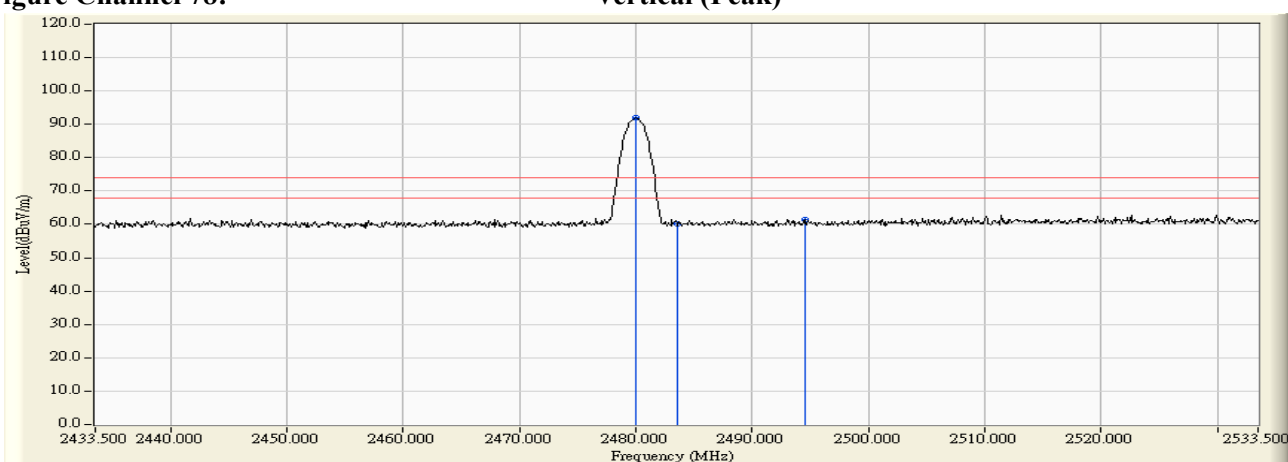
Figure Channel 78:
