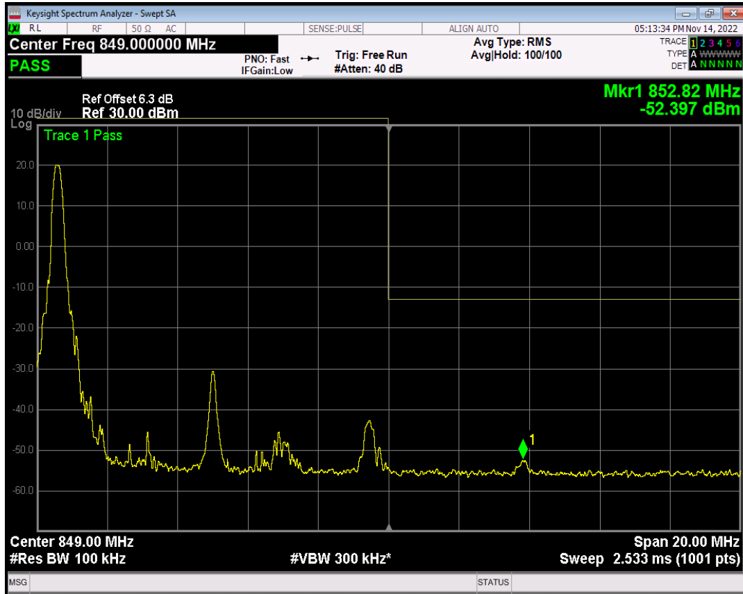
Band26(824-849) QAM16 BW=10MHz Channel=26990 RB Size=1 Position=#Max
